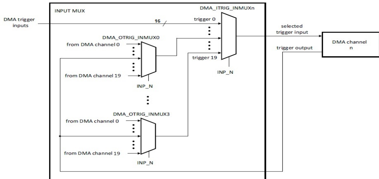
Fig 29. DMA trigger multiplexing
