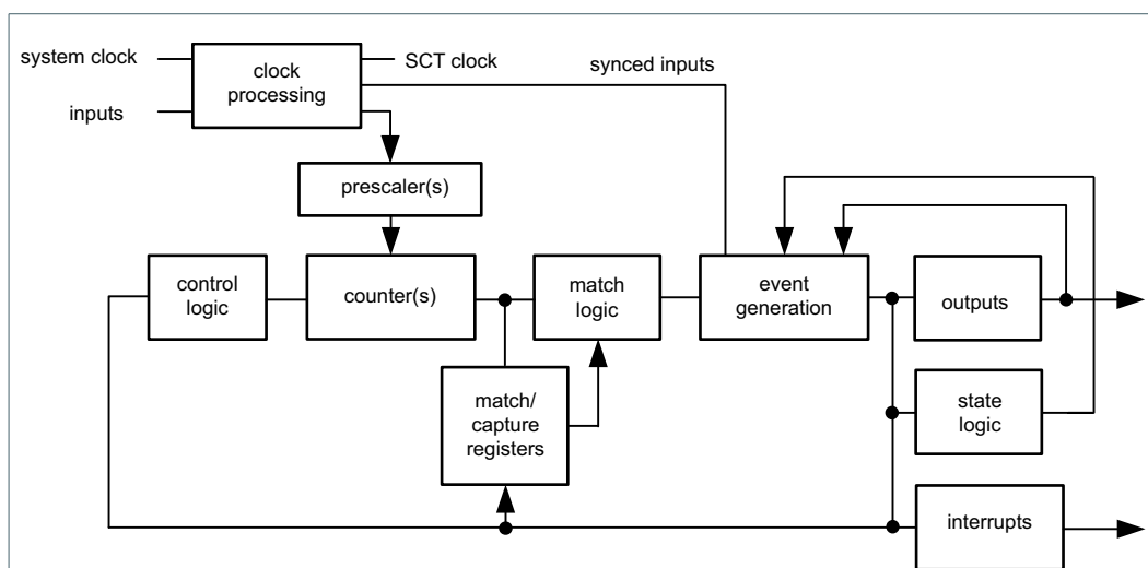
Fig 39. SCTimer/PWM block diagram
