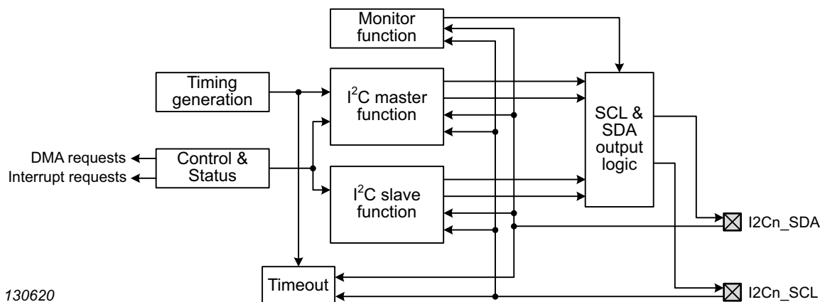
Fig 73. I 2 C block diagram
