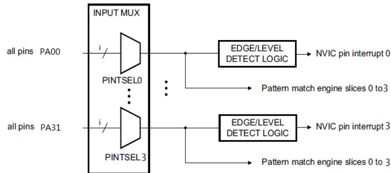
Fig 28. Pin interrupt multiplexing
