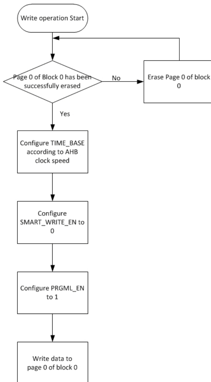
Fig 80. Flash write example 1
