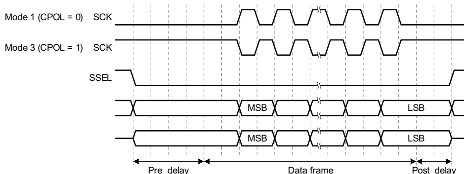
Fig 69. Pre_delay and Post_delay
