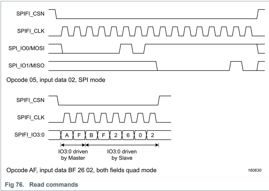
Figure 76 shows a command that reads 1 byte from the slave in SPI mode and a command that reads 3 bytes from the slave with the opcode and input data fields both in quad mode.
