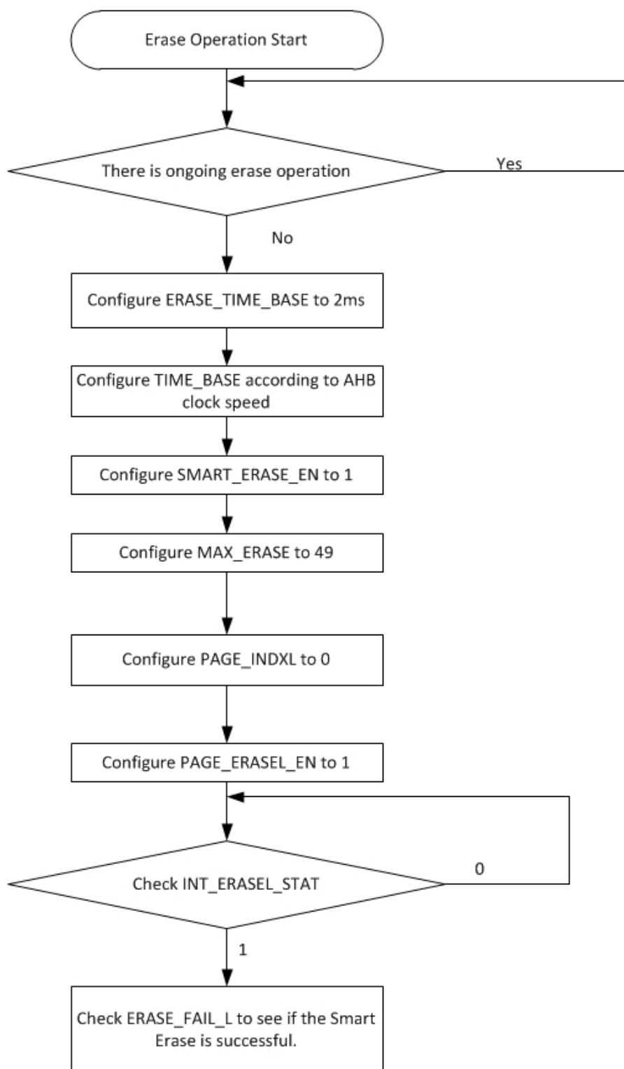
Fig 85. Flash erase example 2
