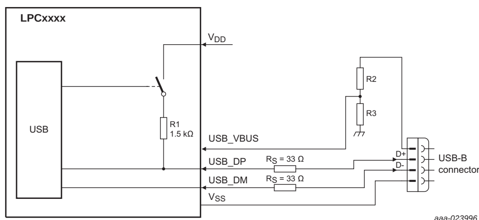
Fig 45. USB interface on a self-powered device where USB_VBUS = 5 V
