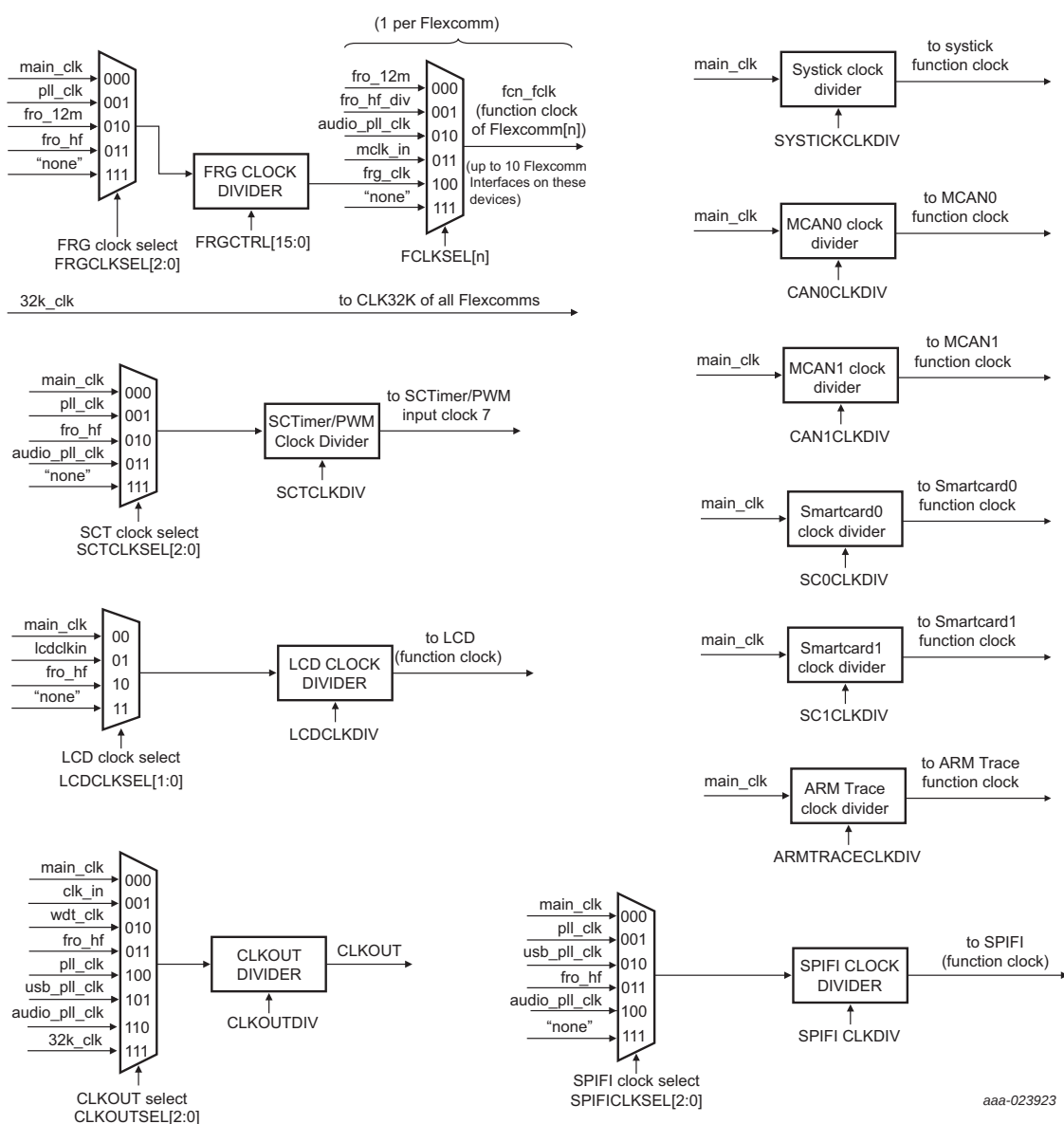
Fig 9. LPC5460x clock generation (continued)
