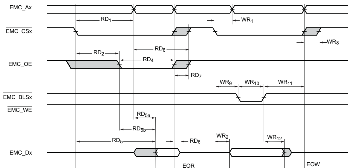
Fig 21. External static memory read/write access (PB = 0)
