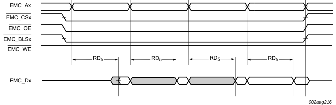
Fig 23. External static memory burst read cycle
