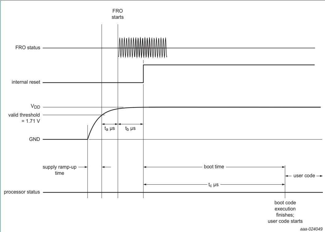
Fig 40. Start-up timing
