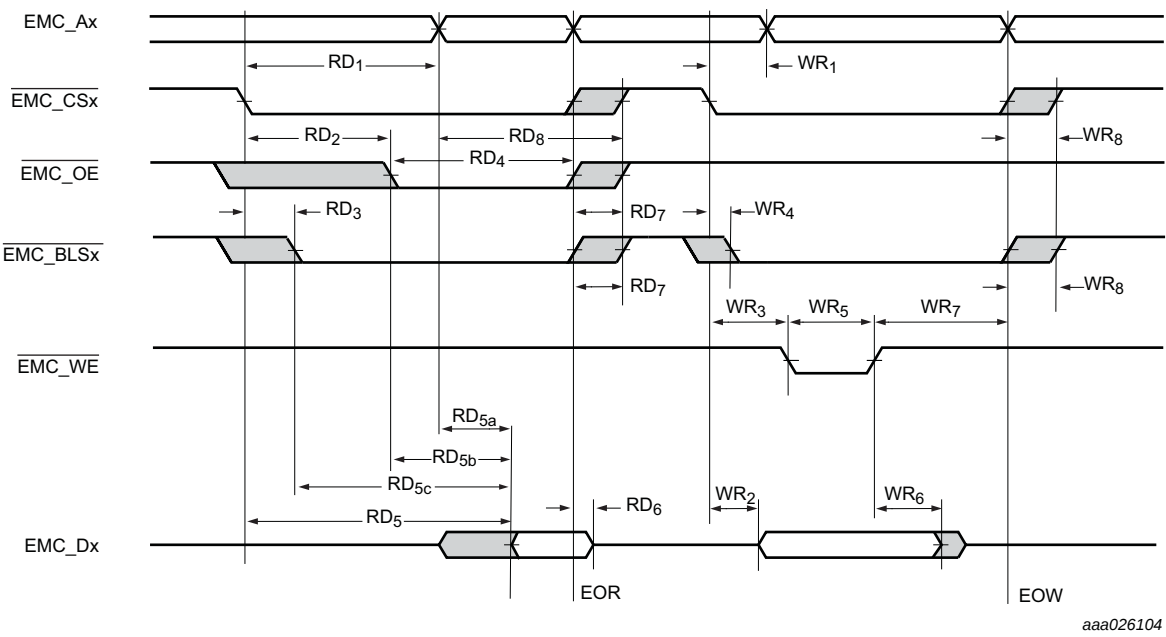
Fig 22. External static memory read/write access (PB =1)
