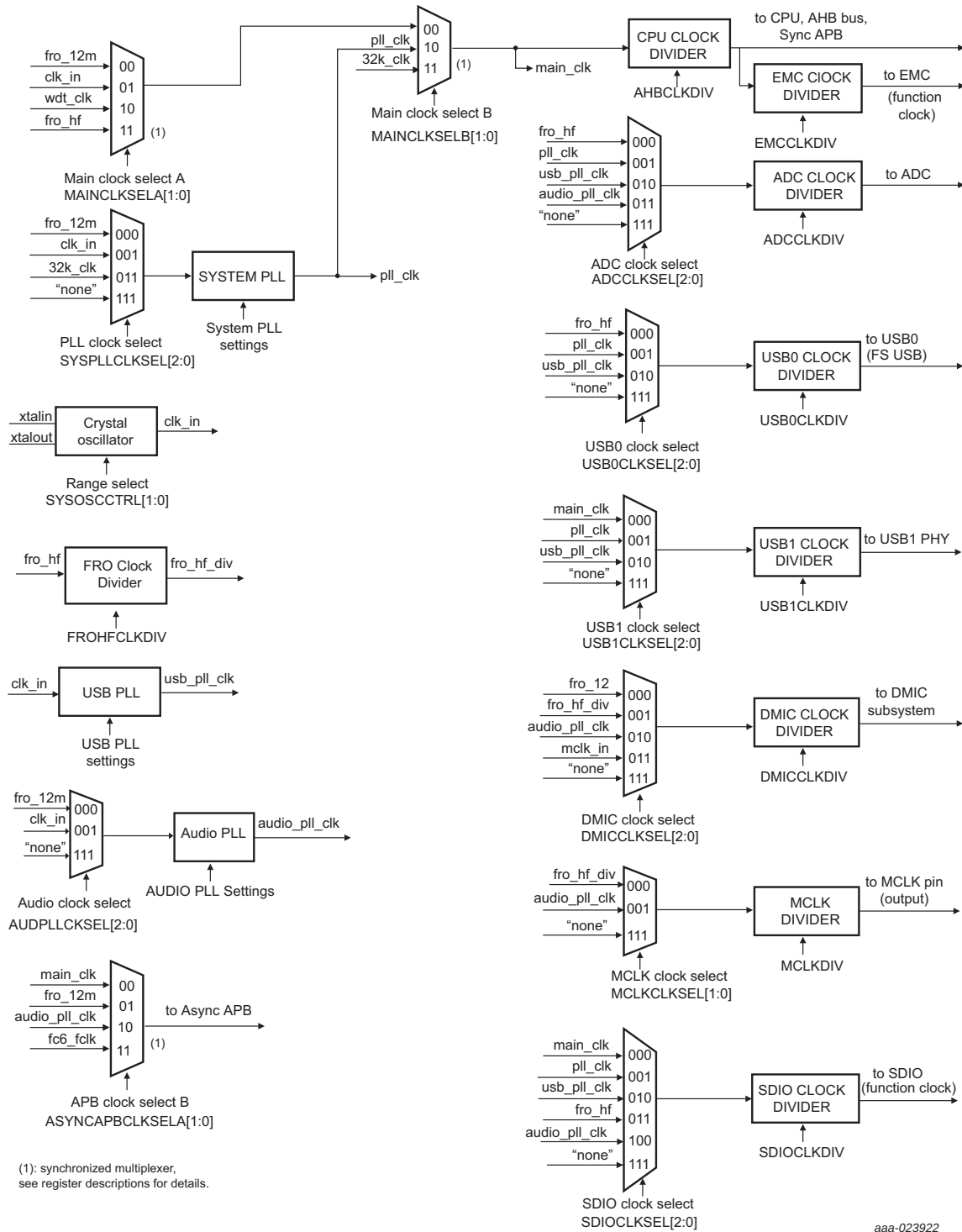
Fig 8. LPC5460x clock generation
