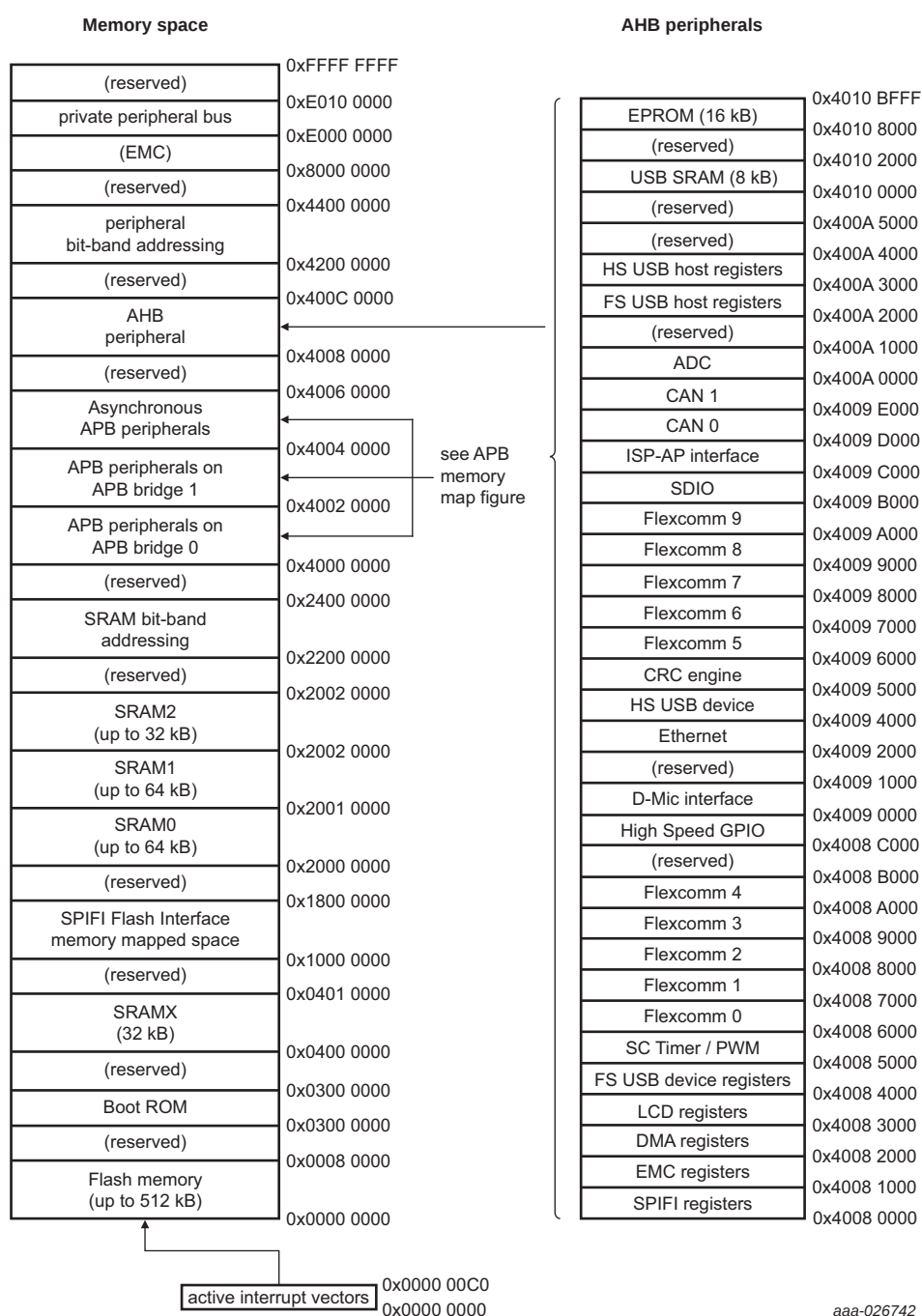
Fig 6. LPC5460x Memory mapping
