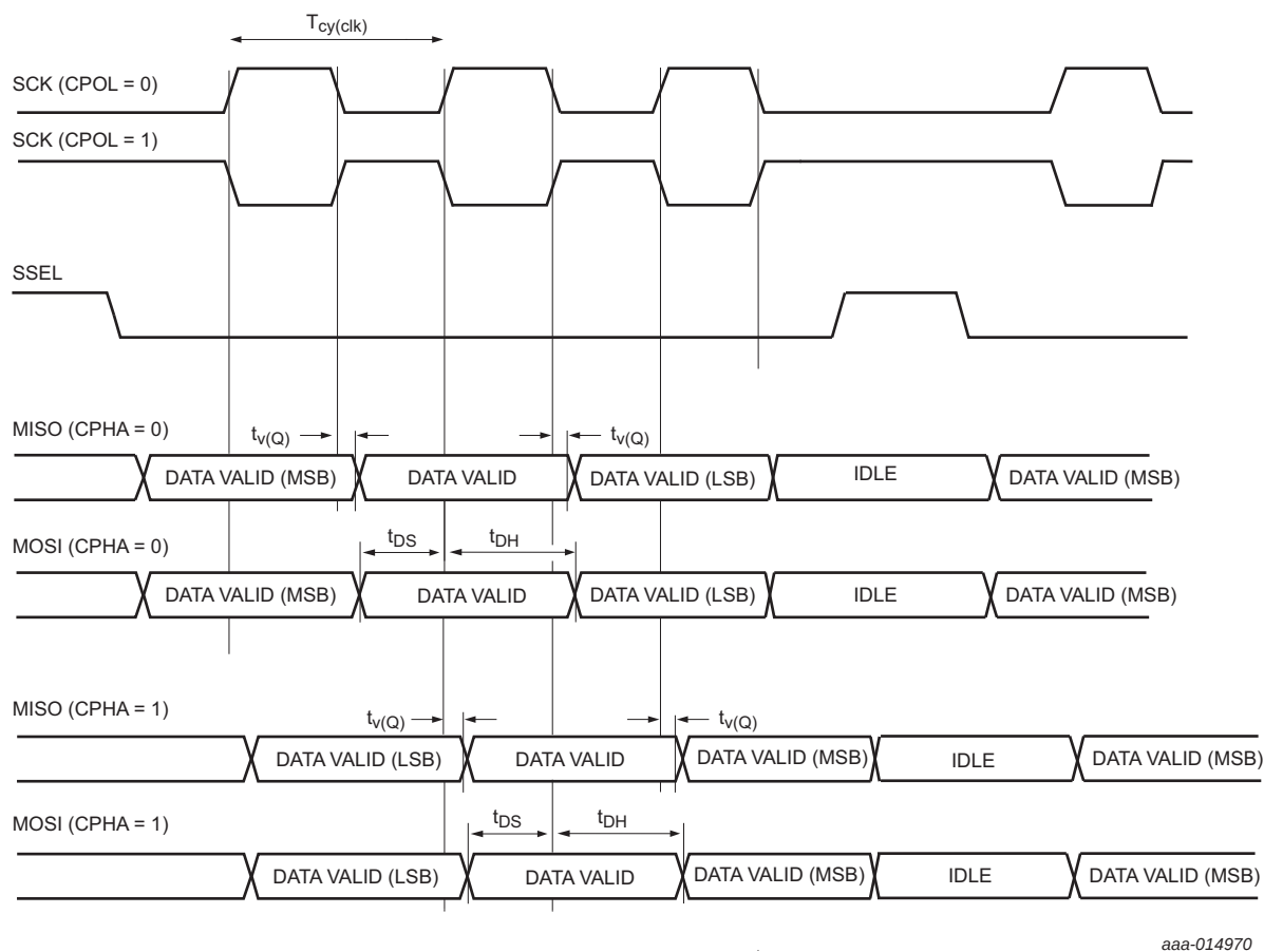
Fig 29. SPI slave timing
