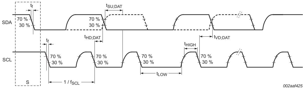
Fig 25. I 2 C-bus pins clock timing
