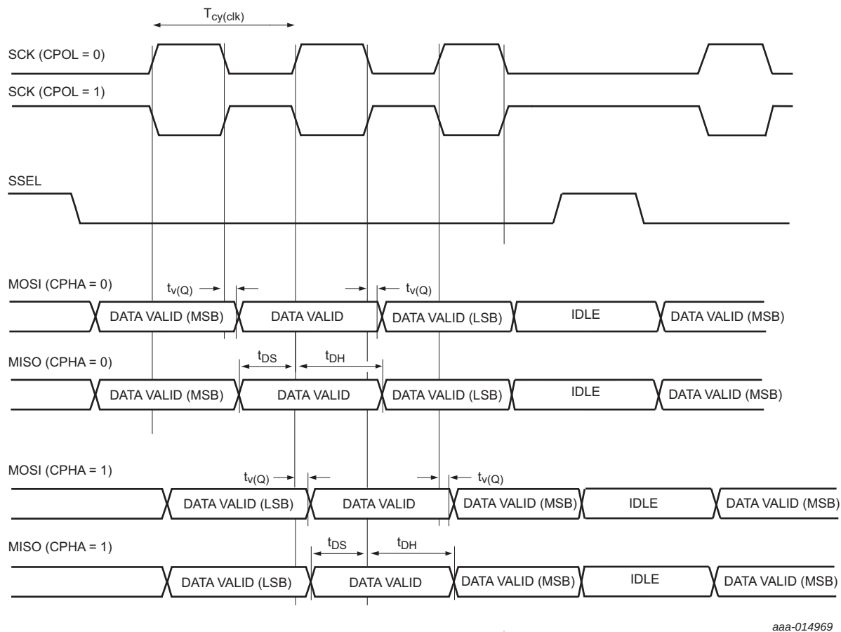
Fig 28. SPI master timing
