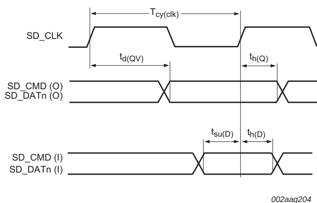
Fig 36. SD/MMC and SDIO timing
