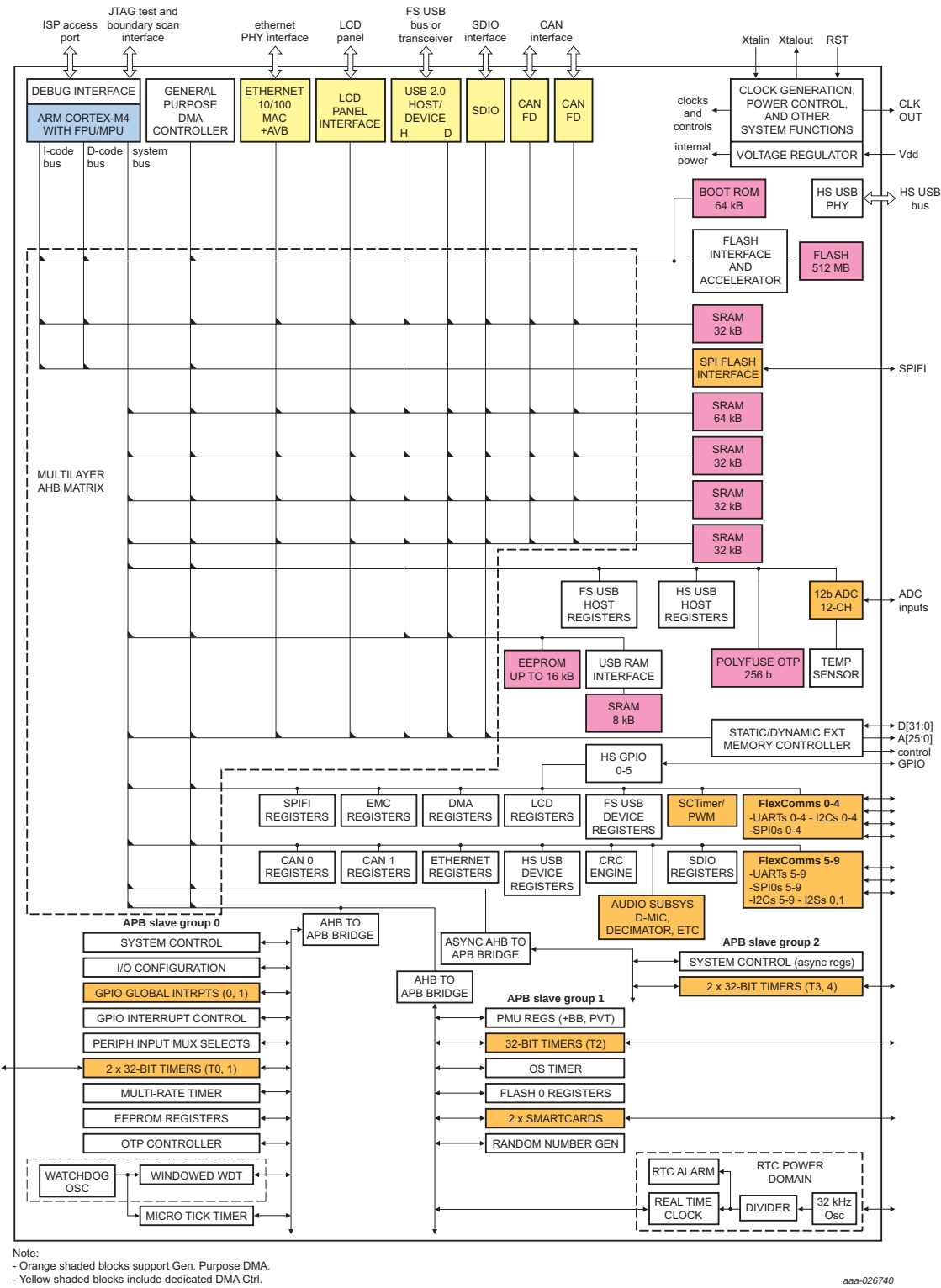
Fig 3. LPC5460x Block diagram
