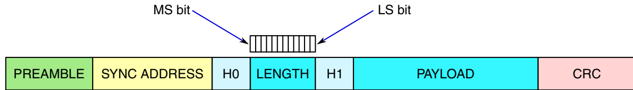
Figure 45-106. LENGTH Bit Ordering (MSB First)
