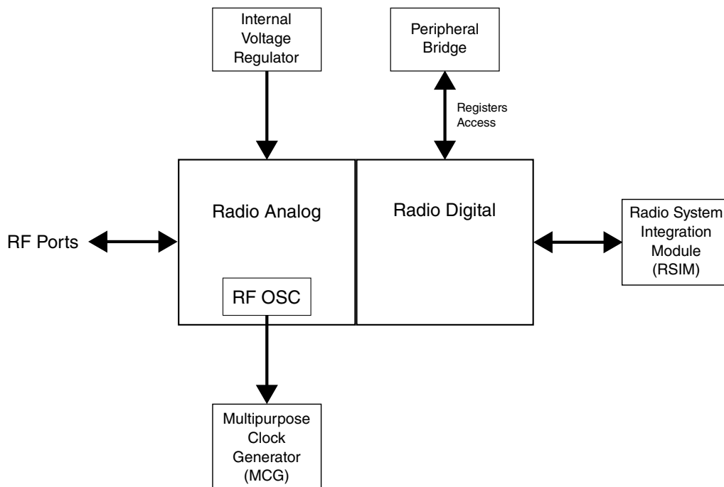
Figure 4-34. Radio configuration
