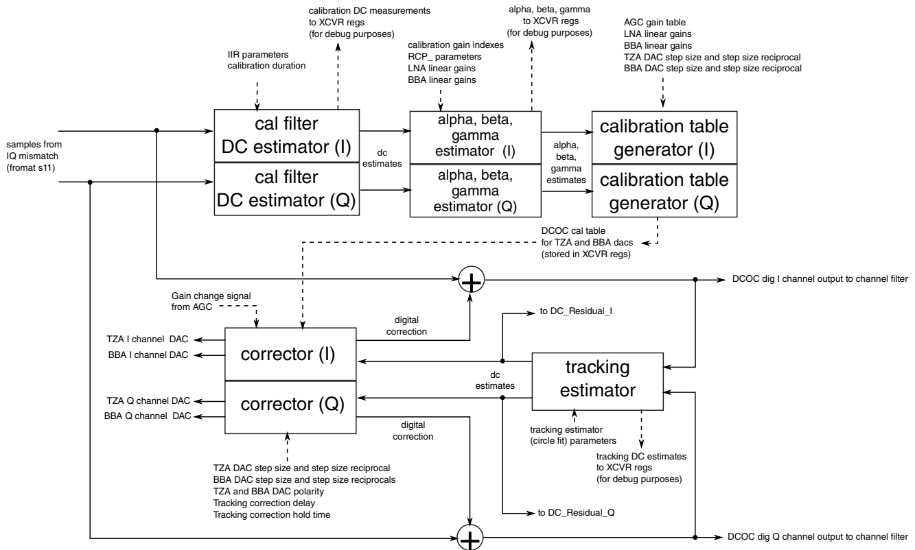
Figure 45-38. RX_DIG DCOC Block Diagram
