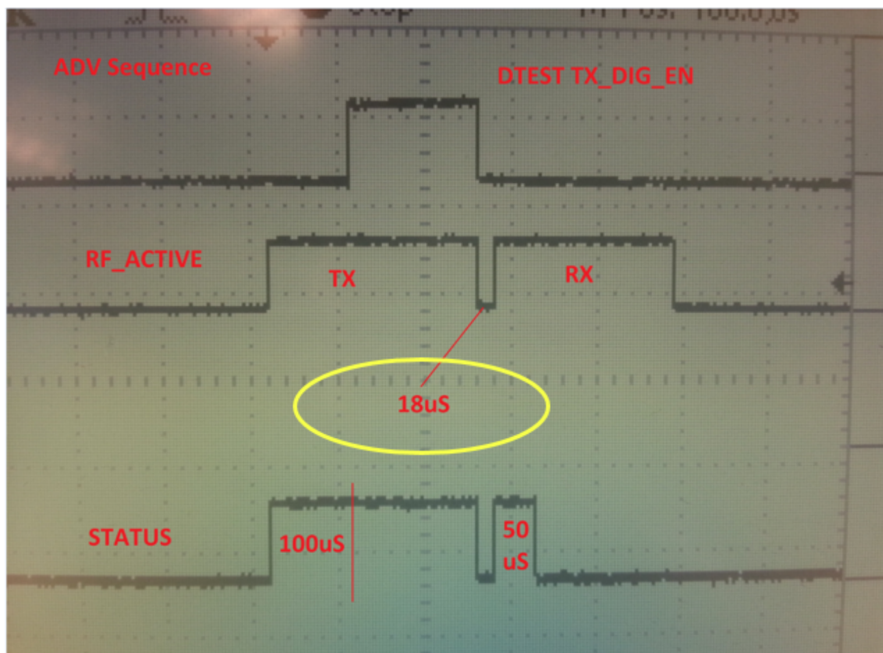
Figure 45-78. ACTUAL RF_ACTIVE TIMING (UNCOMPENSATED)
