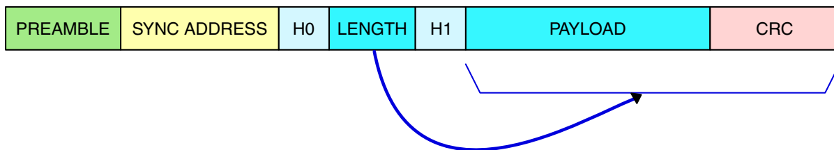
Figure 45-103. LENGTH Field Interpretation with No LENGTH_ADJ
