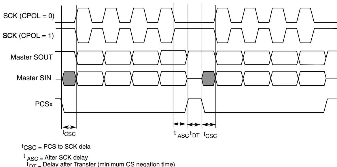
Figure 38-13. Example of non-continuous format (CPHA=1, CONT=0)
