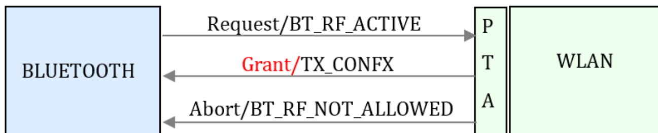
Figure 45-75. 3-WIRE THIRD PARTY INTERFACE
