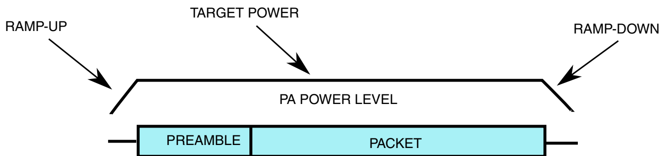
Figure 45-59. PA Target Power
