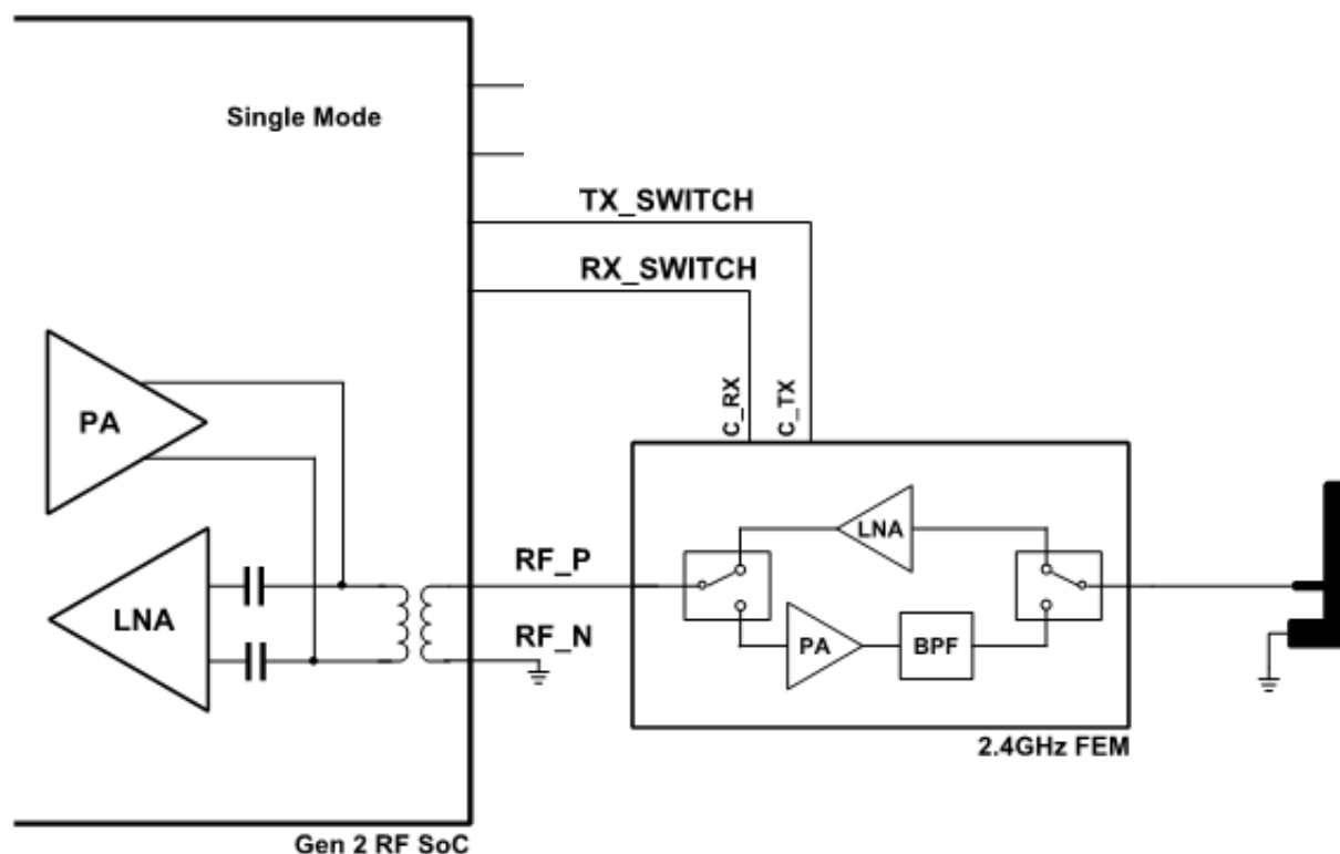
Figure 45-71. FEM Interface Single Antenna Configuration
