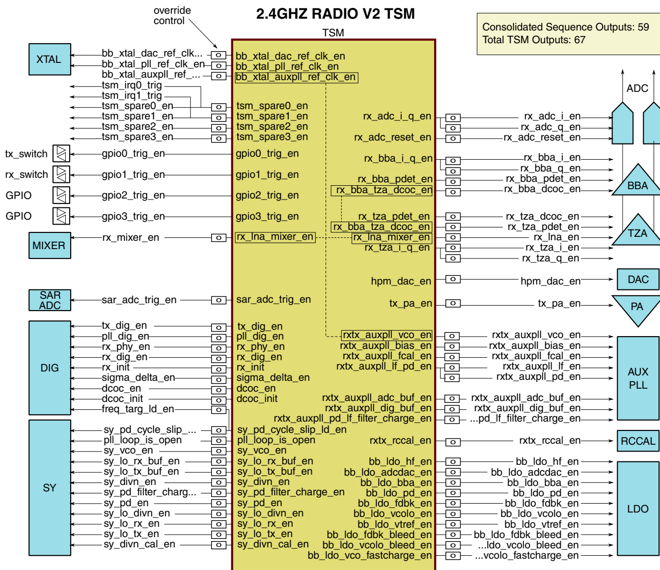
Figure 45-55. 2.4GHZ RADIO TSM
