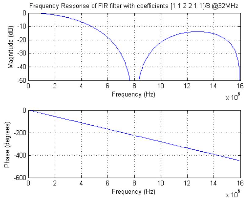
Figure 45-9. Frequency response of the 6-Tap FIR Transmit Image Suppression filter
