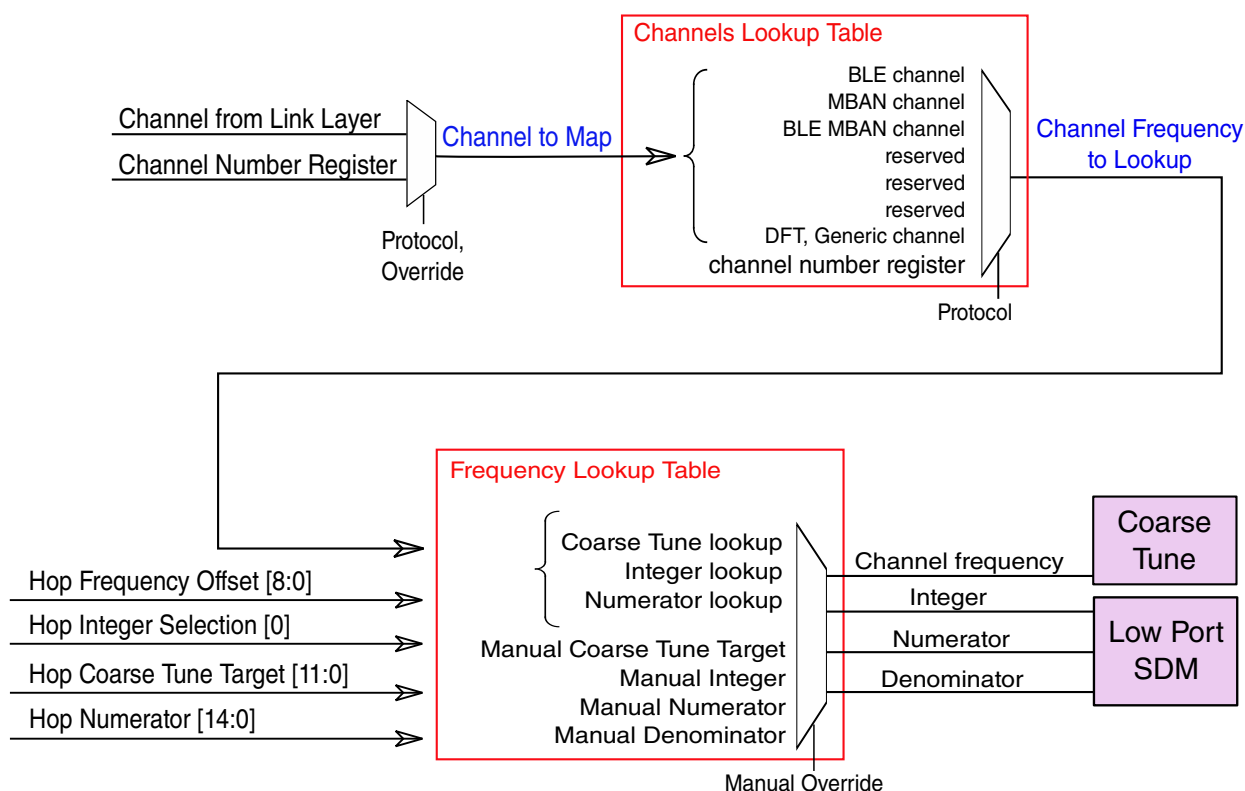
Figure 45-15. Radio Frequency Selection
