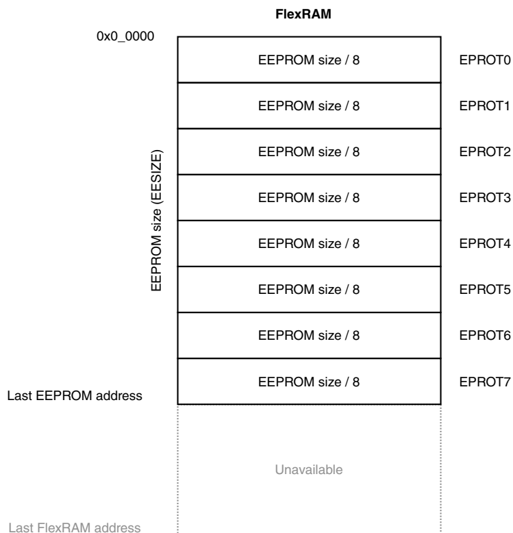
Figure 29-5. EEPROM protection
