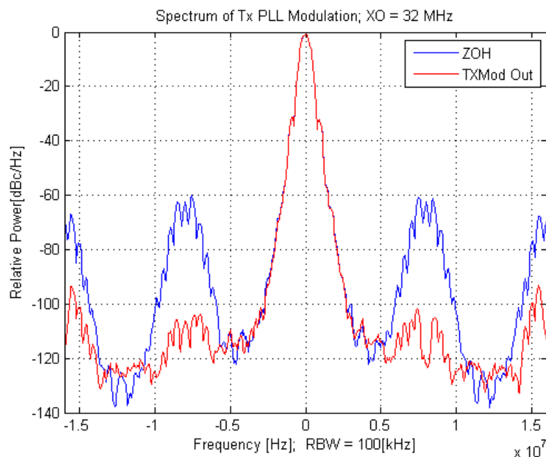
Figure 45-11. Comparison of Transmit Modulation Images at the PLL Output for BLE (1 Mbps GMSK)
