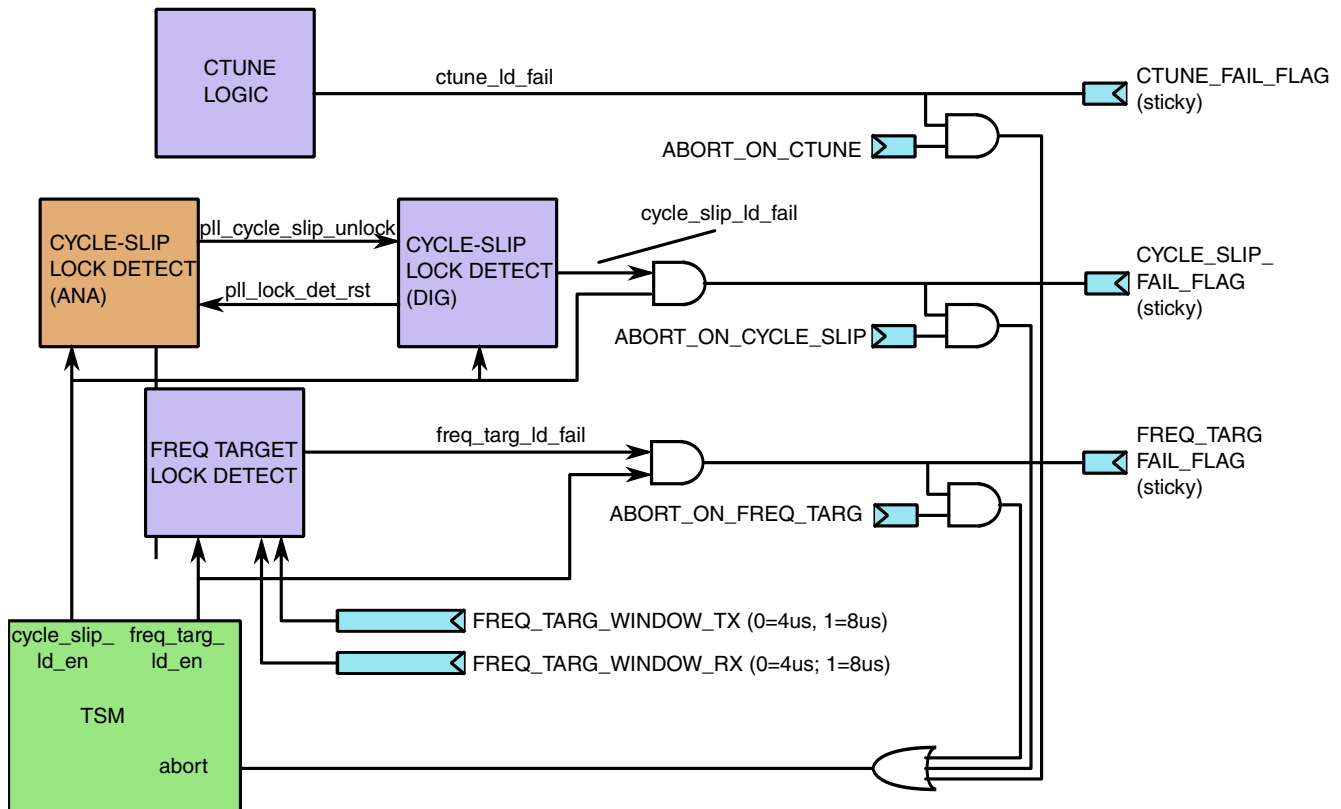
Figure 45-57. PLL UNLOCK MONITORING AND ABORT LOGIC
