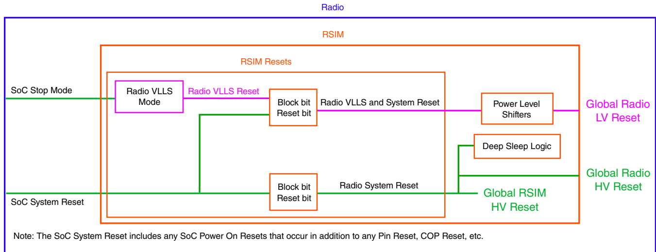
Figure 45-5. Radio Reset Tree
