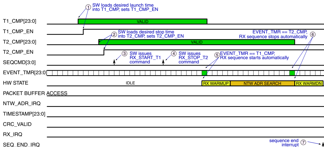
Figure 45-133. GENERIC FSK RX SEQUENCE: SLAVE CHANNEL SEARCH, LAUNCH VIA T1, STOP VIA T2
