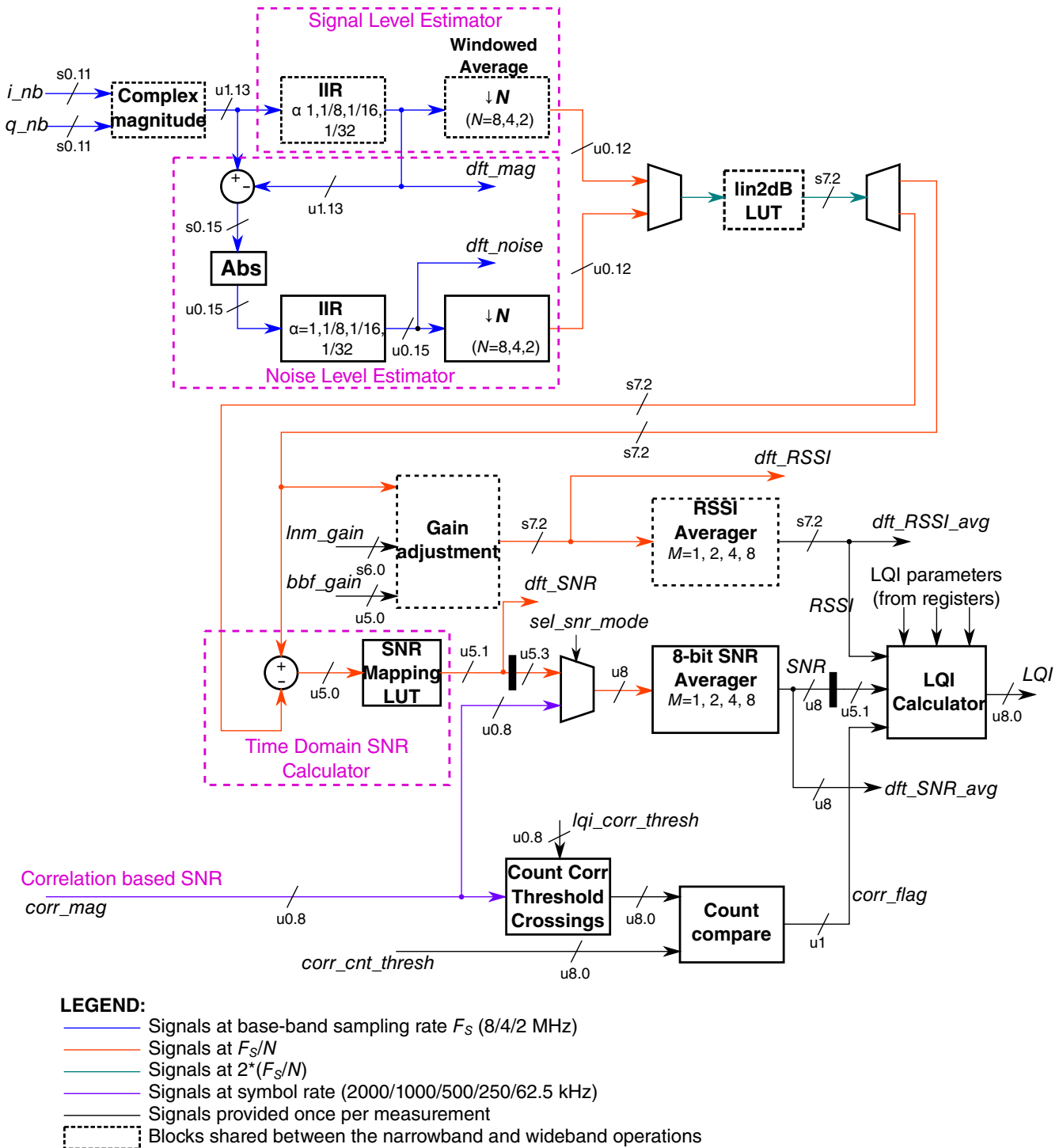
Figure 45-34. Block diagram instantiated for narrowband mode
