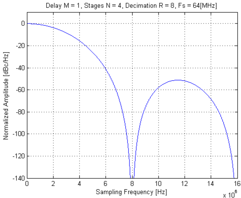
Figure 45-28. 4th order CIC (OSR=8) Decimation Filter Frequency Response
