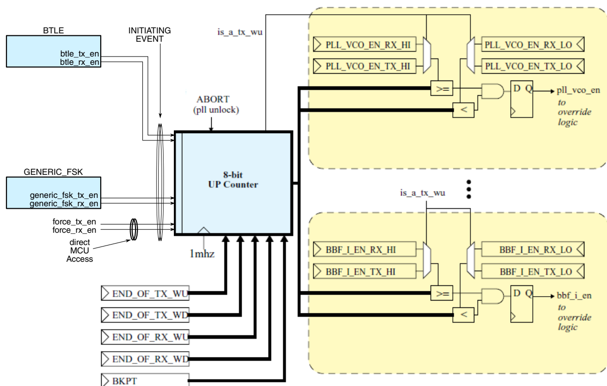
Figure 45-56. 2.4GHZ RADIO TSM BLOCK DIAGRAM
