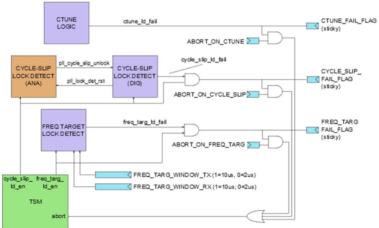
Figure 45-22. PLL Lock Detect Block Diagram
