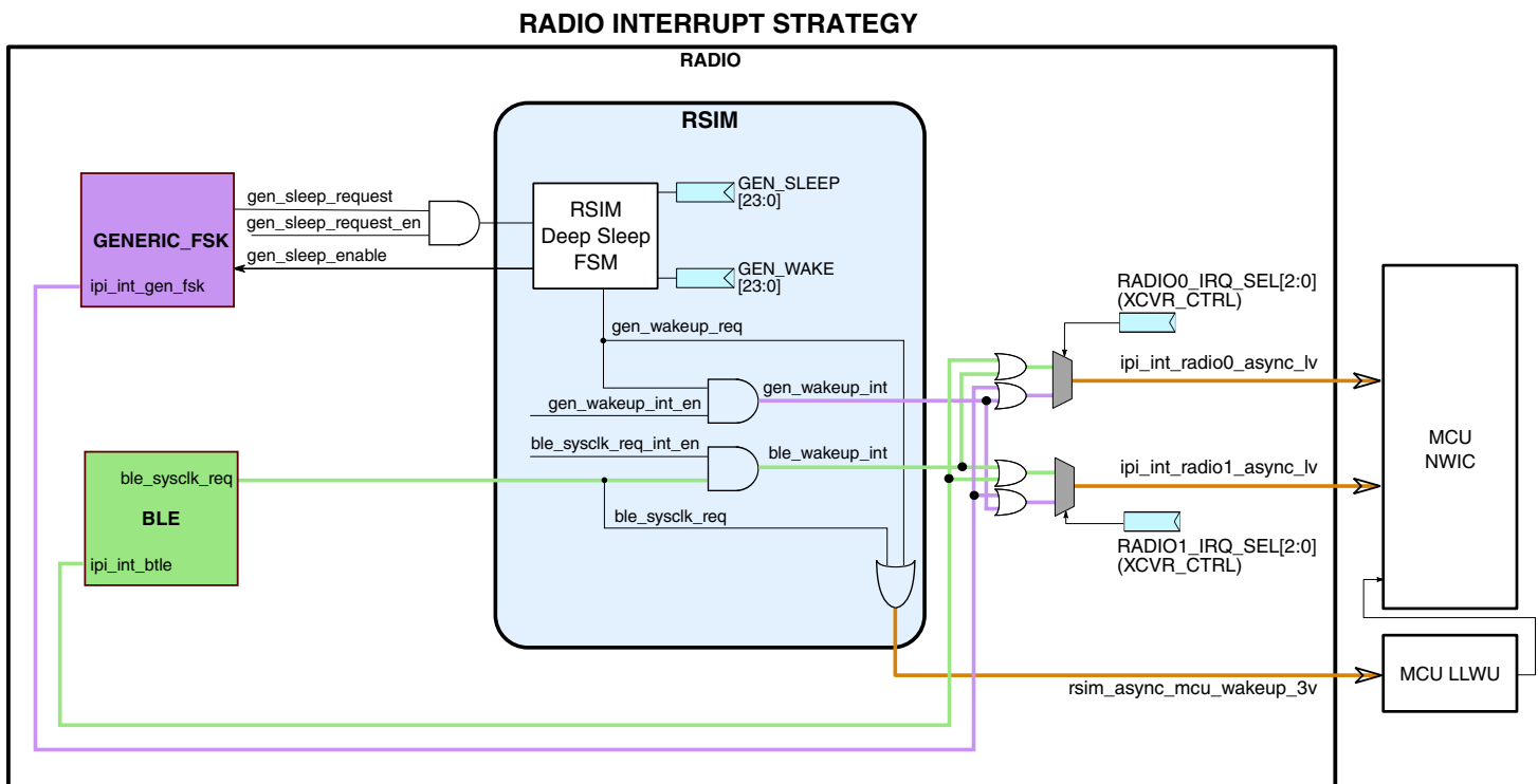
Figure 45-4. Radio Interrupts
