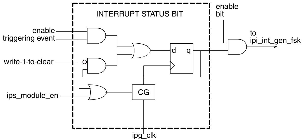
Figure 45-127. Interrupt Status Bit
