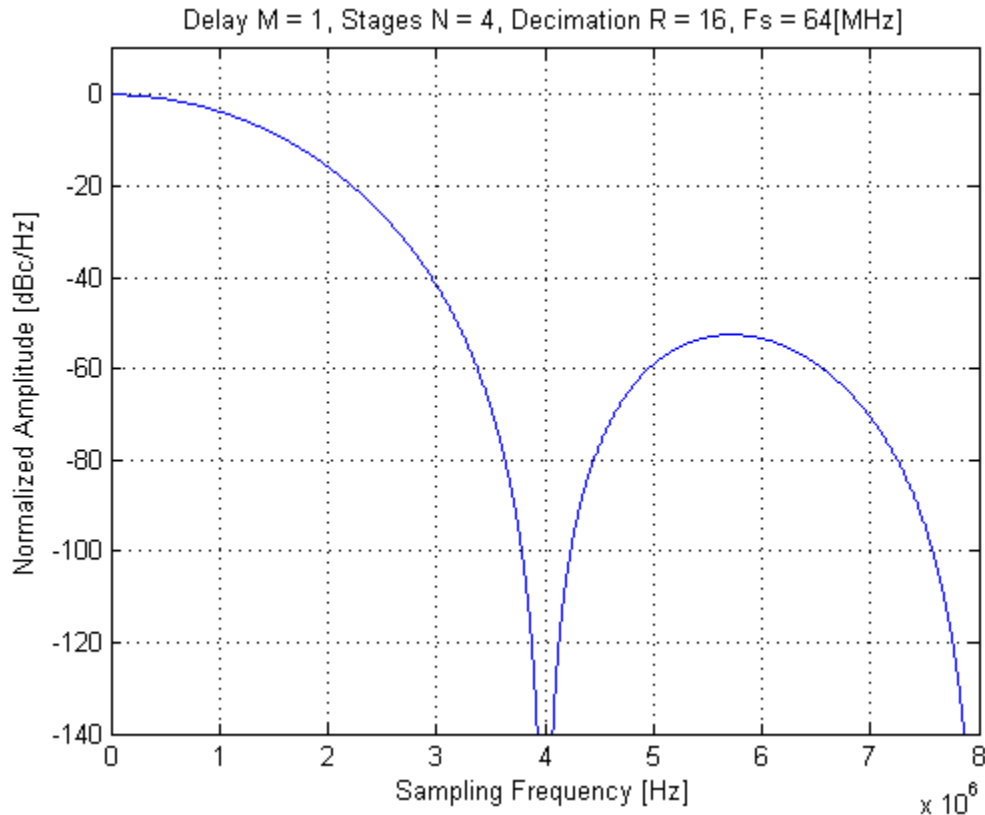
Figure 45-29. 4th order CIC (OSR=16) Decimation Filter Frequency Response
