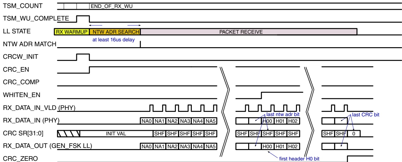
Figure 45-115. BIT STREAM PROCESSING CRC AND WHITENING RX TIMING
