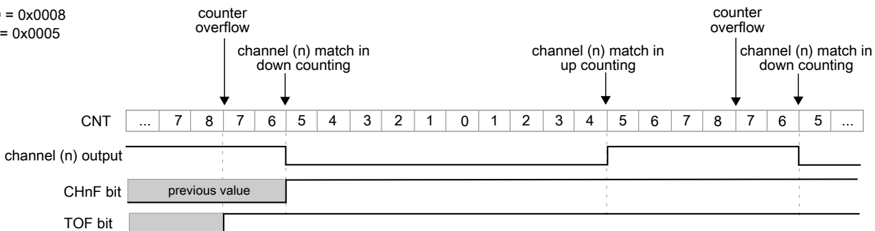
Figure 33-14. CPWM signal with ELSnB:ELSnA = X:1
