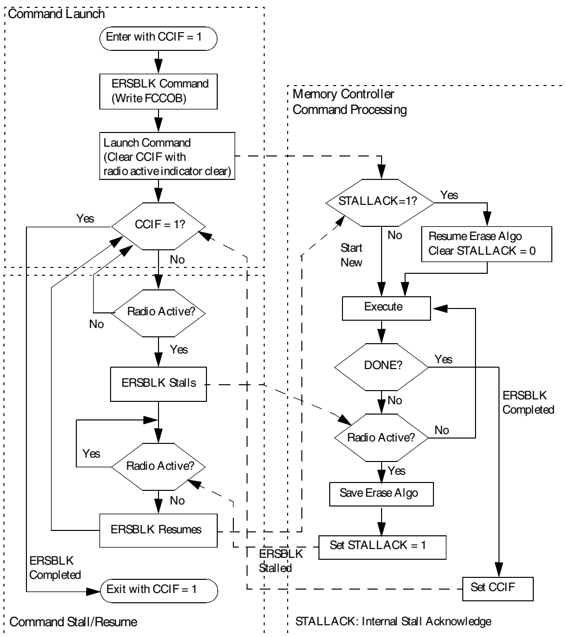
Figure 29-12. Radio Active Impact on Erase Flash Block Operation
