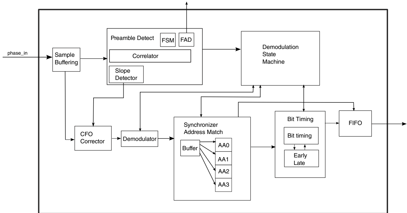
Figure 45-94. PHY Block diagram
