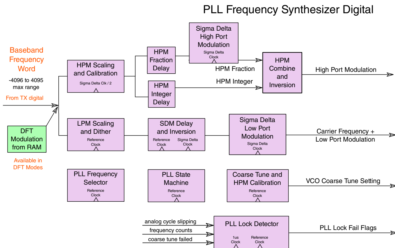
Figure 45-14. PLL Frequency Synthesizer
