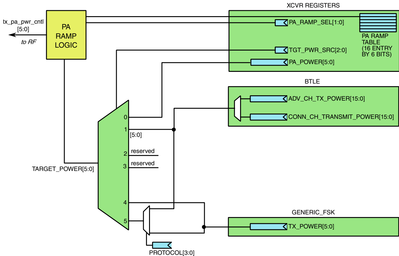
Figure 45-60. PA Target Power Selection
