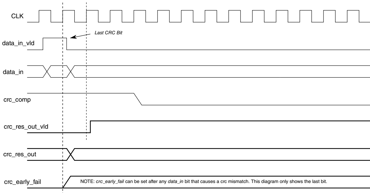
Figure 45-92. CRC Result Out Valid Timing Diagram
