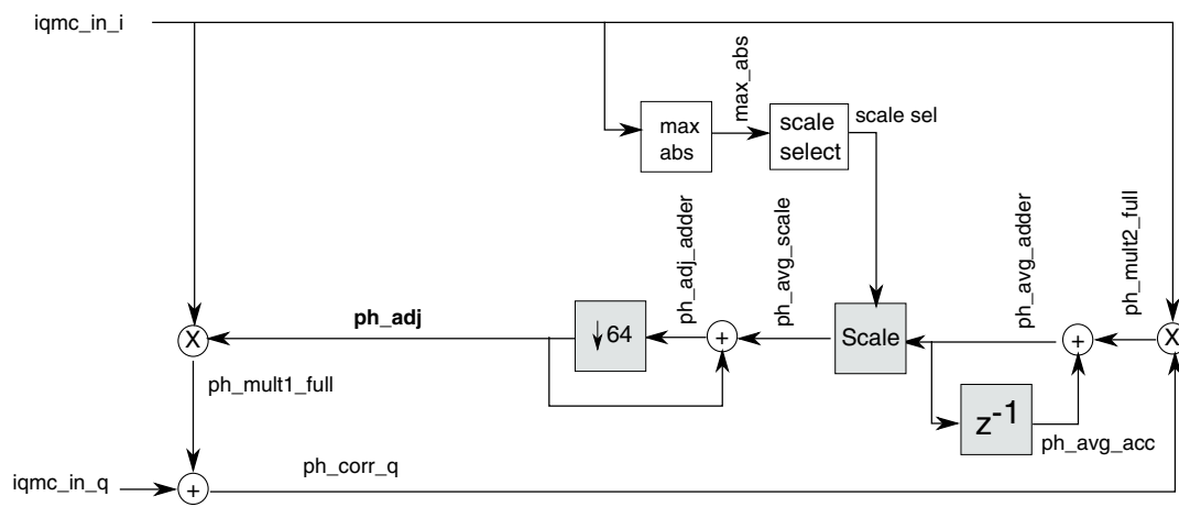
Figure 45-36. I/Q Phase Mismatch Calibration Block Diagram
