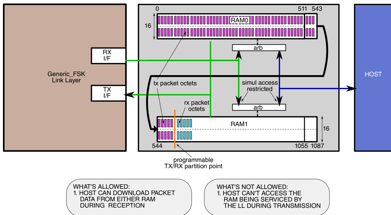
Figure 45-125. RAM ALLOCATIONS FOR GENERIC_FSK
