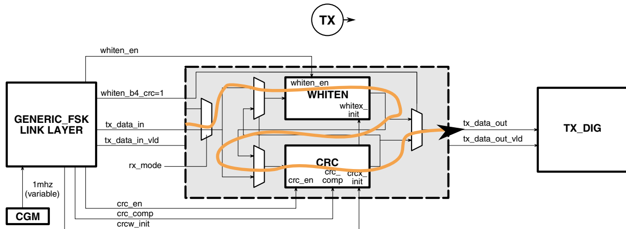
Figure 45-112. Whitening Before CRC (TX)
