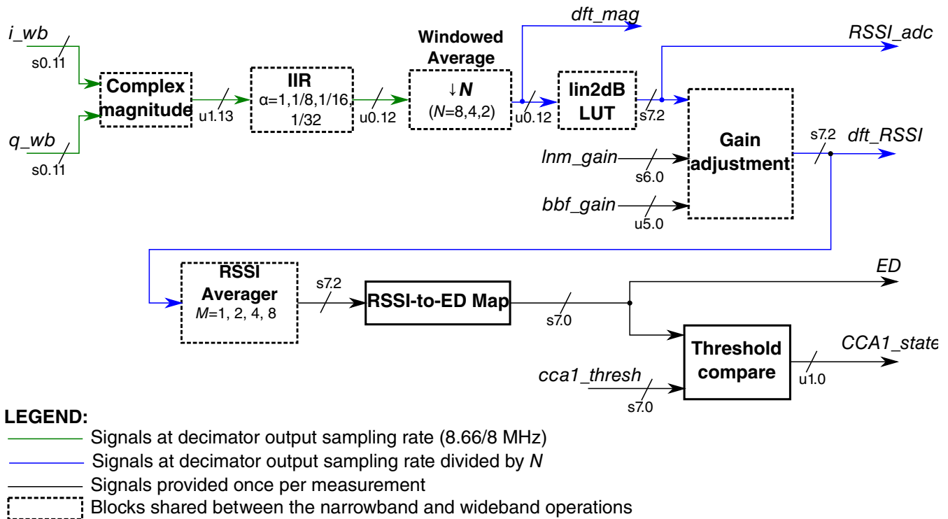
Figure 45-33. Block diagram instantiated for wideband mode
