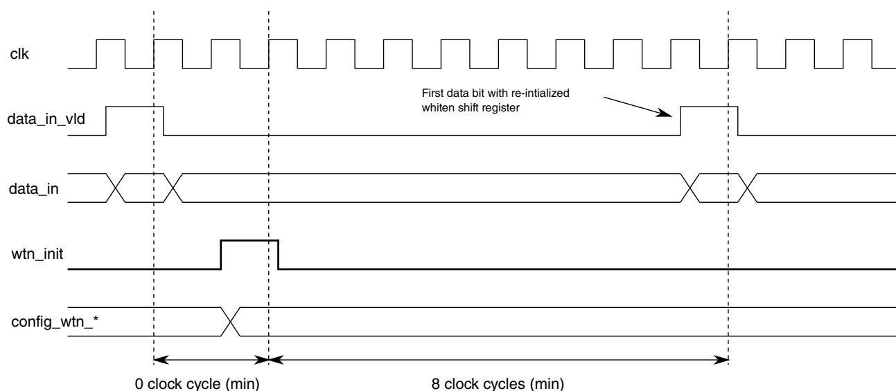
Figure 45-89. Whiten Re-Initialization Timing Diagram
