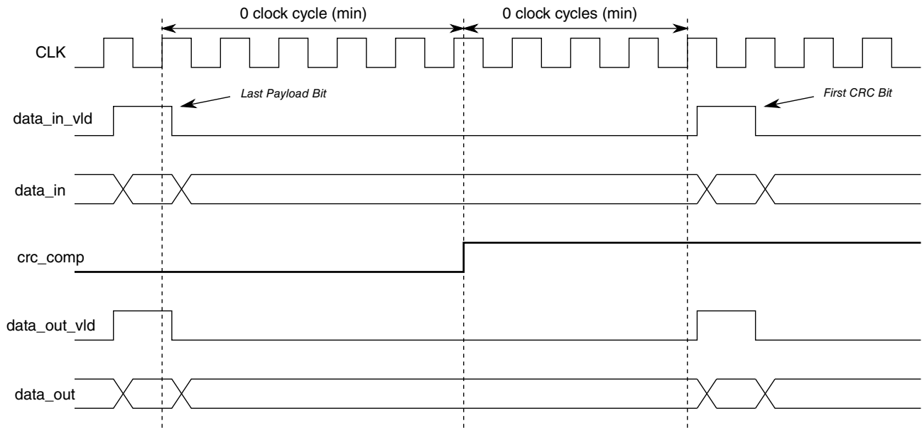
Figure 45-91. CRC Complete Timing Diagram
