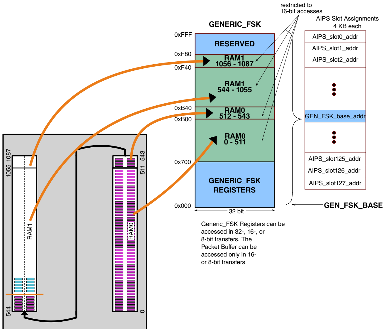
Figure 45-129. GENERIC_FSK MEMORY MAPPING
