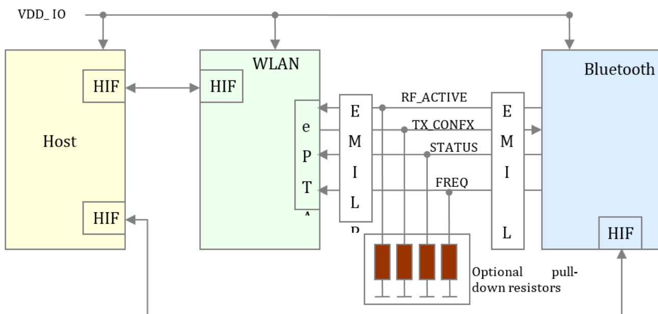
Figure 45-76. 4-WIRE THIRD PARTY INTERFACE
