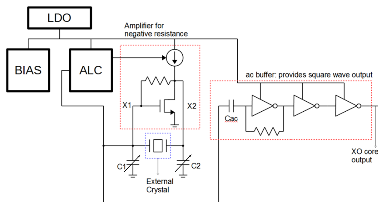
Figure 45-99. XO circuit diagram
