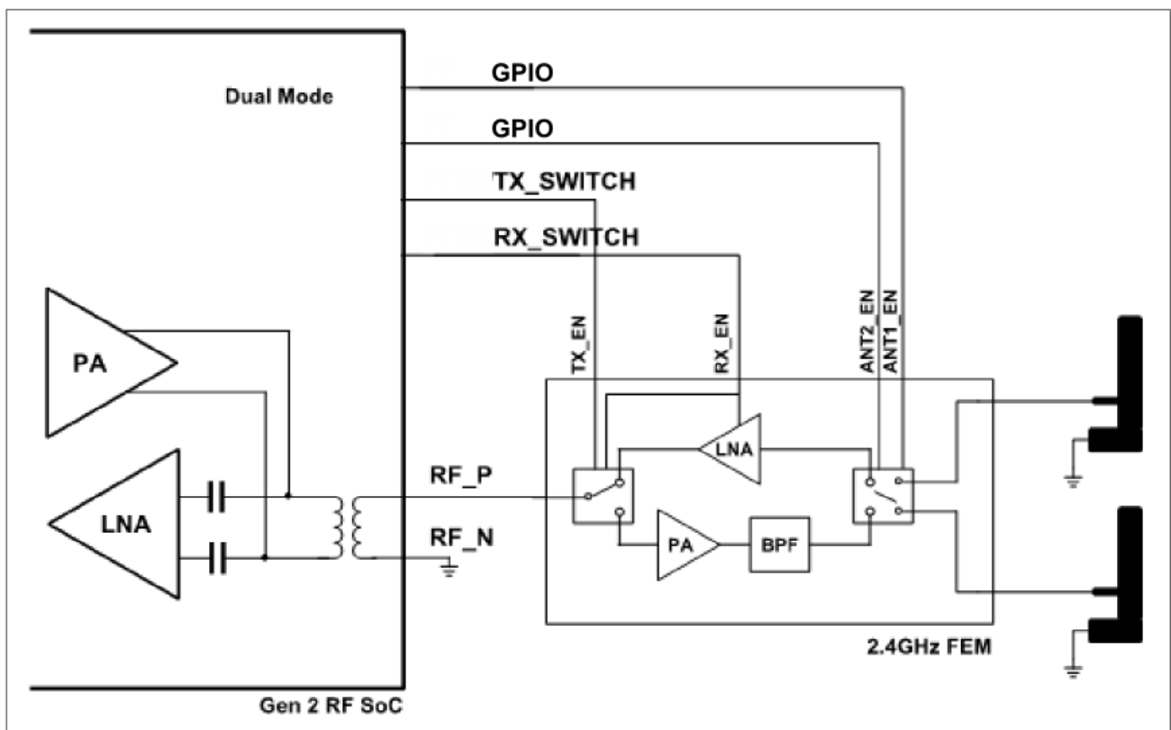
Figure 45-70. FEM Interface Dual Mode
