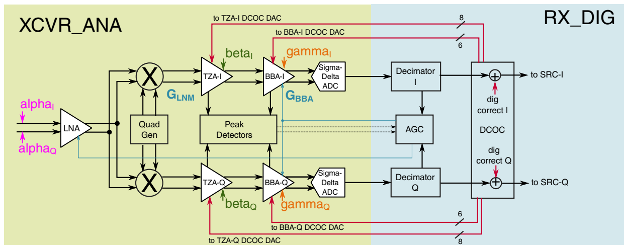
Figure 45-44. Receiver model showing three contributors of DC offset
