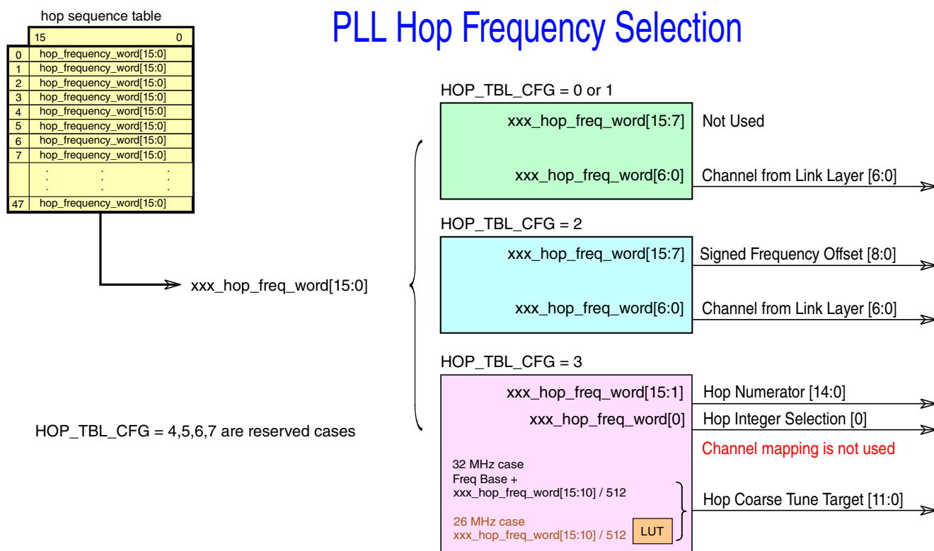
Figure 45-16. PLL Hop Frequency Selection
