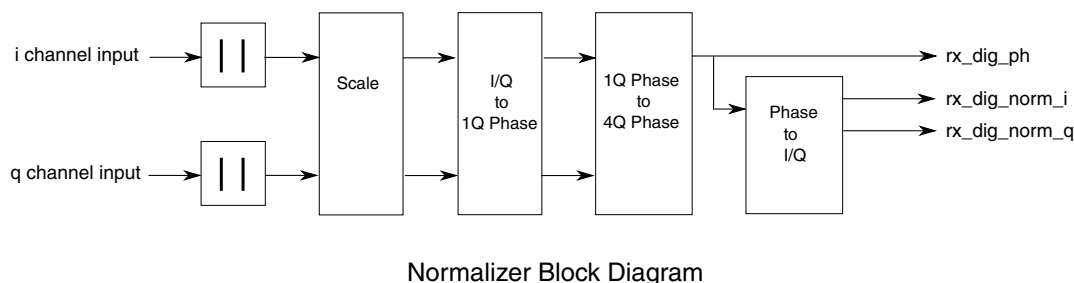
Figure 45-49. Normalizer Block Diagram
