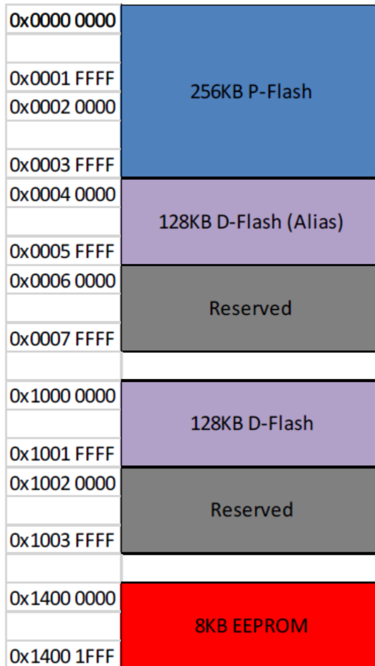
Figure 4-23. KW36 Flash Memory Map, 128 KB D-flash and 128 KB EEPROM Backup Partition
