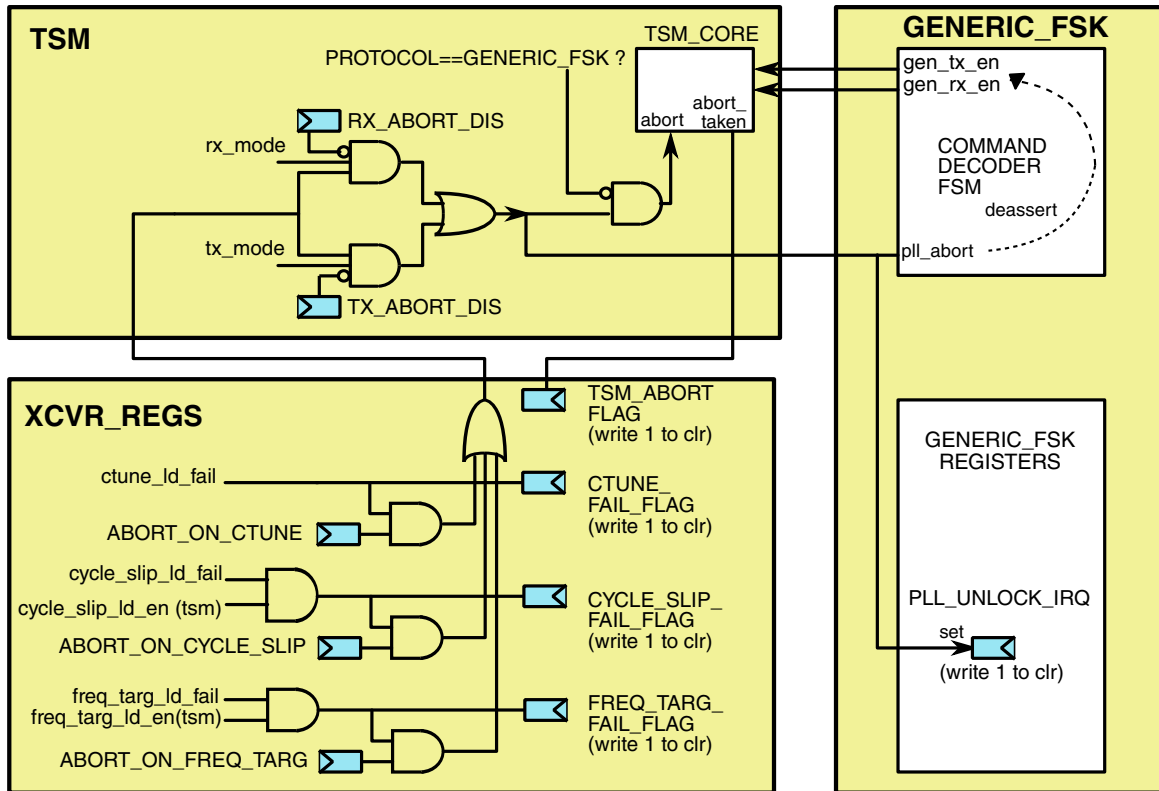
Figure 45-58. GENERIC_FSK PLL UNLOCK HANDLING
