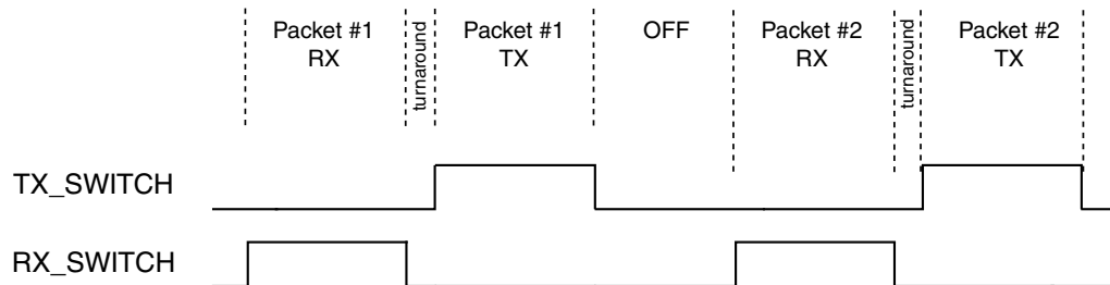
Figure 45-69. FEM Dual Mode Timing
