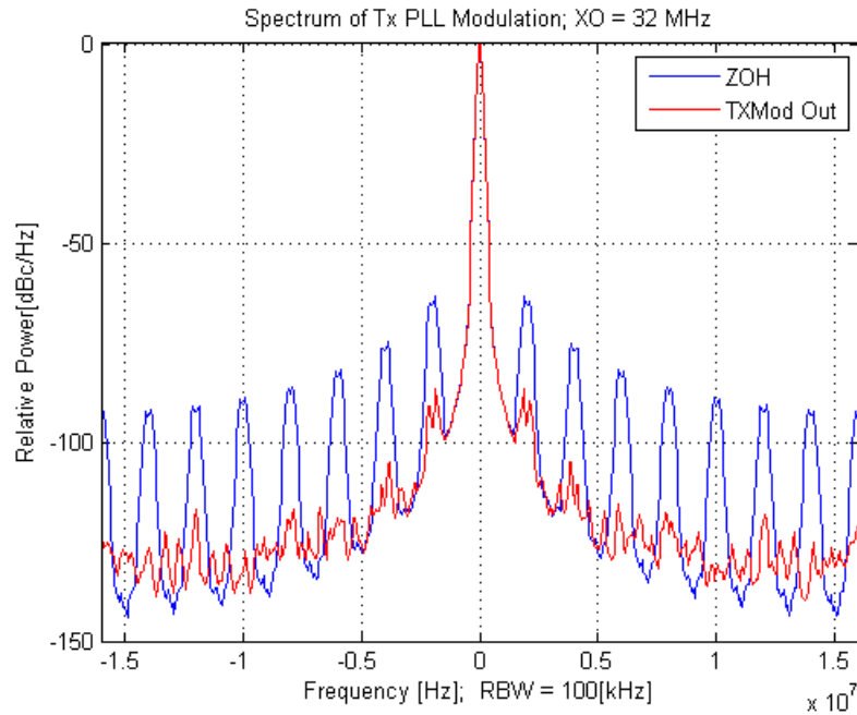
Figure 45-13. Comparison of Transmit Modulation Images at the PLL Output for 250 kbps GMSK
