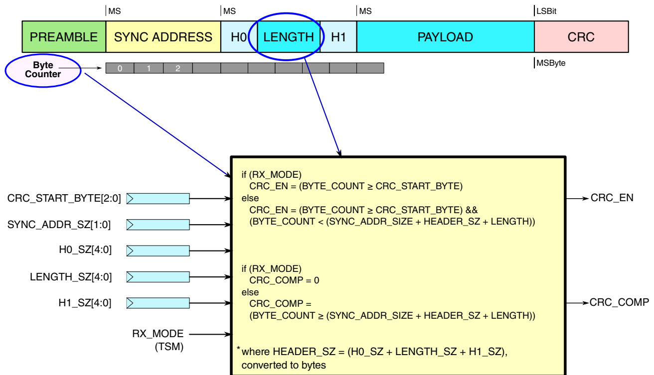
Figure 45-110. GENERIC FSK: CONTROL OF CRC
