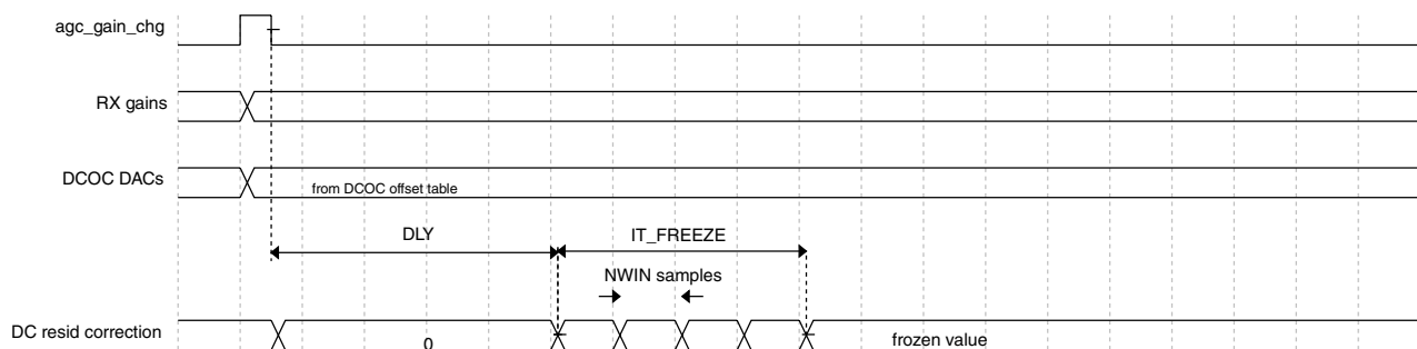
Figure 45-46. DC residual mode 1 timing
