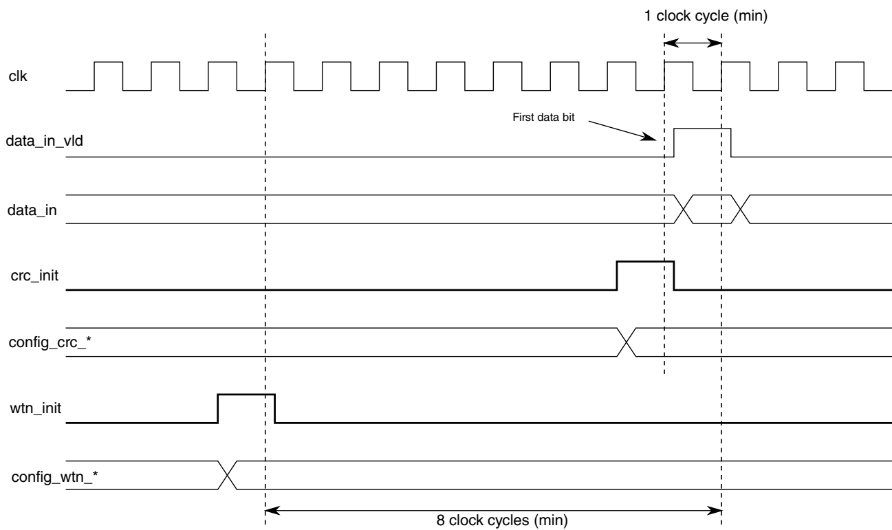
Figure 45-88. Initialization Timing Diagram
