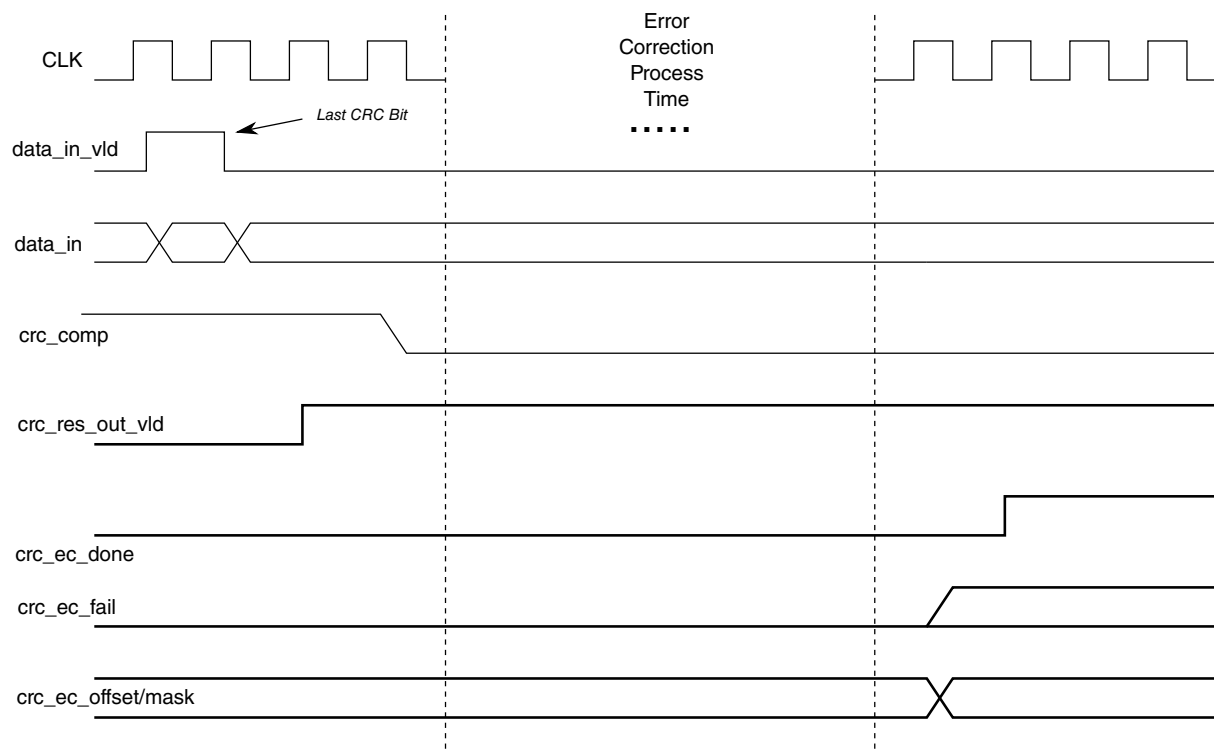
Figure 45-93. CRC Error Correction Done Timing Diagram
