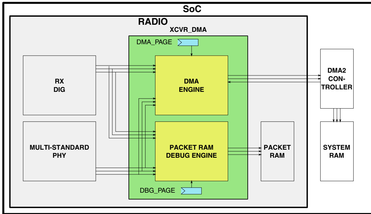
Figure 45-95. Transceiver DMA and Packet RAM Debug
