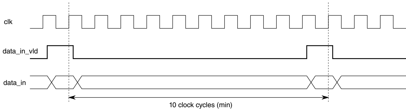
Figure 45-87. Maximum Bitrate Timing Diagram
