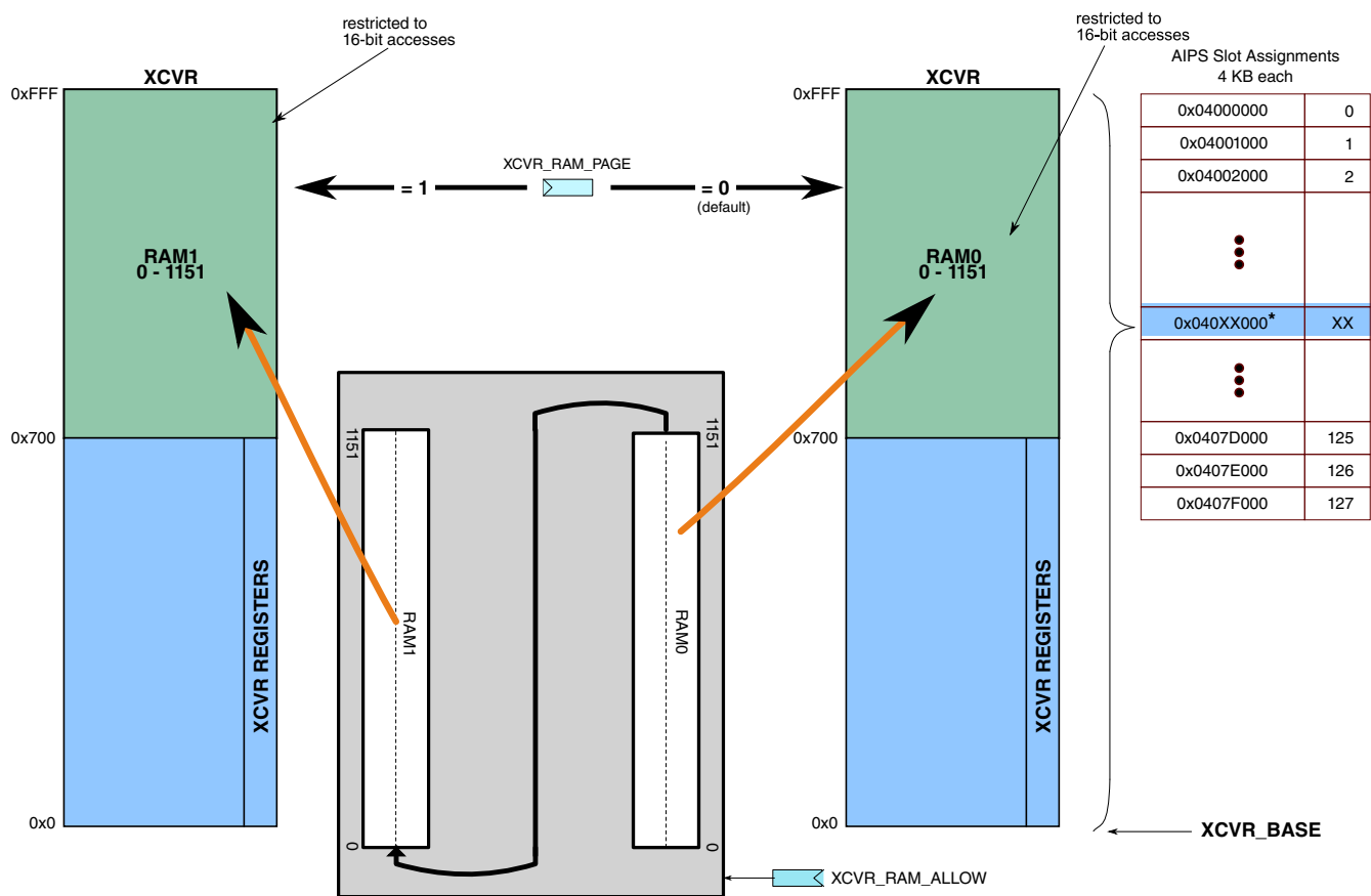
Figure 45-97. Packet RAM Memory Mapping in XCVR Space
