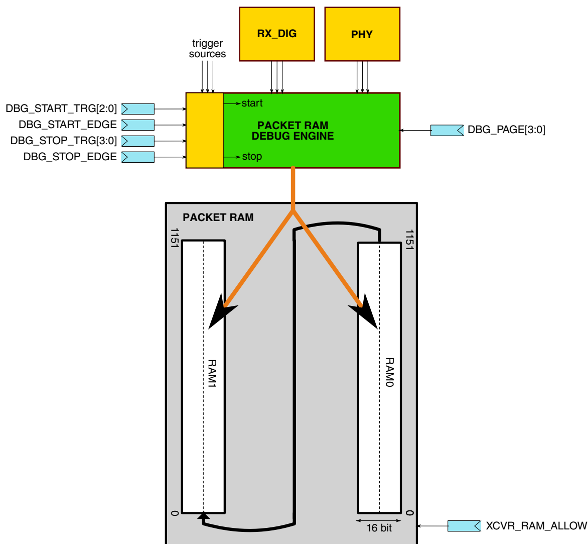
Figure 45-96. Packet RAM Debug Mode Block Diagram
