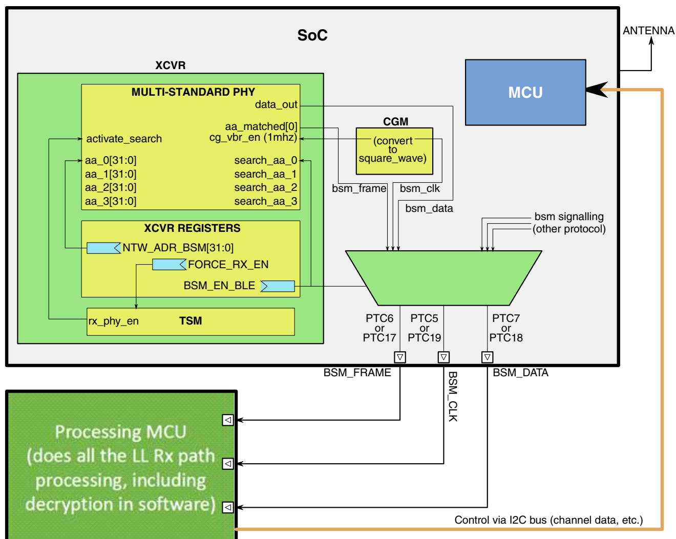
Figure 45-52. BSM Block Diagram
