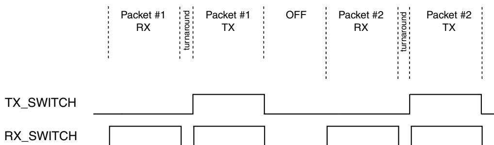
Figure 45-67. FEM Single Mode Timing
