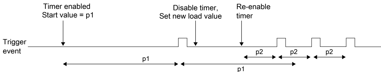
Figure 34-3. Modifying running timer period
