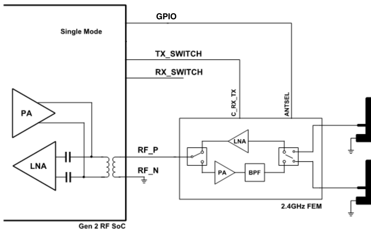
Figure 45-68. FEM Interface Single Mode
