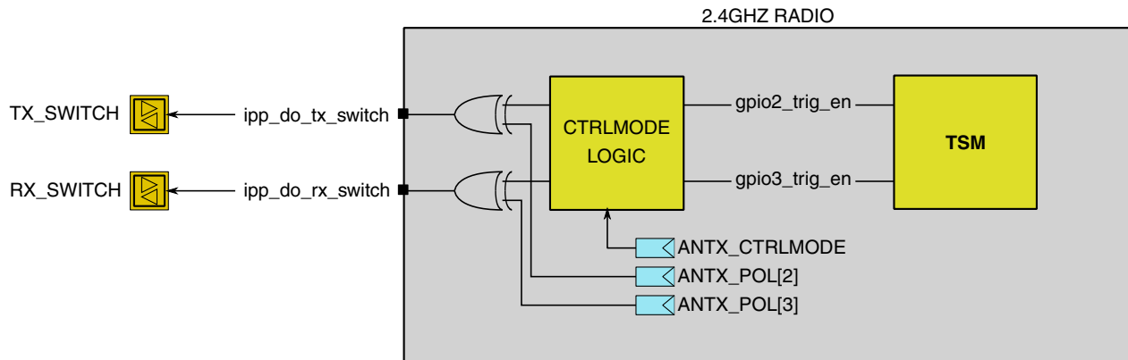
Figure 45-65. FEM Common Pin Interface
