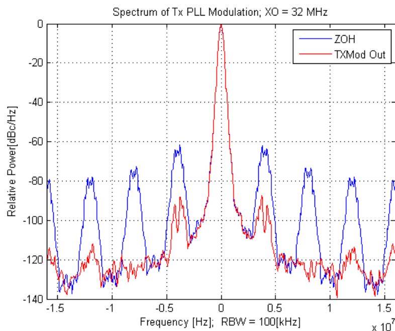
Figure 45-12. Comparison of Transmit Modulation Images at the PLL Output for 500 kbps GMSK
