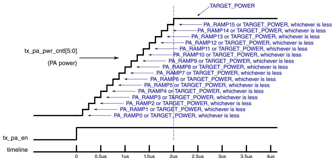
Figure 45-62. 2μS PA RAMP UP (32MHZ TIMING)
