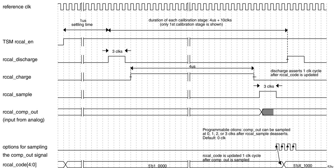
Figure 45-51. RX RCCAL timing
