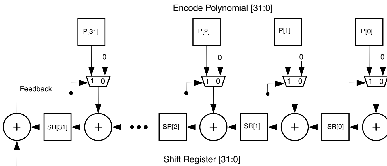
Figure 45-82. CRC Calculation Shift Register
