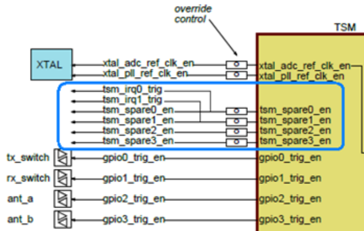
Figure 45-80. TSM Interrupt Re-use Scheme
