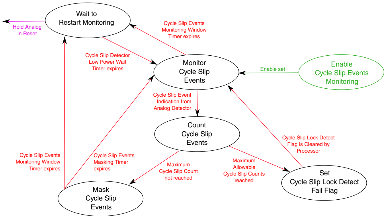
Figure 45-23. PLL Lock Detect State Machine
