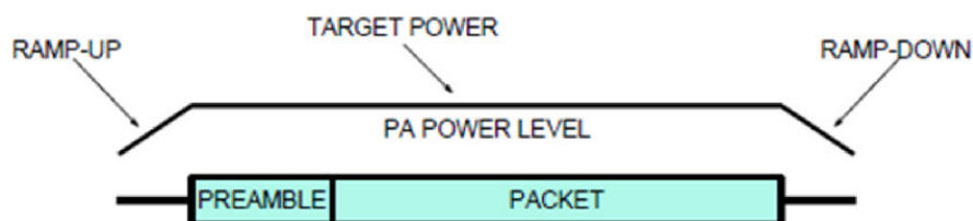
Figure 45-7. Power Amplifier Ramping
