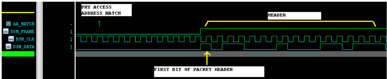
Figure 45-53. BSM Timing Diagram
