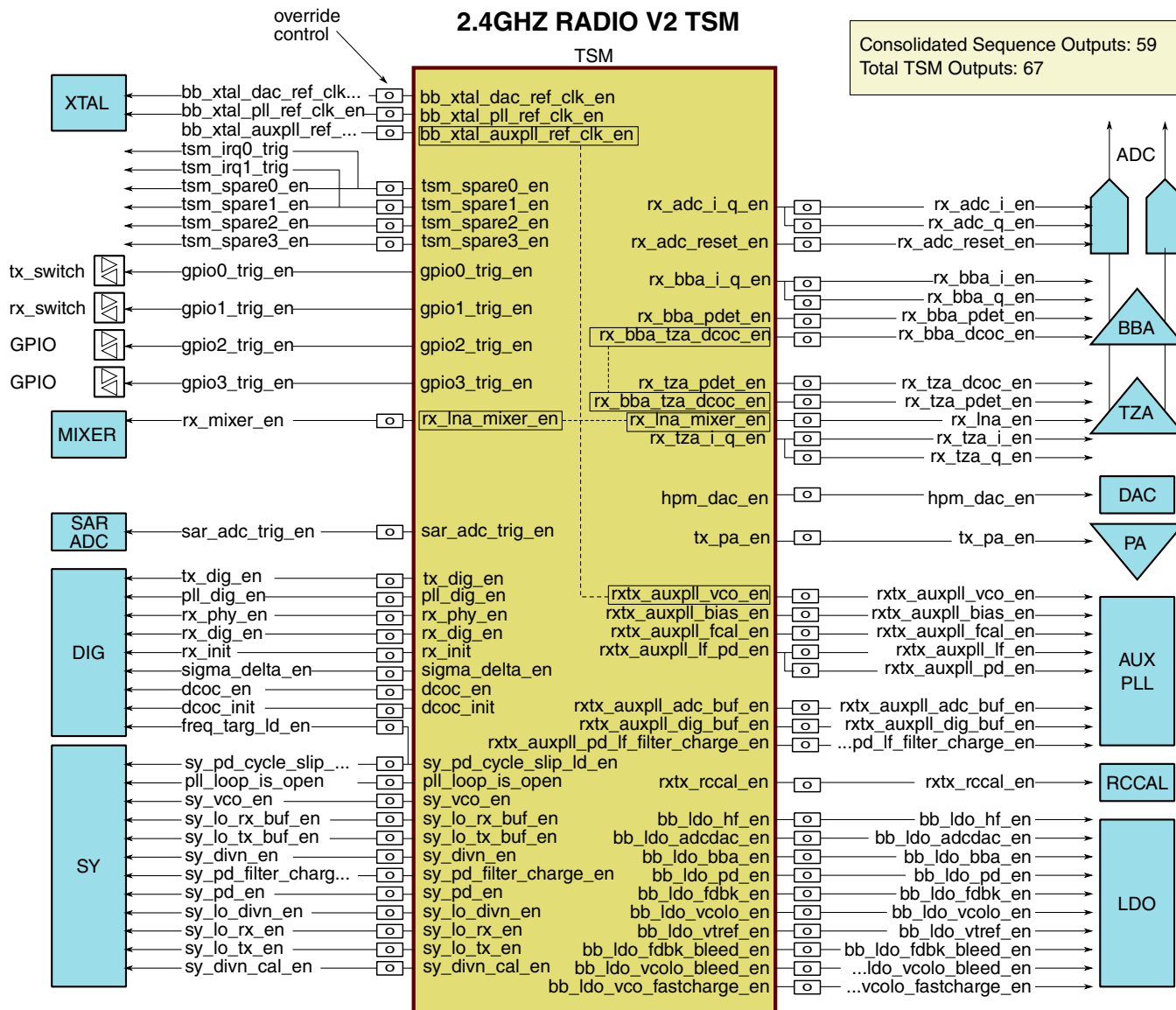
Figure 45-54. Block diagram
