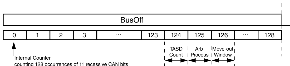
Figure 37-11. Arbitration at the end of bus off and move-out time windows
