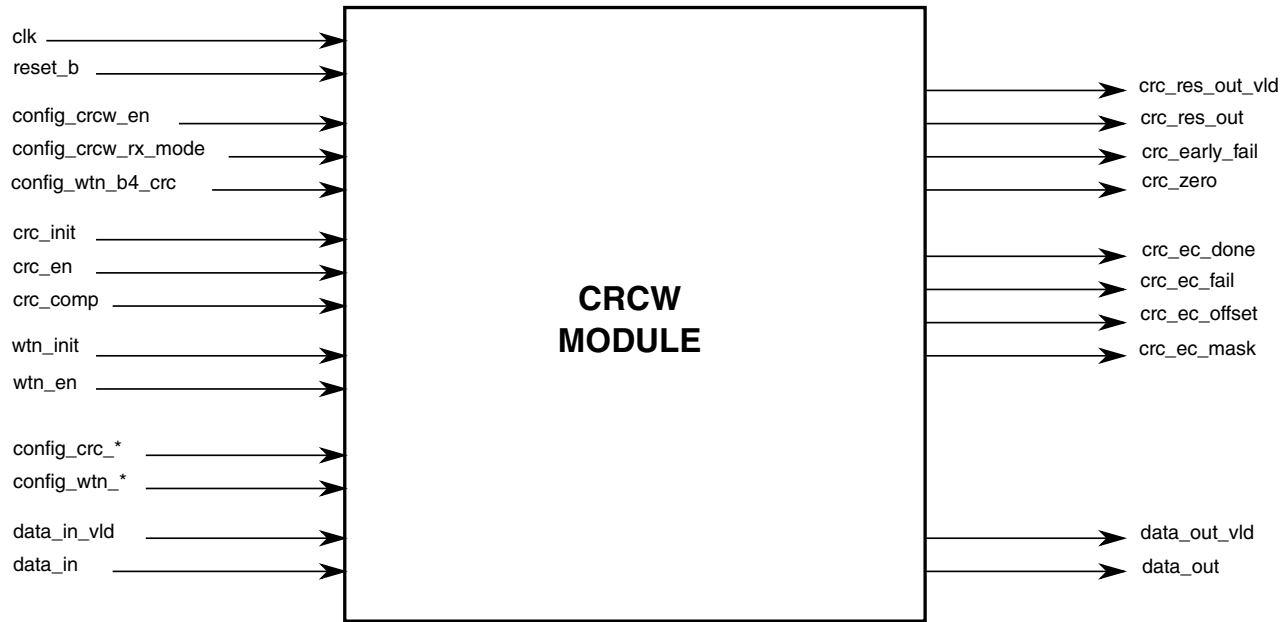
Figure 45-81. CRCW Block Diagram
