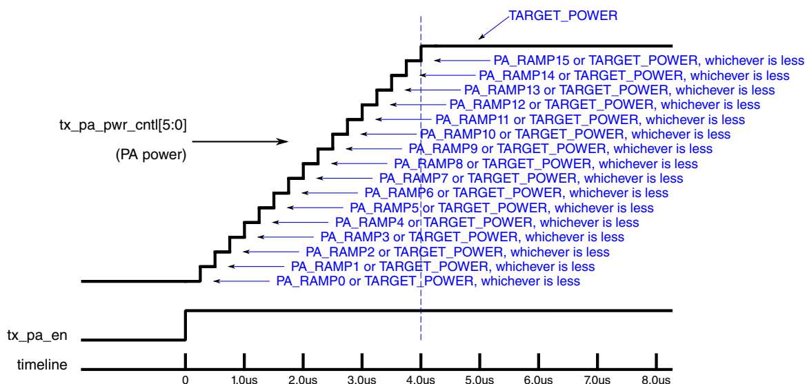
Figure 45-63. 4μS PA RAMP UP (32MHZ TIMING)
