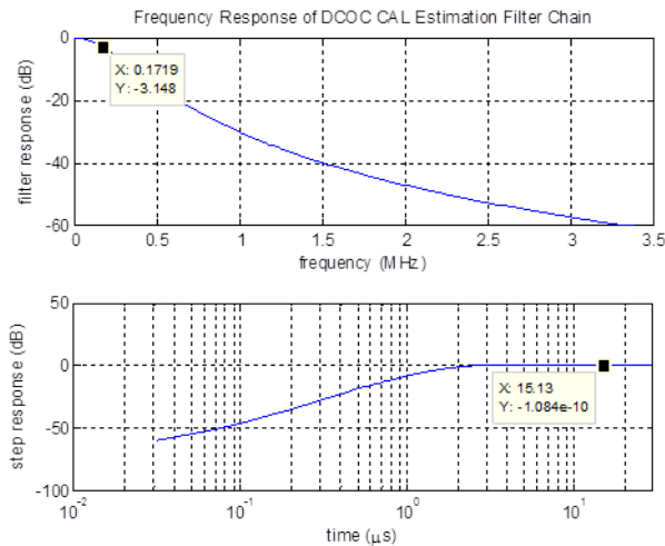
Figure 45-42. Magnitude and Step response of DC Offset Calibration Estimator
