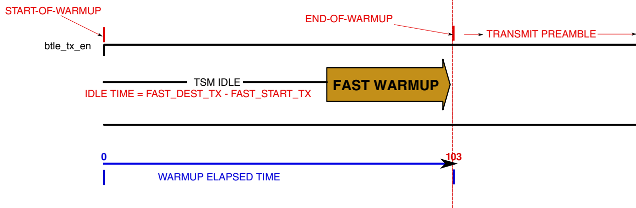
Figure 45-73. Nominal vs. Fast TX Warmups
