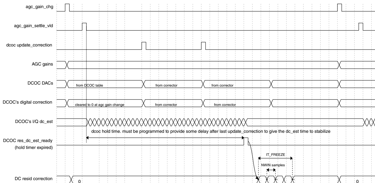
Figure 45-47. DC residual mode 2 timing
