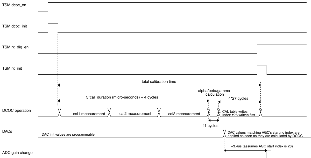
Figure 45-40. DCOC Calibration Timing Diagram
