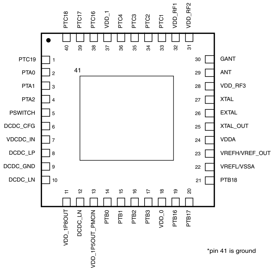
Figure 3-3. 40-pin "Wettable" QFN pinout diagram
