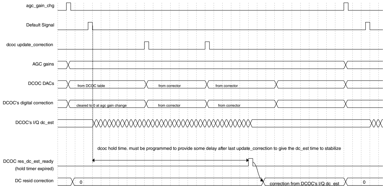
Figure 45-48. DC residual mode 3 timing
