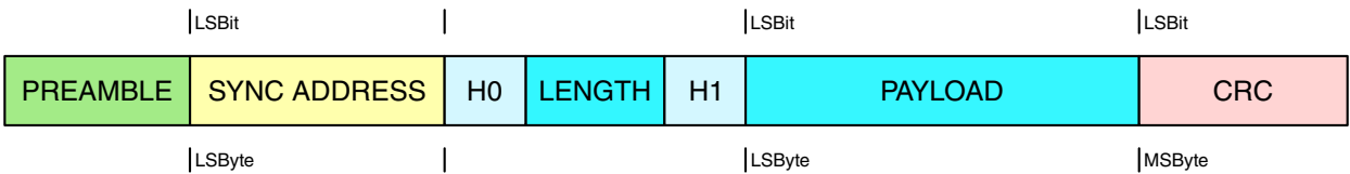
Figure 45-100. GENERIC_FSK Packet Structure
