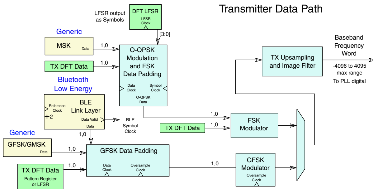
Figure 45-6. Transmitter Digital
