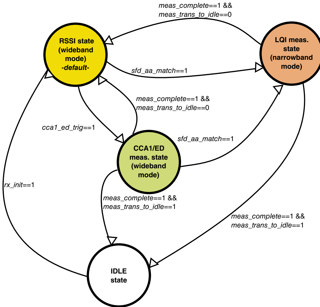
Figure 45-32. Module state machine
