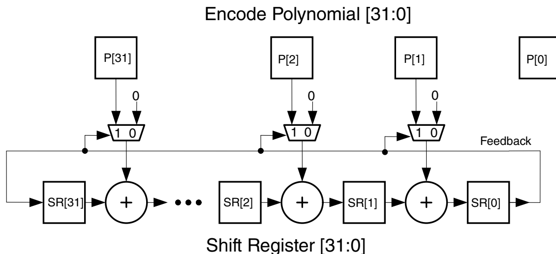
Figure 45-86. CRC Correction Shift Register
