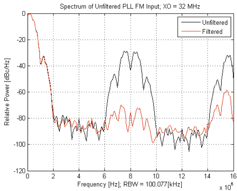
Figure 45-10. Comparison of Transmit Modulation Images at the PLL Input for BLE
