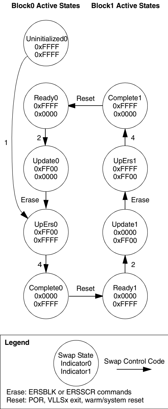
Figure 29-15. Valid Swap State Sequencing
