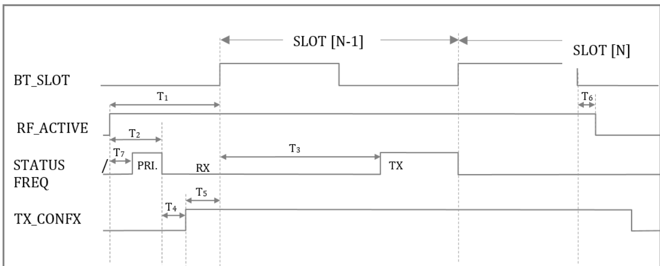
Figure 45-77. IDEAL RF_ACTIVE TIMING (NO GLITCH)
