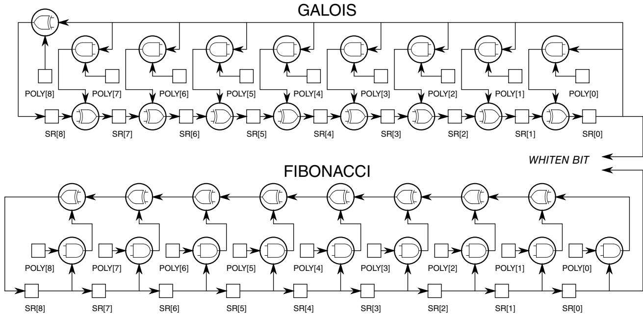
Figure 45-85. Data Whitening Shift Register
