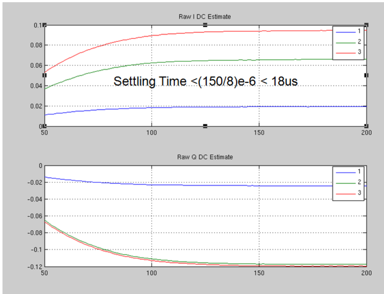
Figure 45-43. 3-step {I,Q} DC estimation during calibration
