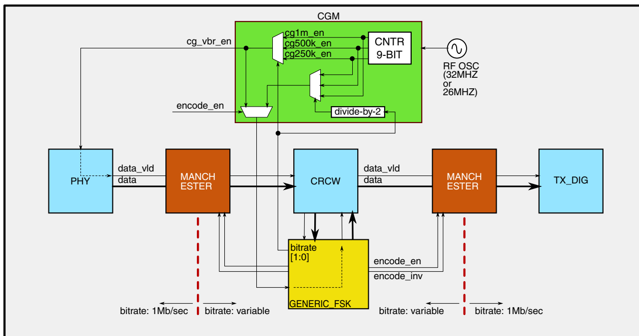
Figure 45-118. BITSTREAM PROCESSING WITH MANCHESTER ENCODING
