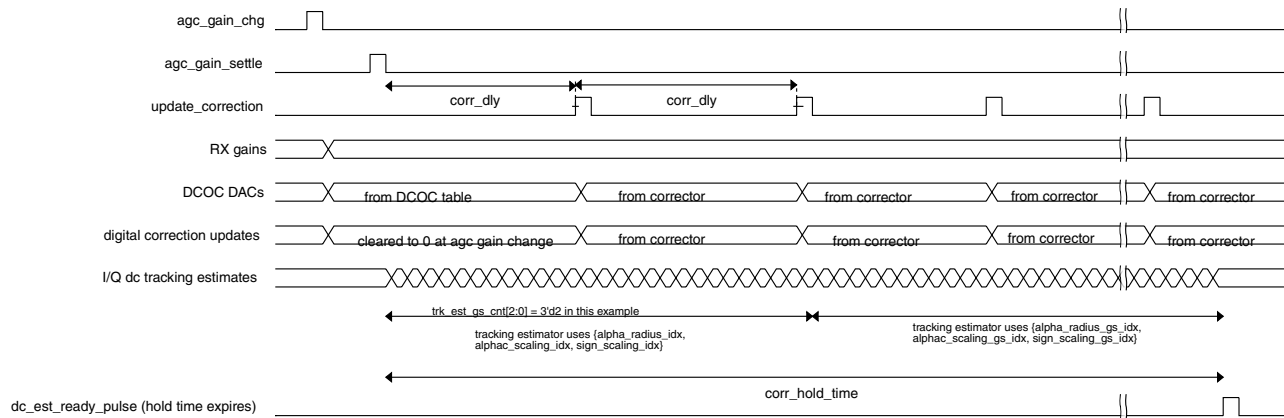
Figure 45-45. DC Offset Tracking Correction Timing
