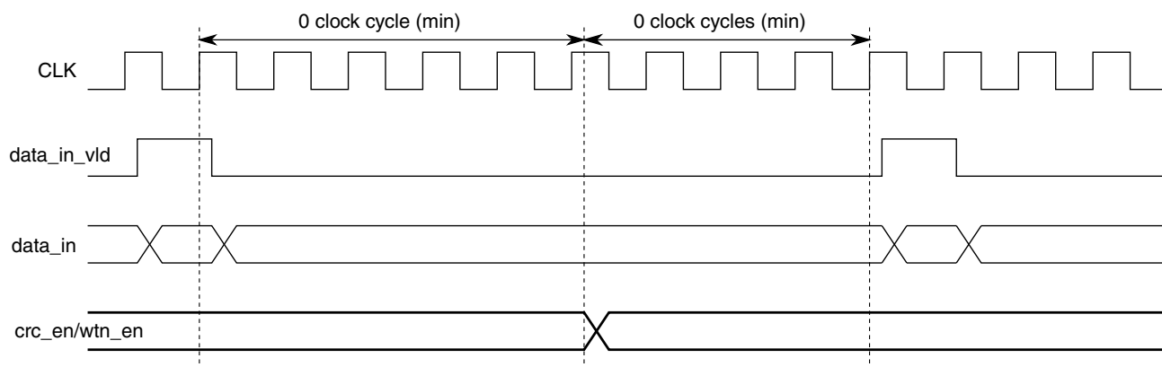
Figure 45-90. CRC/WTN Enable Timing Diagram
