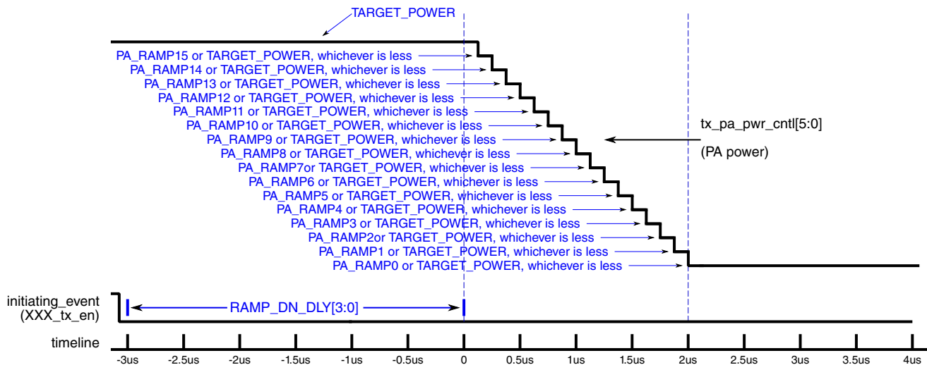
Figure 45-64. PA RAMP DOWN (32MHZ TIMING)
