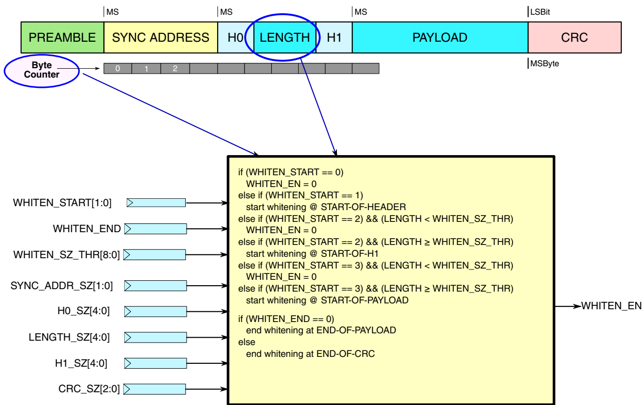
Figure 45-111. GENERIC FSK: CONTROL OF WHITENING
