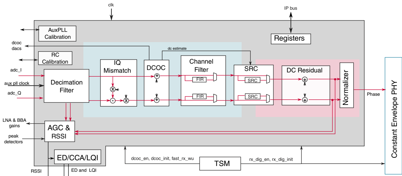
Figure 45-26. RX DIG Block diagram
