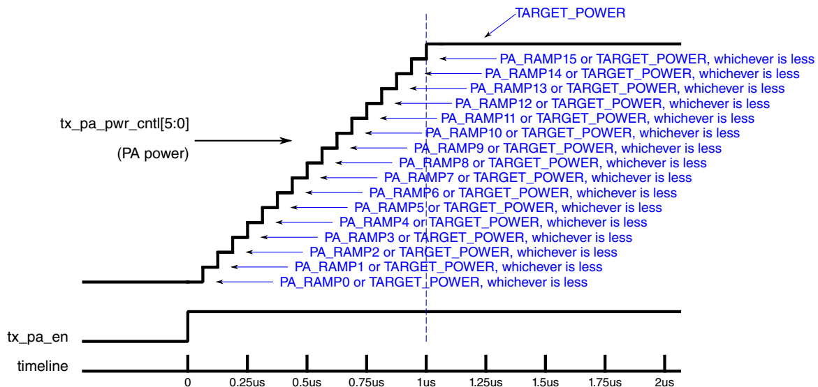
Figure 45-61. 1μS PA RAMP UP (32MHZ TIMING)
