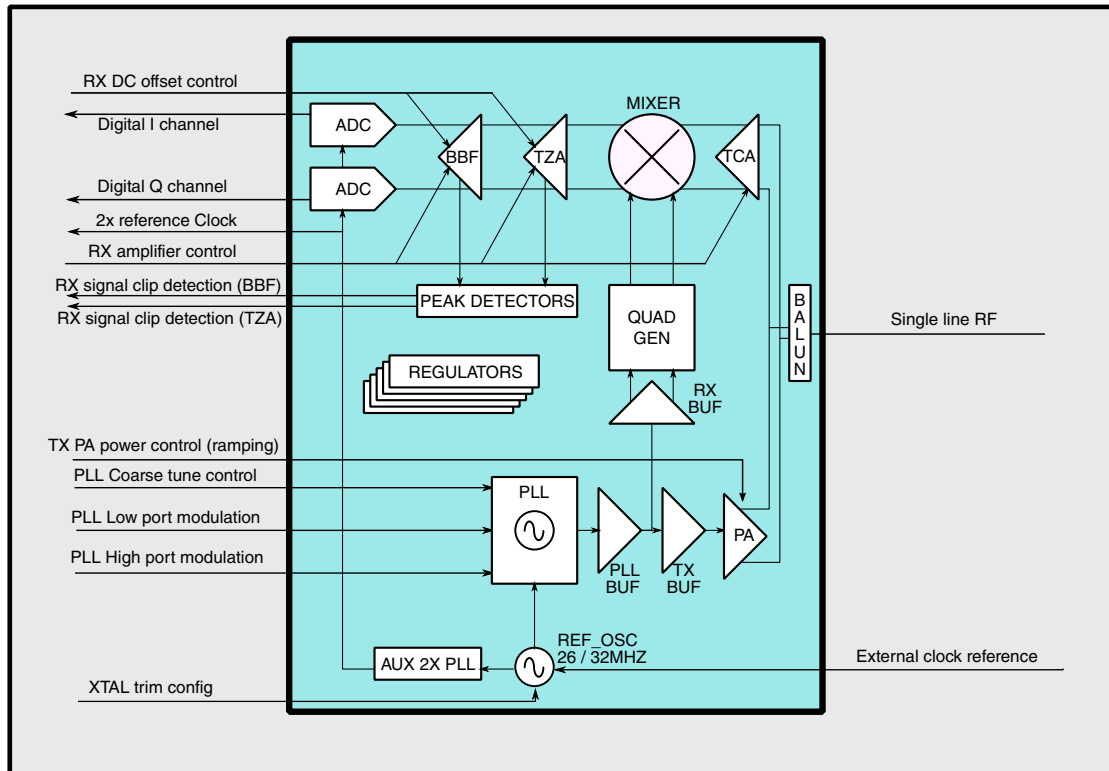
Figure 45-98. Analog Radio Block diagram
