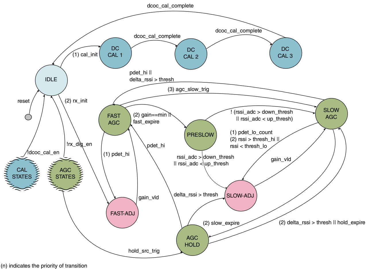
Figure 45-30. AGC State Machine
