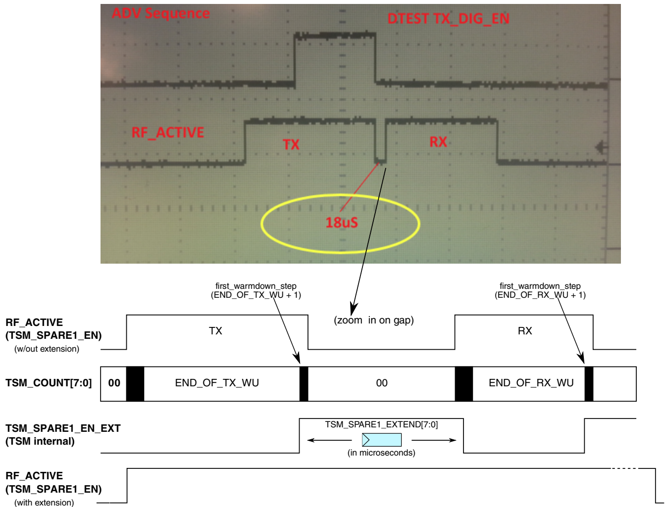
Figure 45-79. TSM_SPARE1_EN EXTENSION
