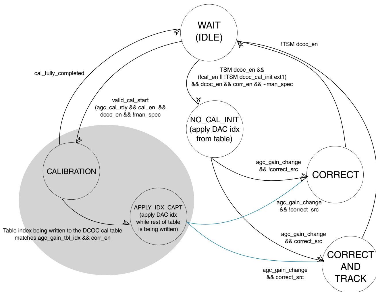
Figure 45-39. DCOC State Diagram
