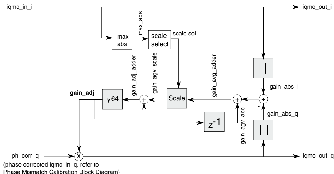
Figure 45-35. I/Q Gain Mismatch Calibration Block Diagram
