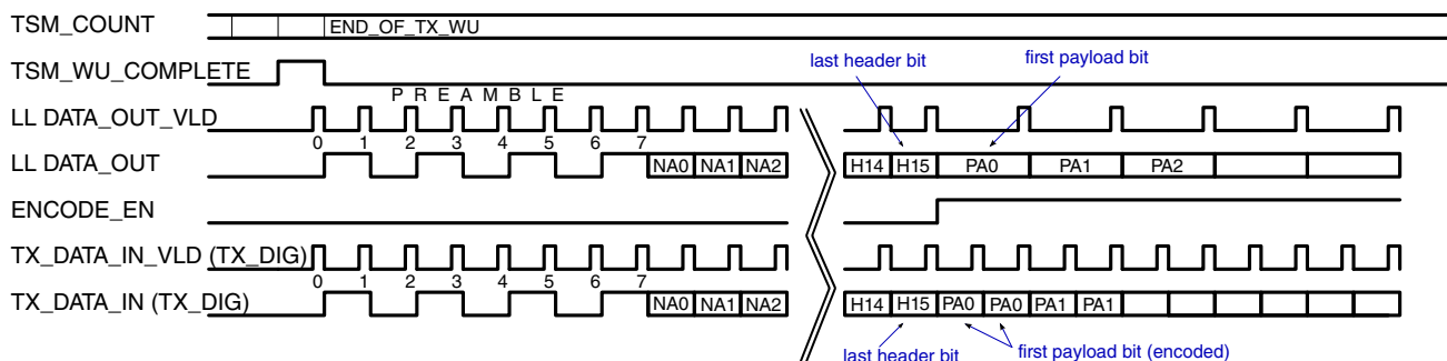
Figure 45-119. BIT STREAM PROCESSING (WITH MANCHESTER) TX TIMING -- 1MBIT/SEC OTA
