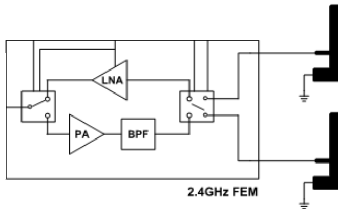
Figure 45-66. FEM Block Diagram
