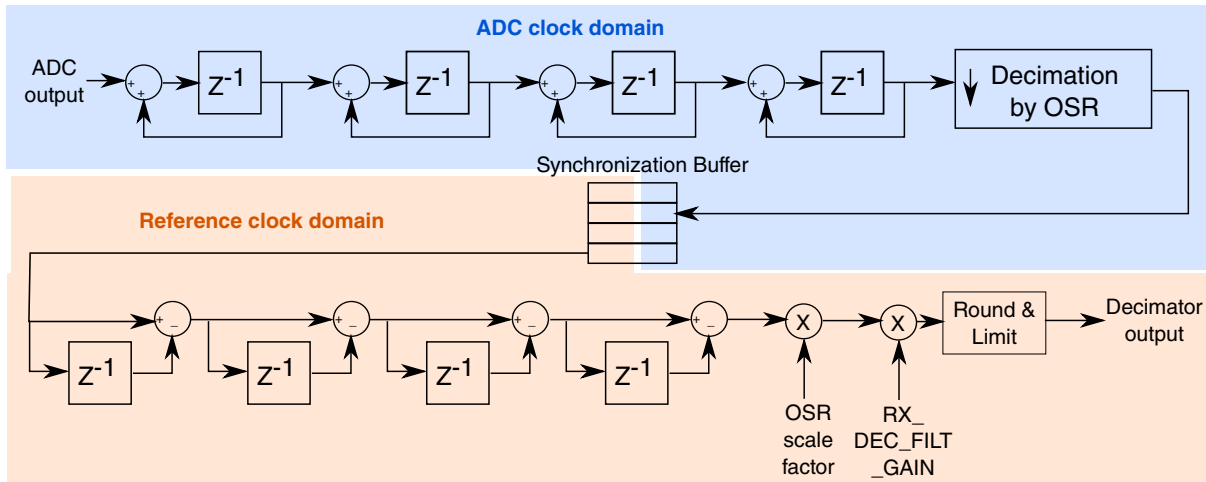
Figure 45-27. Decimation Filter Block Diagram
