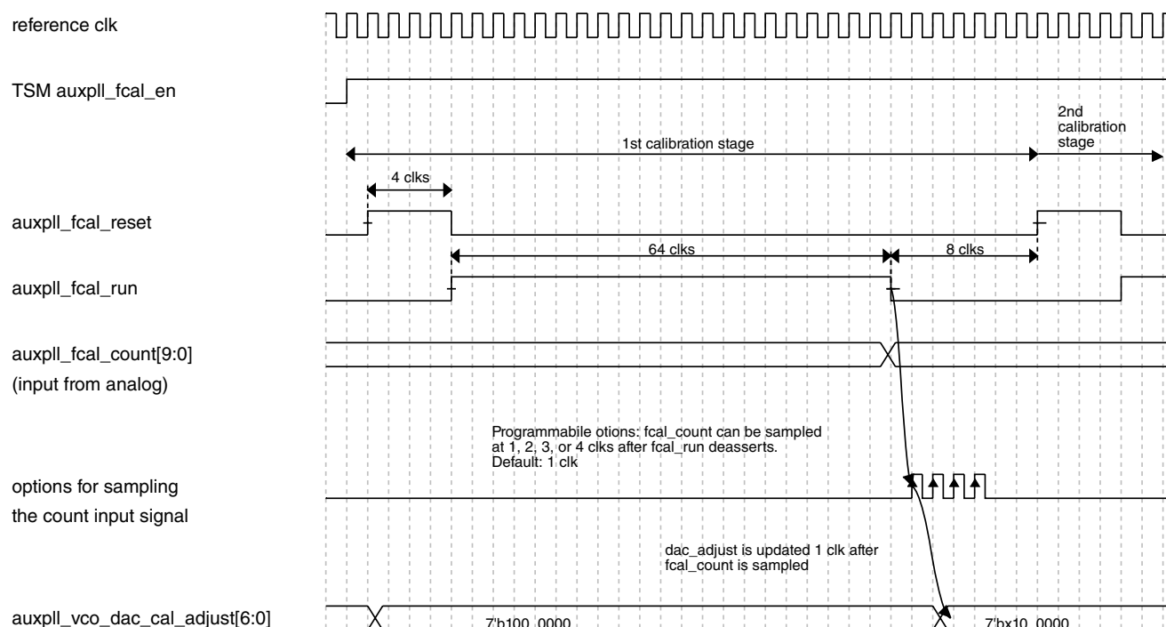
Figure 45-50. RX AuxPLL FCAL timing
