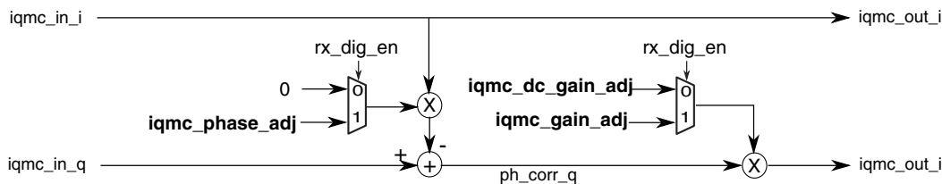
Figure 45-37. I/Q Mismatch Correction Block Diagram
