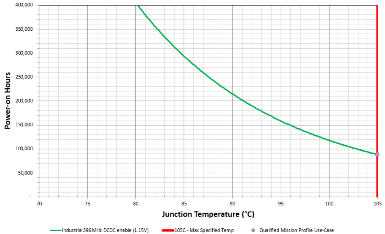
Figure 3. i.MXRT1020 Industrial lifetime estimates DCDC-enabled mode
