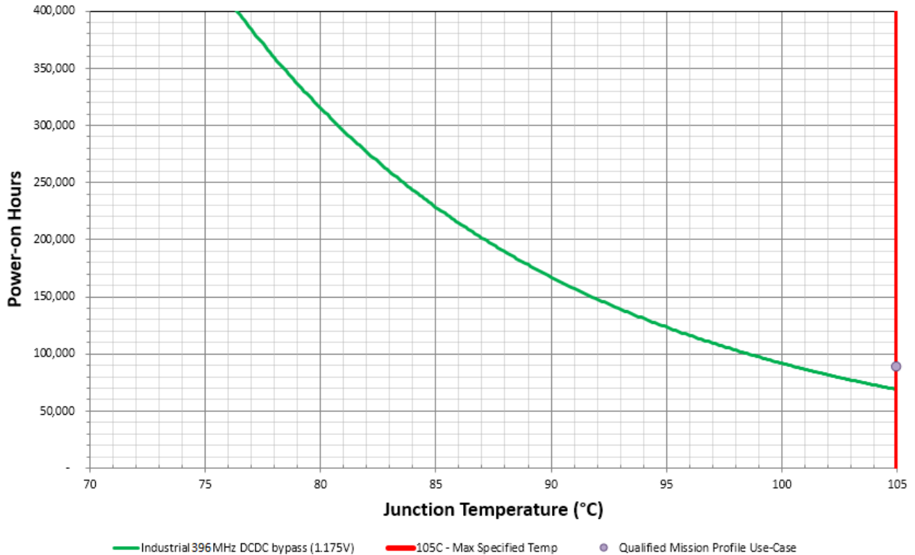
Figure 4. i.MXRT1020 Industrial lifetime estimates DCDC-bypass mode
