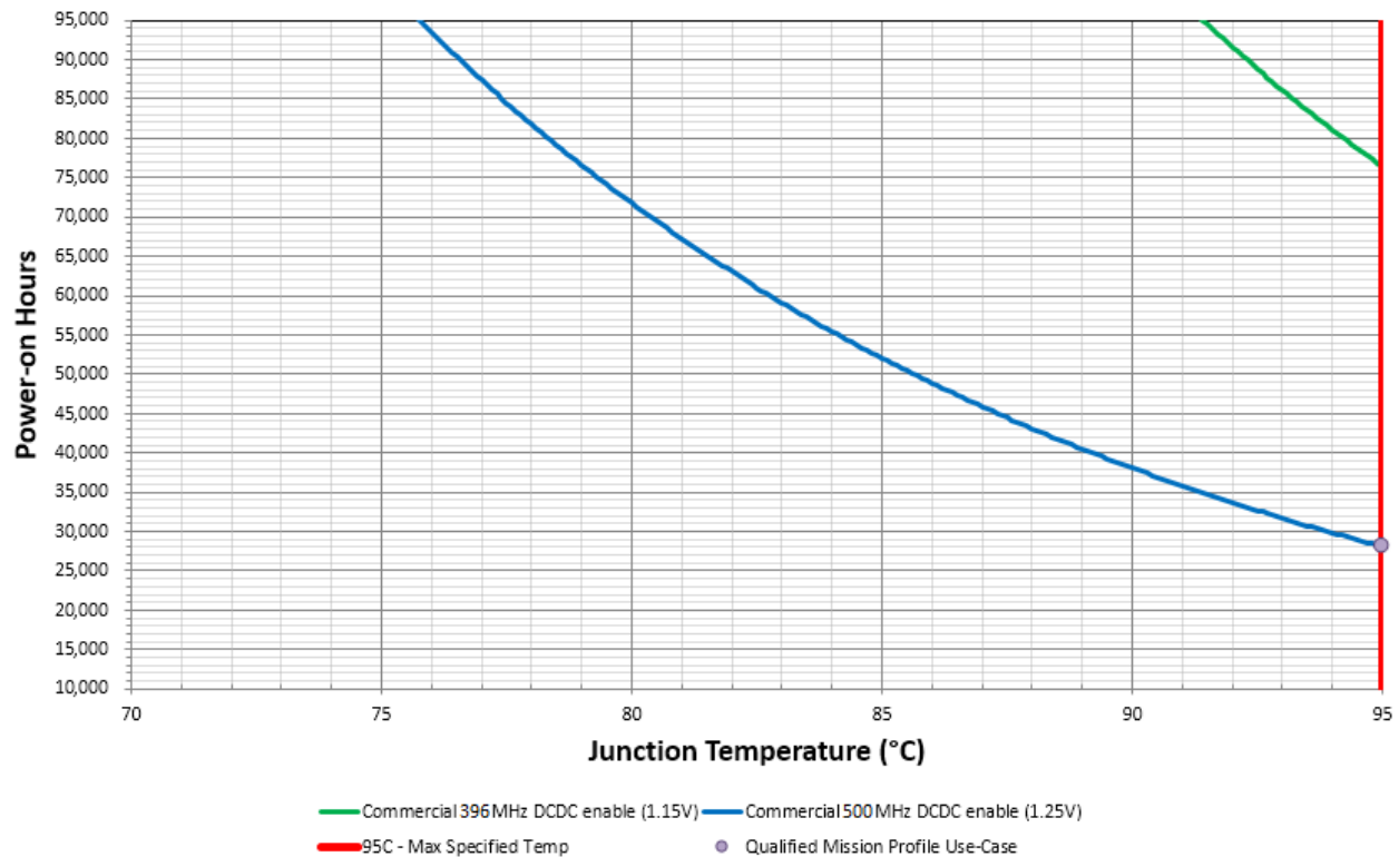
Figure 1. i.MXRT1020 commercial lifetime estimates, DCDC-enabled mode
