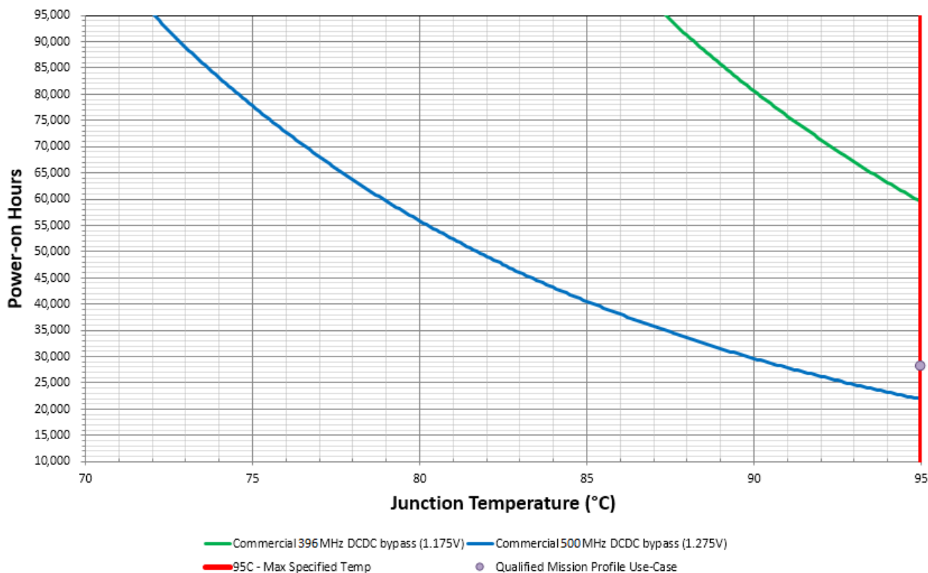
Figure 2. i.MXRT1020 commercial lifetime estimates, DCDC-bypass mode
