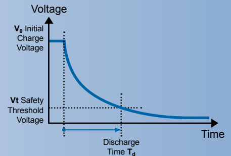
Figure 3 Exponential discharge
