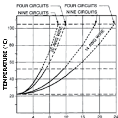
CURRENT (AMPERES) TERMINAL TEMPERATURE VERSUS CURRENT FOR BRASS TERMINALS
