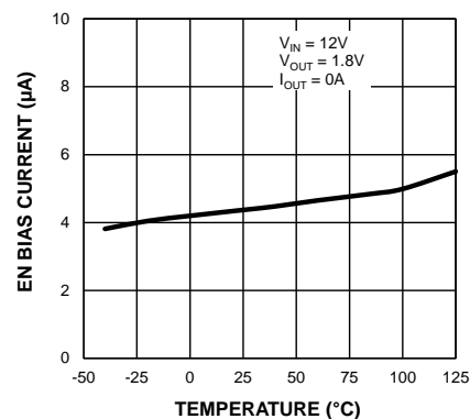
EN Bias Current vs. Temperature
