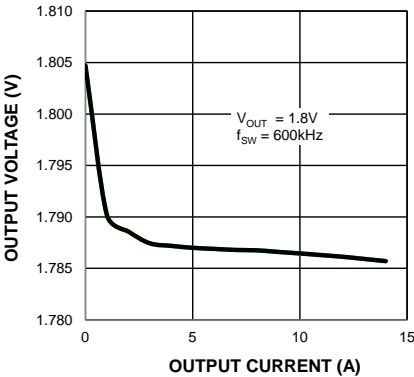
Load Regulation (MIC45212-1)
