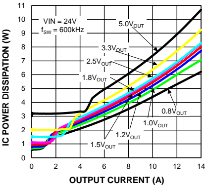
IC Power Dissipation vs. Output Current
