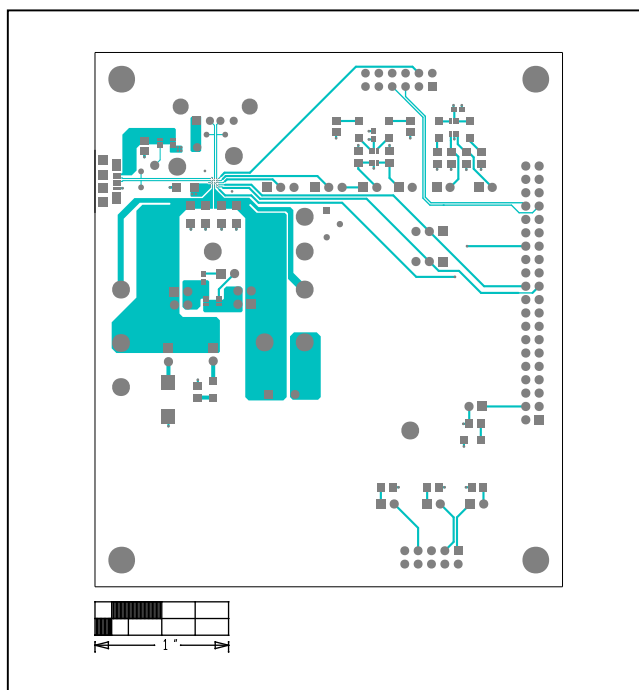
MAX14746 EV Kit—Top
