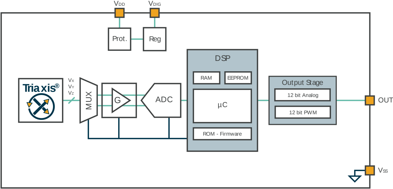
Figure 1: Block diagram
