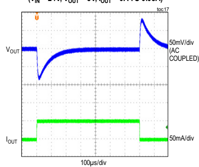
LOAD CURRENT TRANSIENT RESPONSE (V IN = 24V, V OUT = 5V, I OUT = 0A TO 0.05A)
