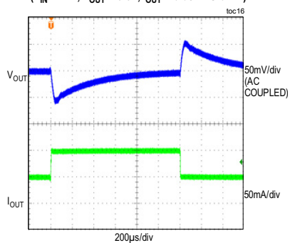
LOAD CURRENT TRANSIENT RESPONSE (V IN = 24V, V OUT = 3.3V, I OUT = 0.05A TO 0.1A)
