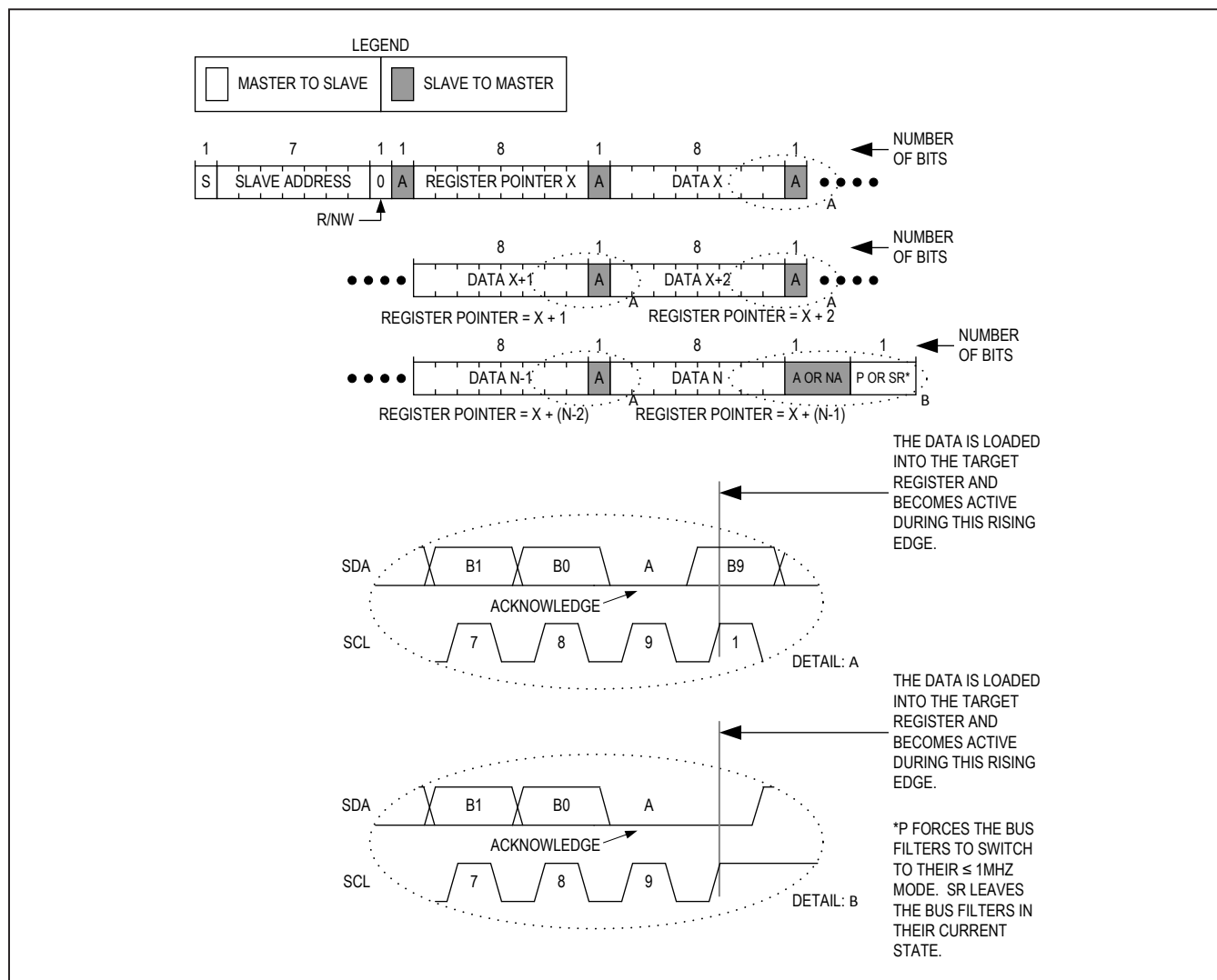
Figure 8. Writing to Sequential Registers X to N
