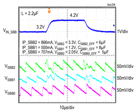
SIMO LINE TRANSIENT
