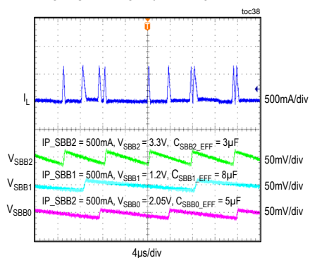
SIMO SWITCHING WAVEFORMS LIGHT UTILIZATION 10mA PER CHANNEL
