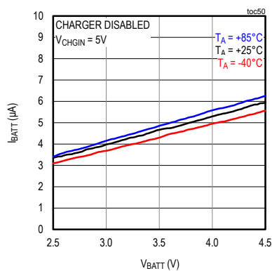
BATT BIAS CURRENT vs. BATT VOLTAGE
