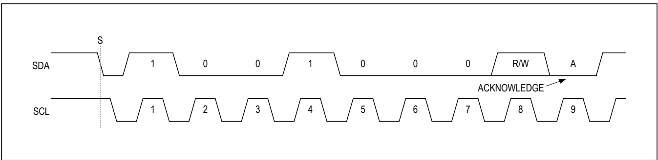
Figure 25. Slave Address Example
