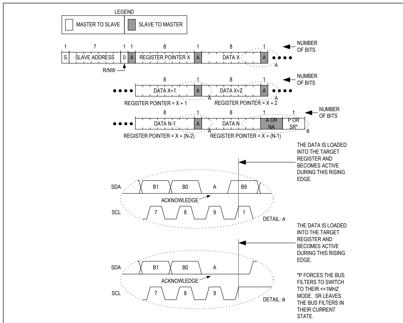
Figure 27. Writing to Sequential registers X to N
