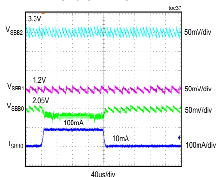
SBB0 LOAD TRANSIENT
