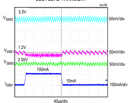
SBB1 LOAD TRANSIENT
