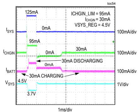
SYS LOAD TRANSIENT CAUSING BATTERY SUPPLEMENT
