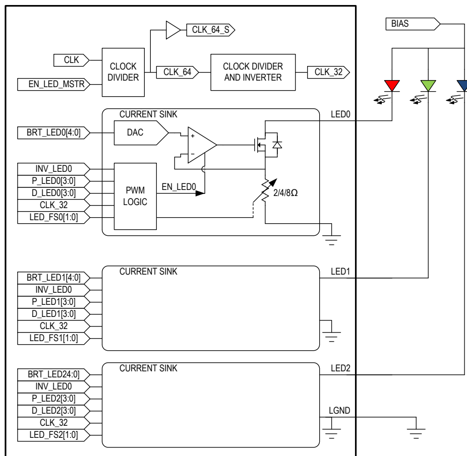
Figure 20. Current Sink Block Diagram
