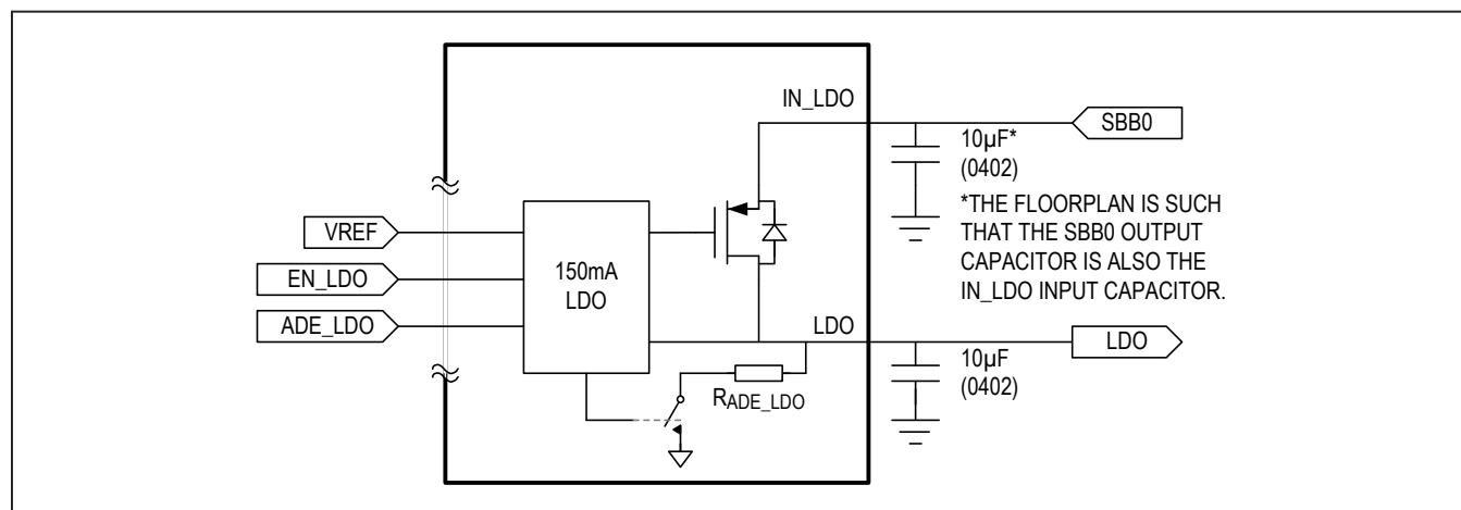
Figure 19. LDO Simplified Block Diagram
