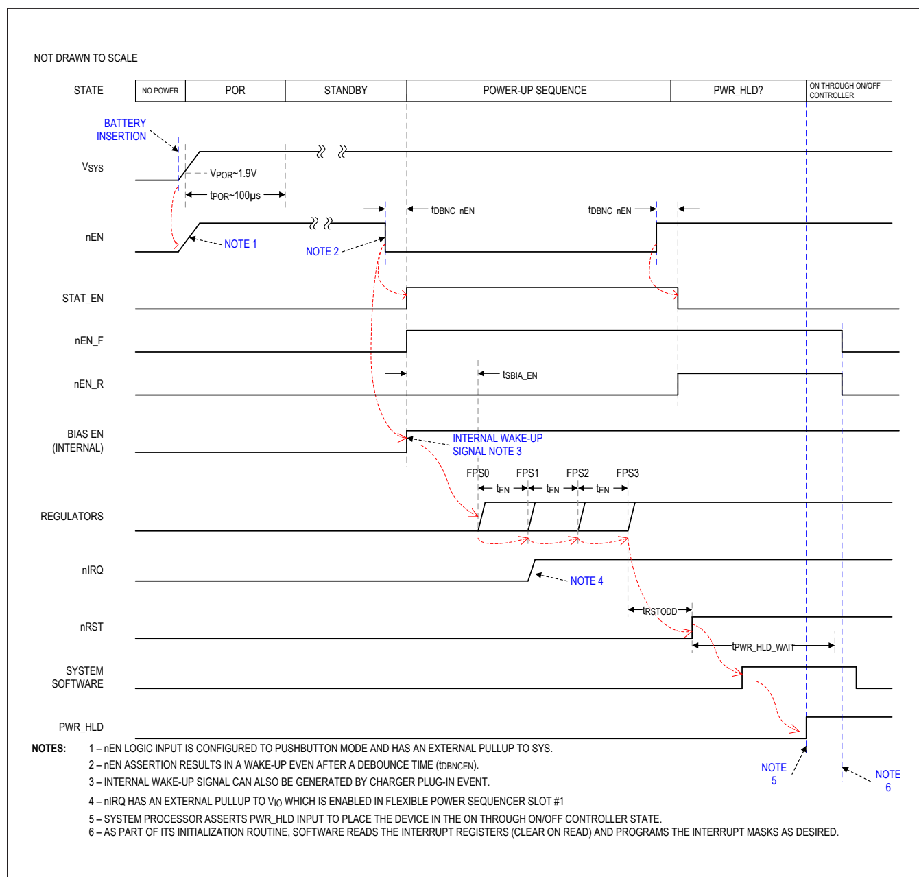
Figure 7. Startup Timing Diagram Due to nEN
