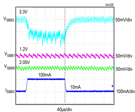
SBB2 LOAD TRANSIENT
