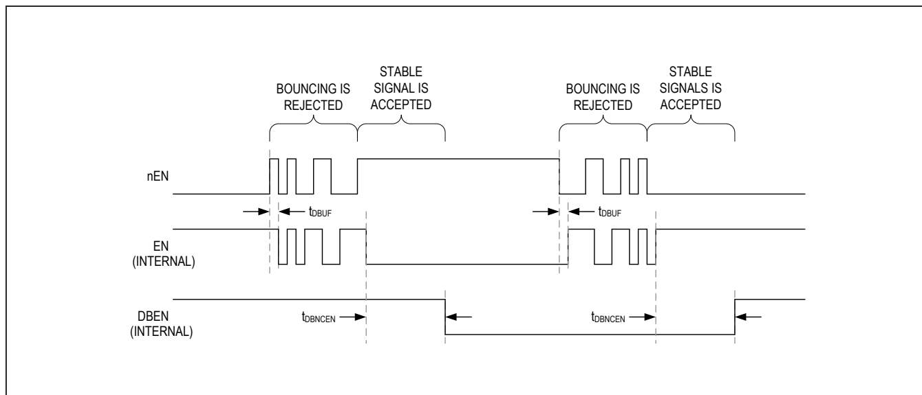
Figure 9. Debounced Inputs
