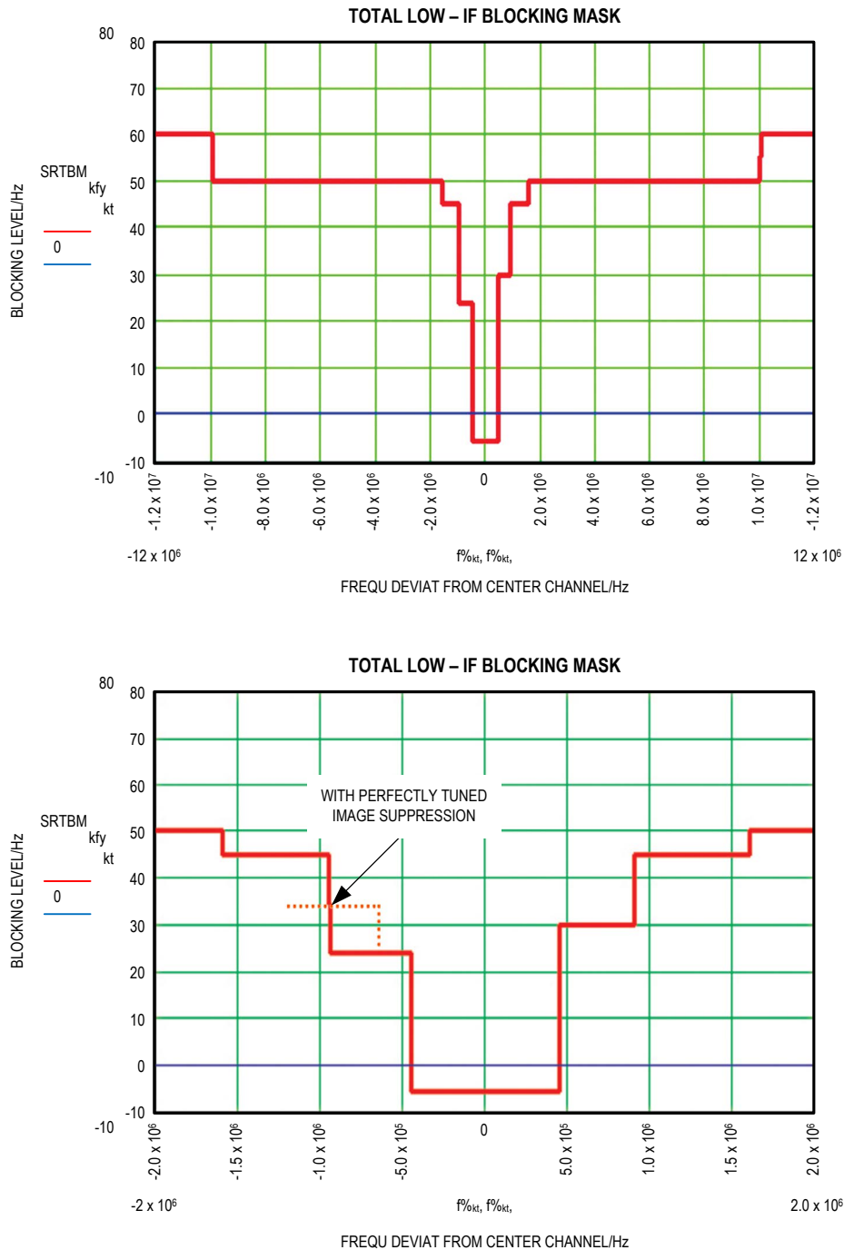
Figure 1. Blocking Mask of the Receiver at Double Wideband Operation. (Dotted line with perfect image rejection tuning. The image position may be swapped to upper side too. SRQ fulfilled with: Useful signal applied 3dB above the measured sensitivity limit. However, not below maximum of S0_X + 3\text{dB} . Blocking signal unmodulated CW.)
