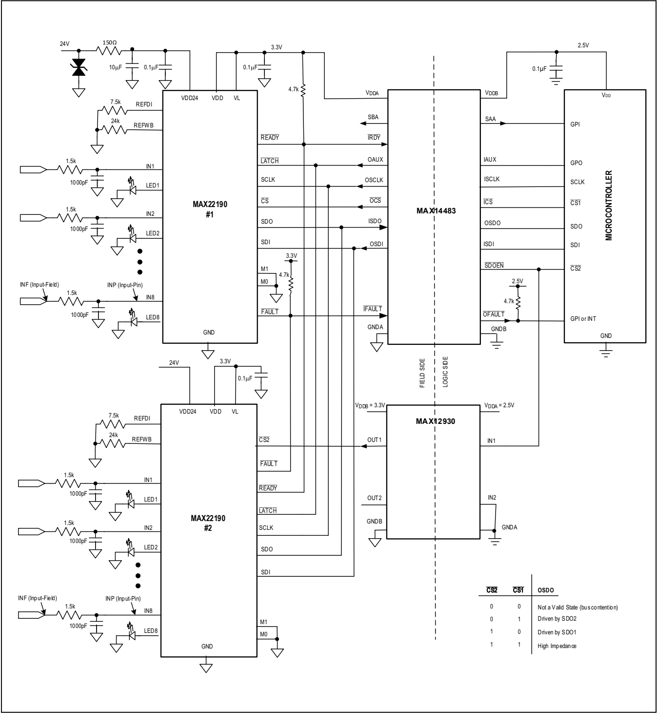
Figure 10. 16 Input, Independent Slave SPI (Separate CS for Each SPI Slave)
