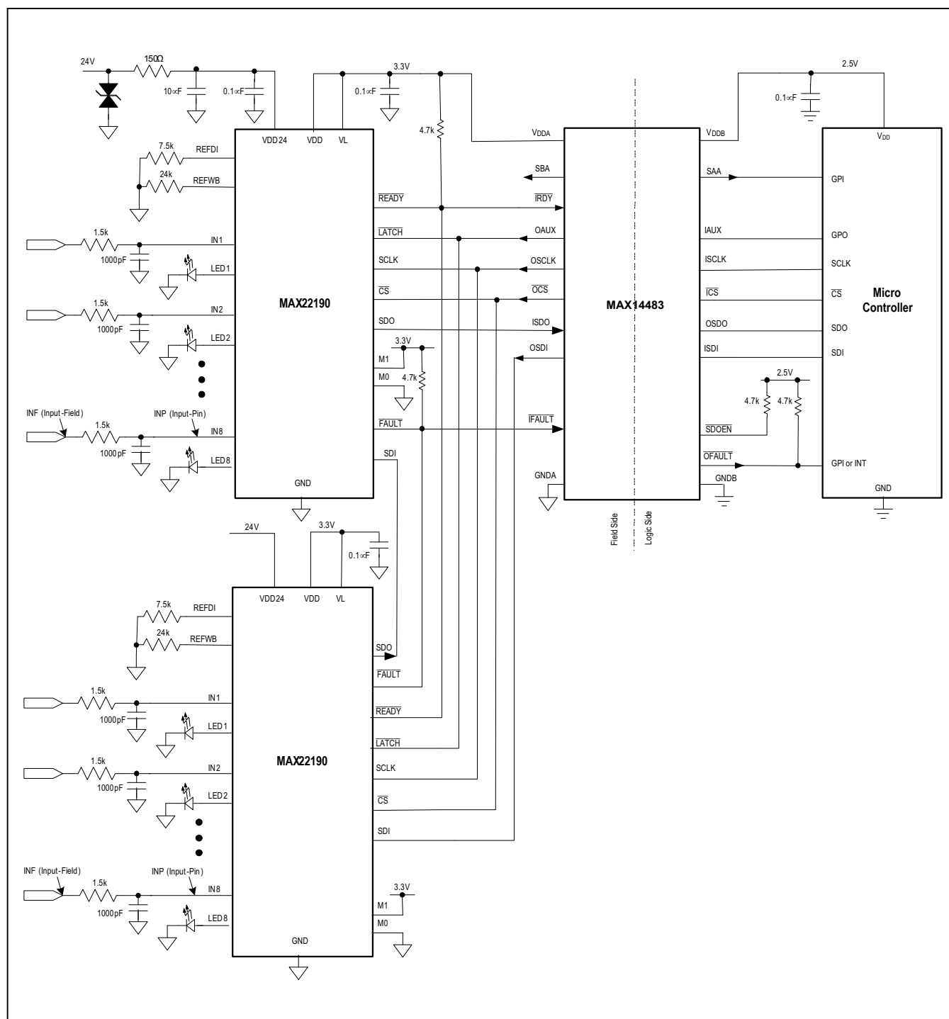
Figure 9. 16 Input, SPI Daisy Chain
