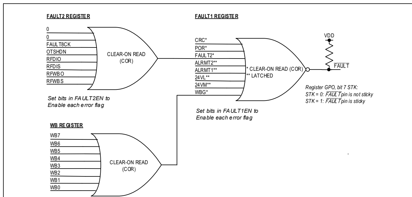
Figure 8. \overline{FAULT} Output Sources
