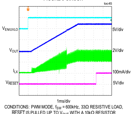
MAX17672C, 5V OUTPUT SOFT-START FROM EN/UVLO FIGURE 8 CIRCUIT
