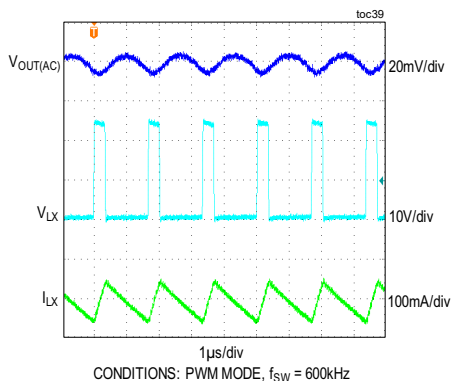
MAX17671F, 5V OUTPUT STEADY STATE AT 0mA LOAD FIGURE 6 CIRCUIT
