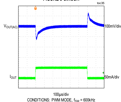
MAX17672C, 5V OUTPUT LOAD TRANSIENT BETWEEN 0mA AND 50mA FIGURE 8 CIRCUIT
