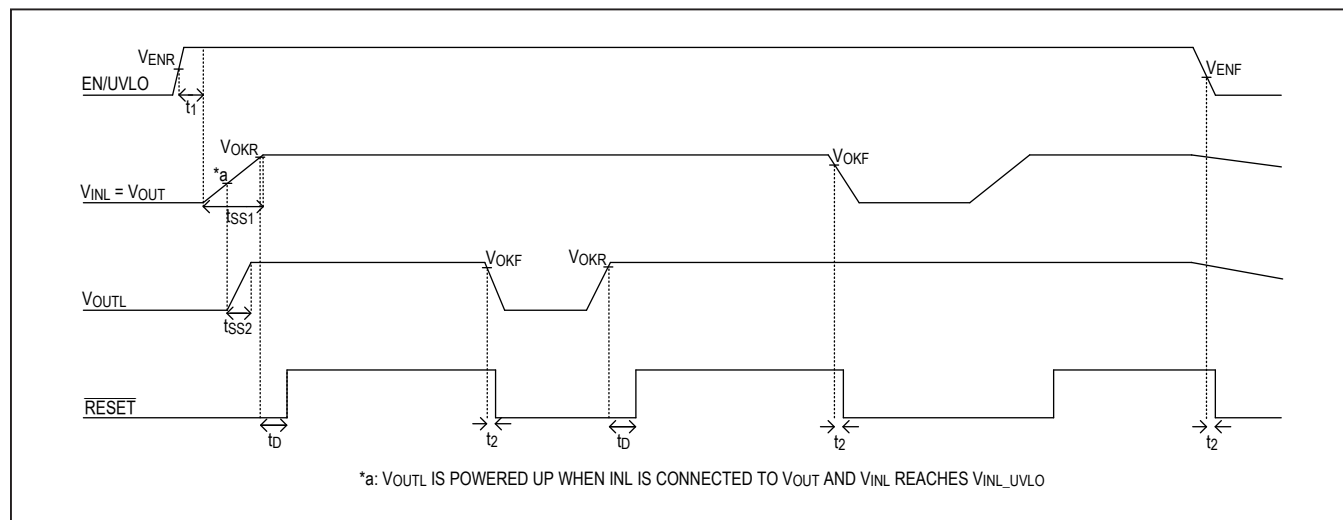
Figure 1. \overline{\text{RESET}} Output Logic Diagram when INL is Connected to the Step-Down Converter Output
