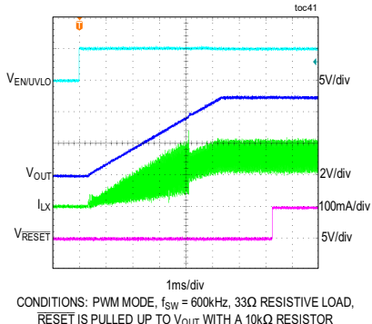
MAX17671F, 5V OUTPUT SOFT-START FROM EN/UVLO FIGURE 6 CIRCUIT
