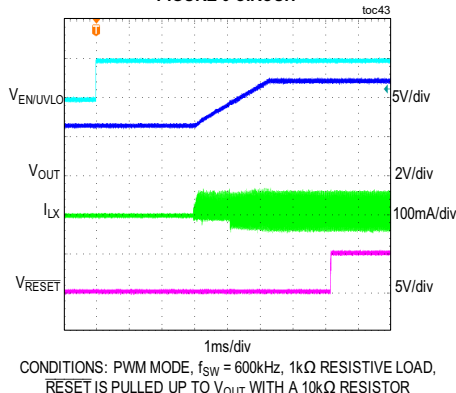
MAX17671F, 5V OUTPUT SOFT-START WITH PREBIAS VOLTAGE OF 2.5V FIGURE 6 CIRCUIT
