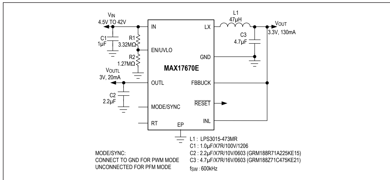
Figure 7. Fixed 3.3V Step-Down Converter Output at 600kHz Switching Frequency and 3.0V Linear Regulator Output
