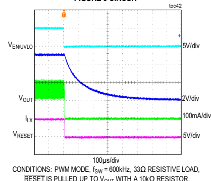
MAX17671F, 5V OUTPUT SHUTDOWN FROM EN/UVLO FIGURE 6 CIRCUIT
