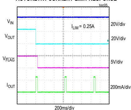
AUTORETRY CURRENT-LIMIT RESPONSE
