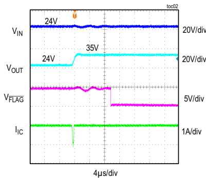
REVERSE-BLOCKING RESPONSE
