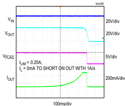
CURRENT-LIMIT RESPONSE
