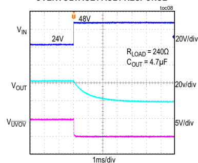
OVERVOLTAGE FAULT RESPONSE
