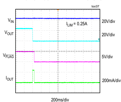
LATCH-OFF CURRENT-LIMIT RESPONSE
