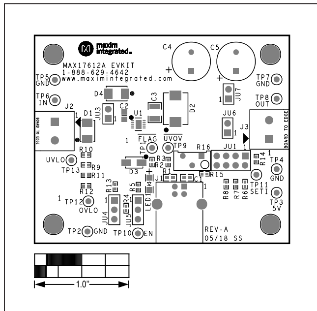
MAX17612A EV Kit PCB Layout—Top Silkscreen
