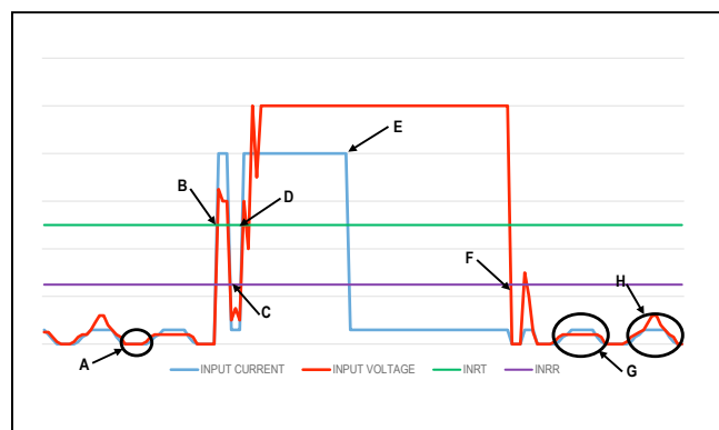
Figure 4. Voltage Triggerred Inrush Mode
