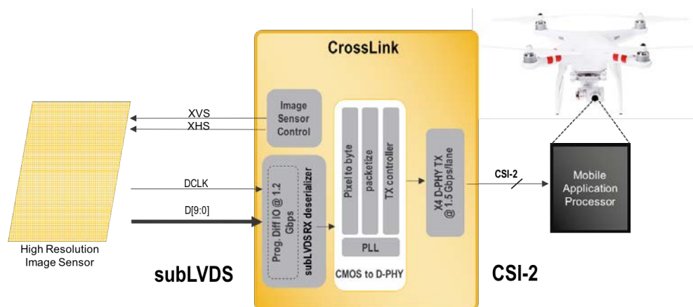
Camera Interface Conversion Bridging
