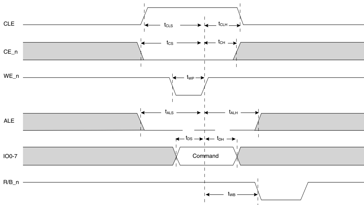
Figure 44. Command Cycle
