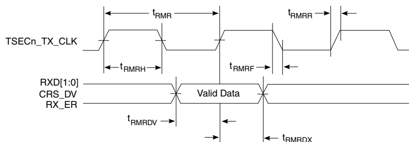
Figure 24. RMI receive AC timing diagram
