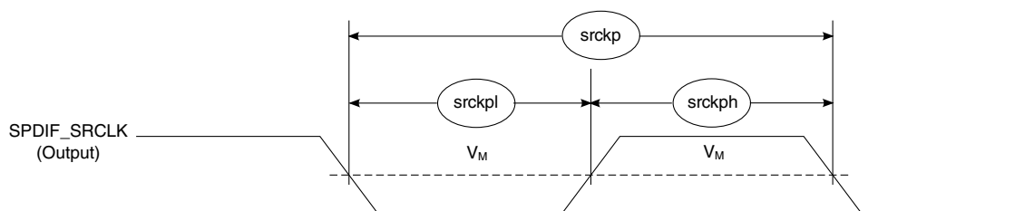
Figure 50. SPDIF_SRCLK timing
