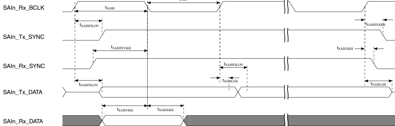
Figure 49. SAI timing — slave modes
