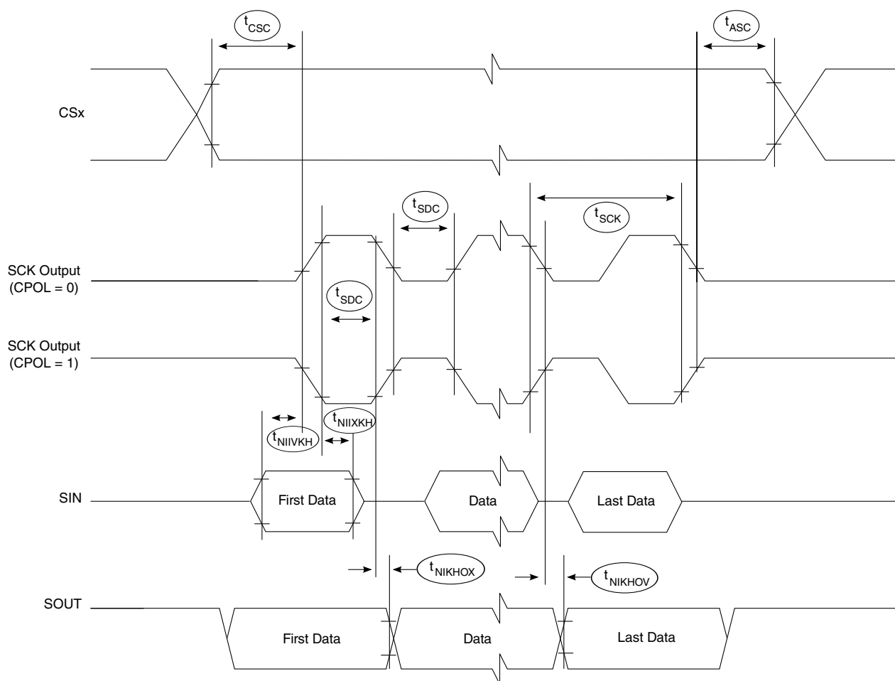
Figure 52. SPI timing master, \text{CPHA} = 0
