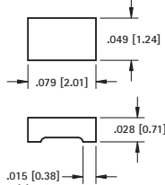
Mounting Detail
