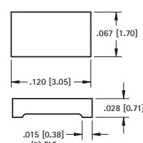
Mounting Detail
