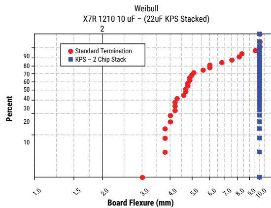
Board Flex vs. Termination Type
