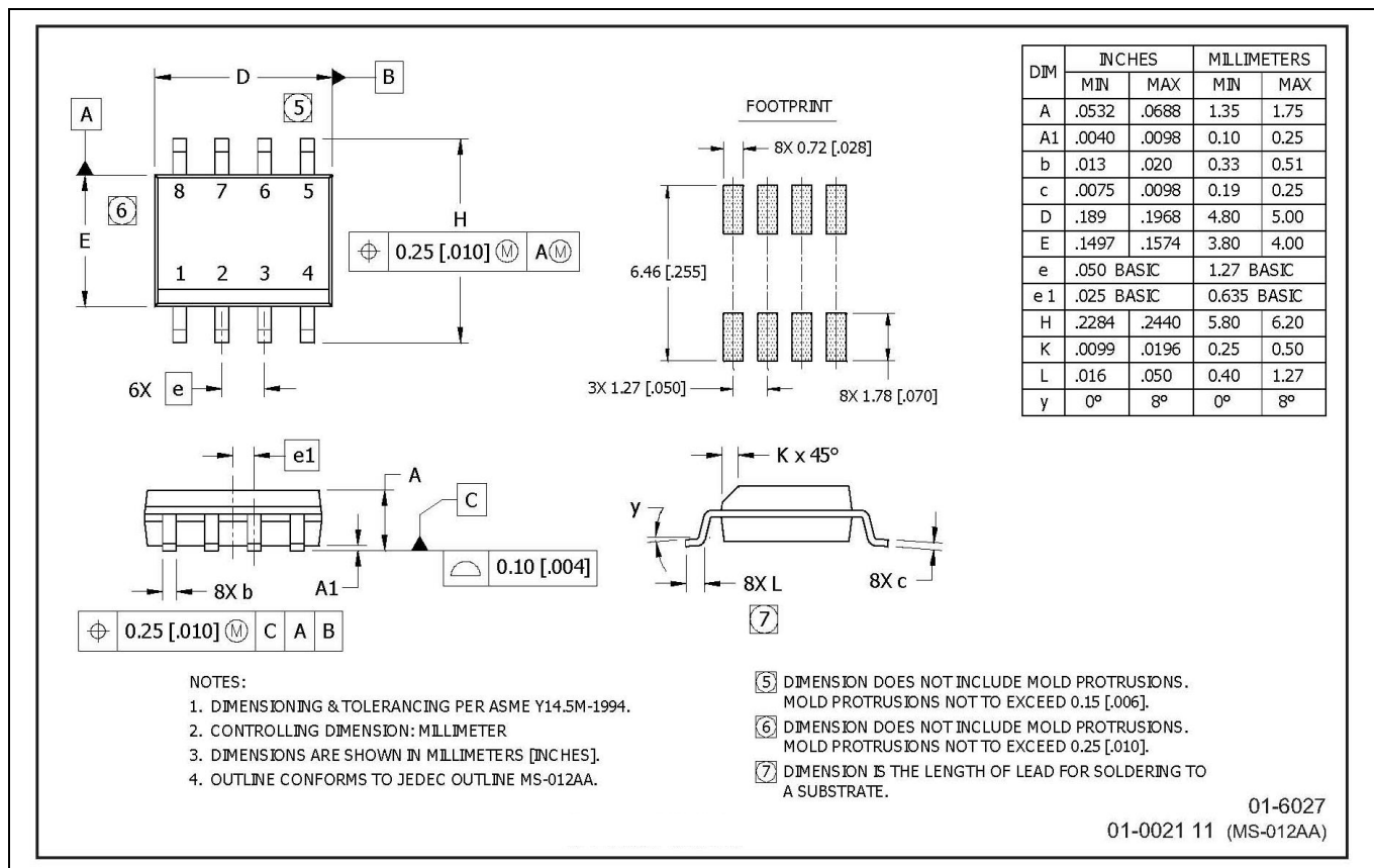
Figure 2 Package outline dimensions
