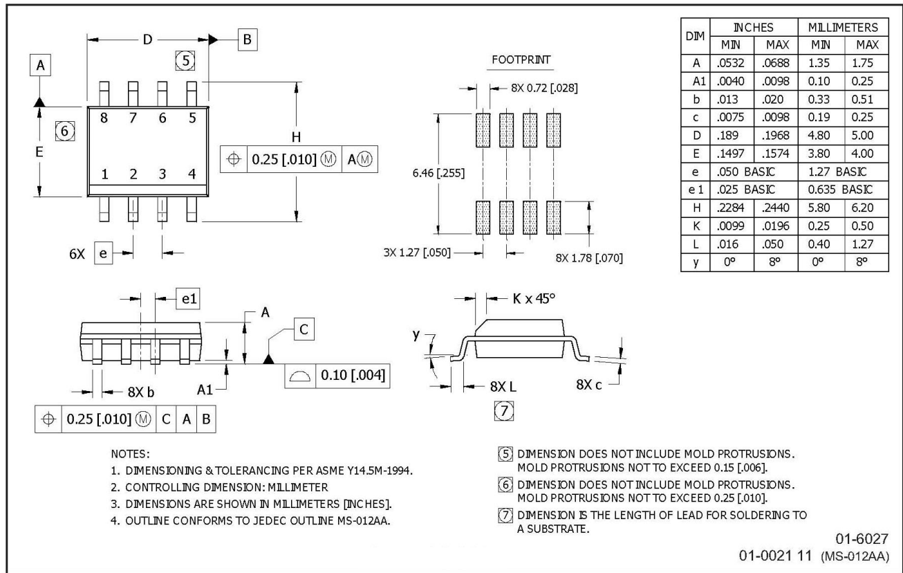
Figure 16 Package outline
