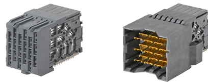
Impel Plus 3-Pair, 2.35mm-Pitch Right-Angle Orthogonal Direct Connector System
