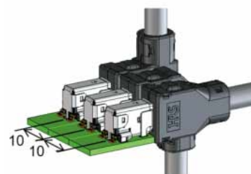
Parallel mounting on a narrow pitch (P=10mm)
