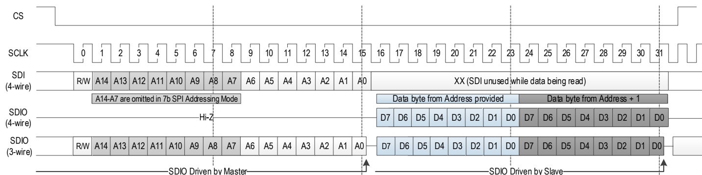
Figure 20. SPI Sequencing
