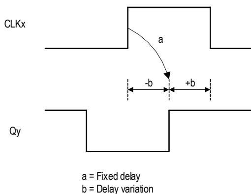
Figure 32. Input-Output Delay
