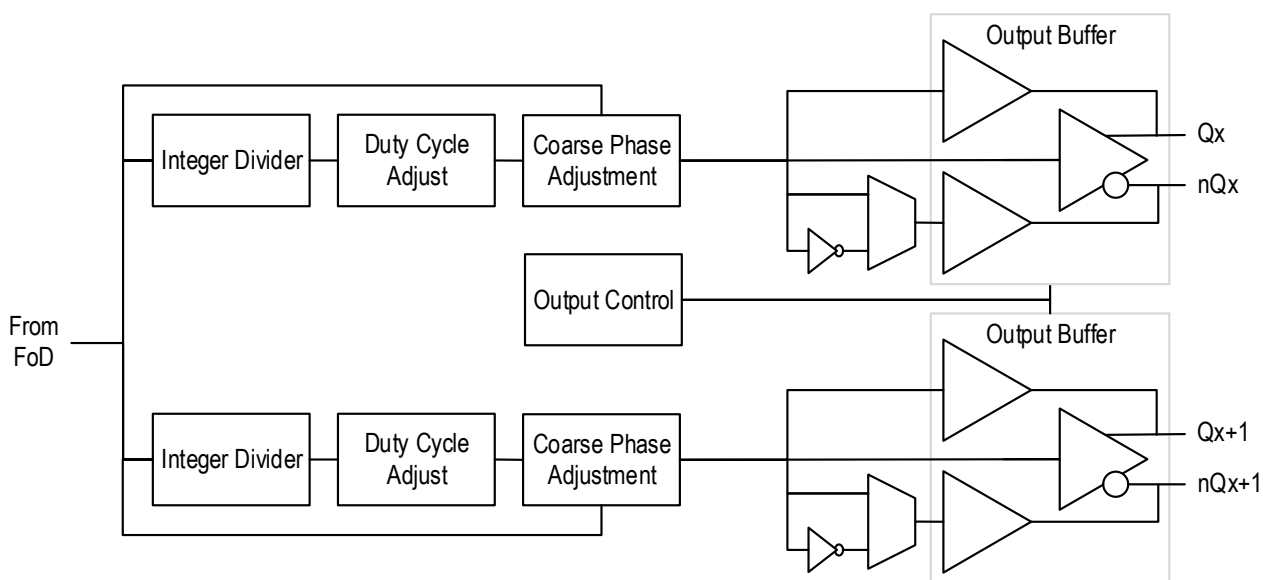
Figure 14. Dual Output Stage
