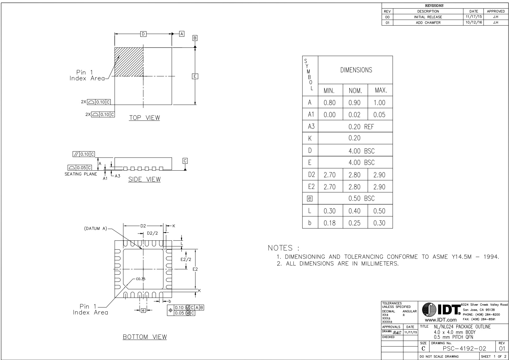
Figure 23. NLG24P2, 4 × 4 mm 24-VFQFPN Package Drawings – page 1
