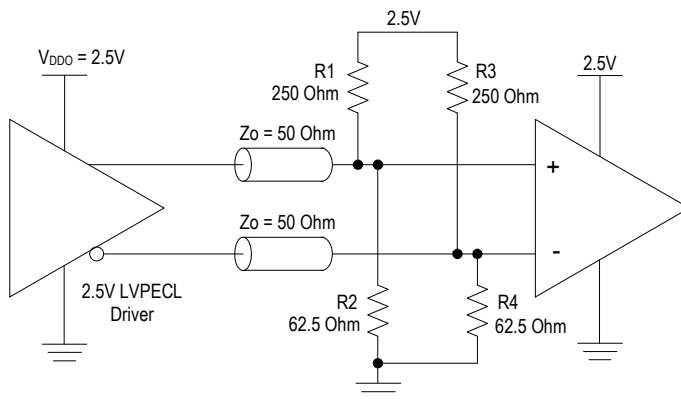
Figure 17. 2.5V LVPECL Output Termination (3)
