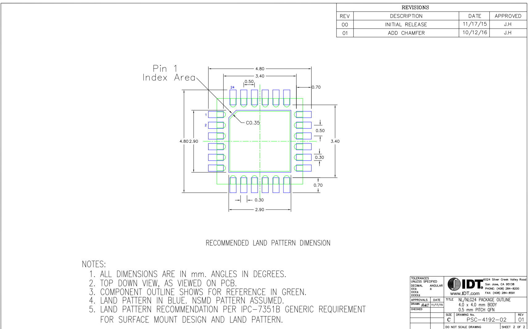
Figure 24. NLG24P2, 4 x 4 mm 24-VQFPN Package Drawings – page 2
