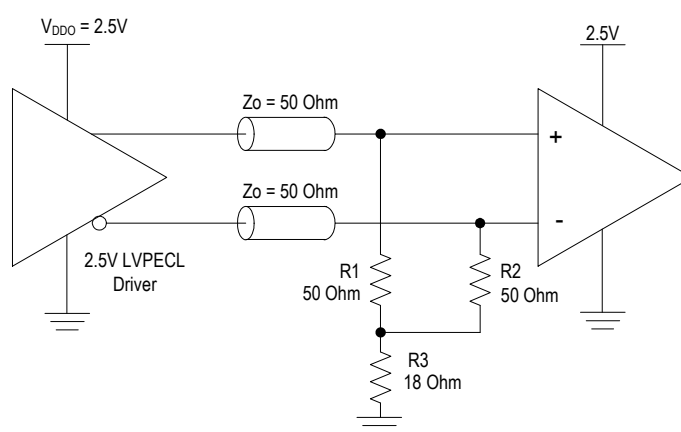
Figure 19. 2.5V LVPECL Driver Termination (3)
