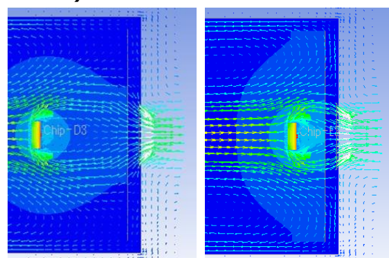
Figure 22 Airflow at the back of the MOSFET
