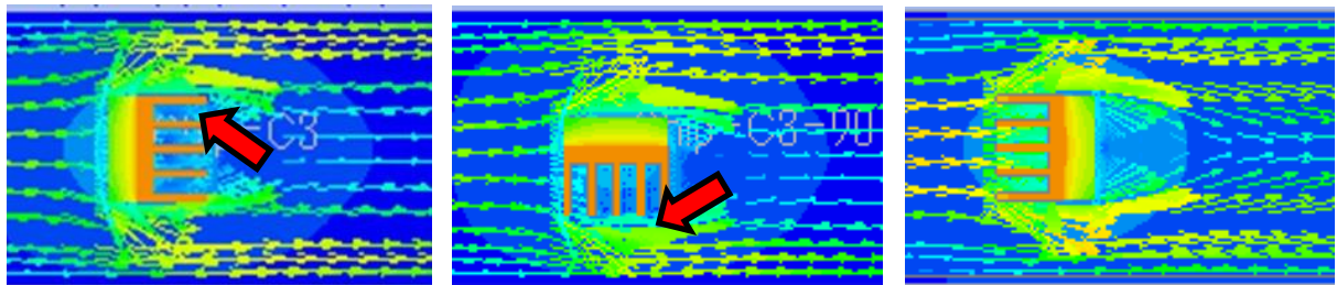
Figure 28 Air velocity distribution around the heatsink
