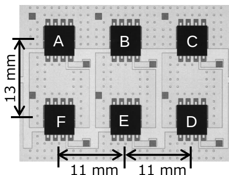
Device arrangement
