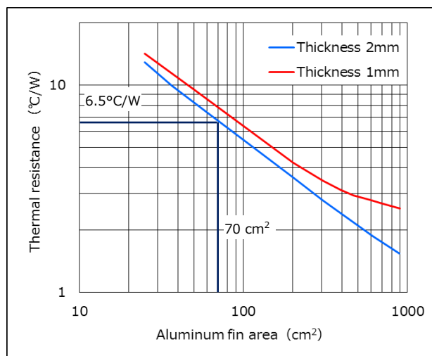
Figure 2 - Heatsink surface area vs. thermal resistance (example)
