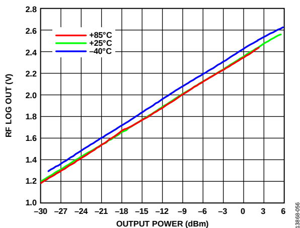
Figure 57. Log RF Detector vs. Output Power over Temperature, RF = 4 GHz
