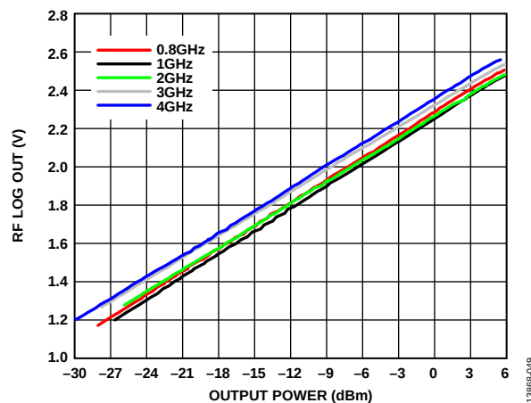
Figure 50. Log RF Detector vs. Output Power over RF Frequency
