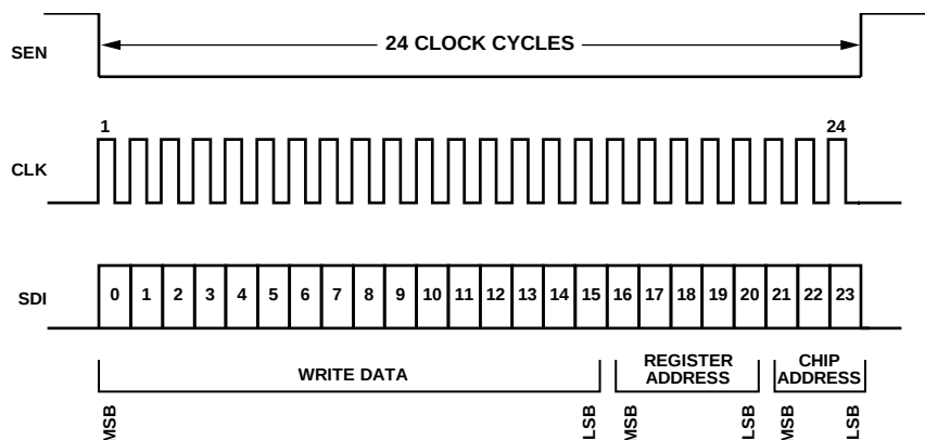
Figure 61. Timing Diagram, SPI Register Write
