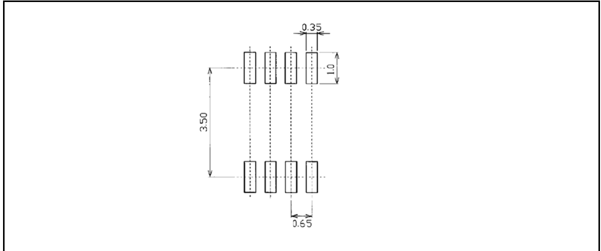
Figure 4-2 Recommended Footprint (Reference)
