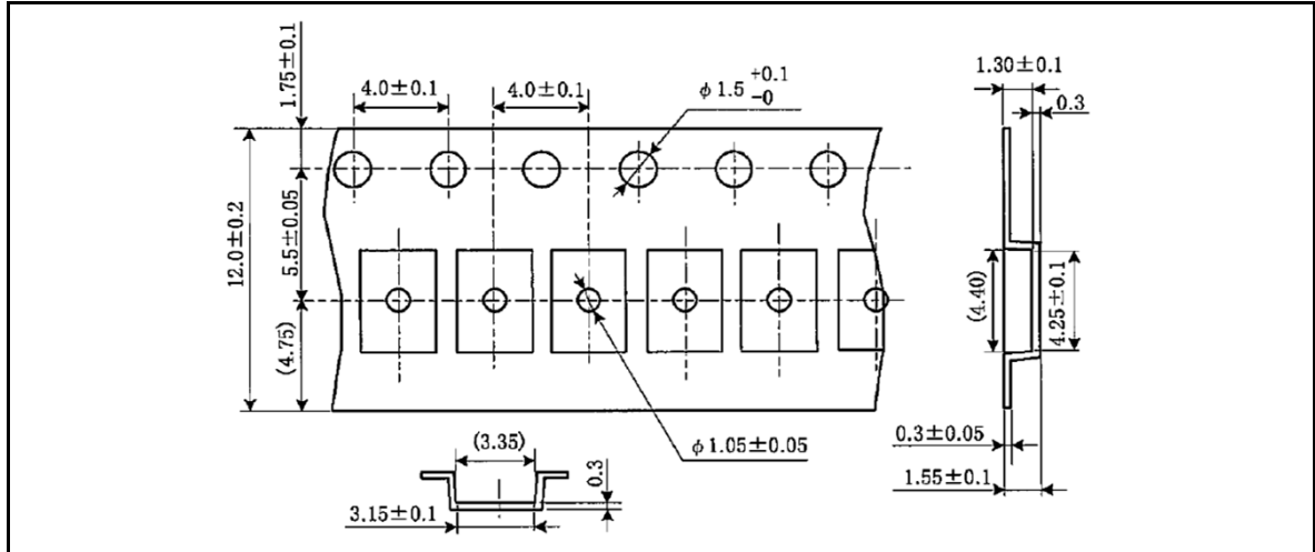
Figure 5-1 Emboss Tape Dimensions
