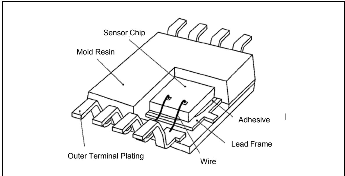
Figure 4-4 Internal Structure
