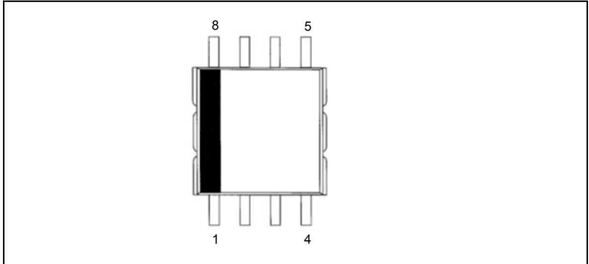
Figure 2-1 Pin Configuration
