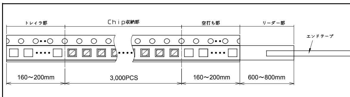
Figure 5-5 Taping Specification
