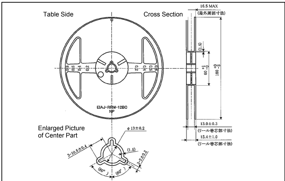
Figure 5-2 Reel Dimensions
