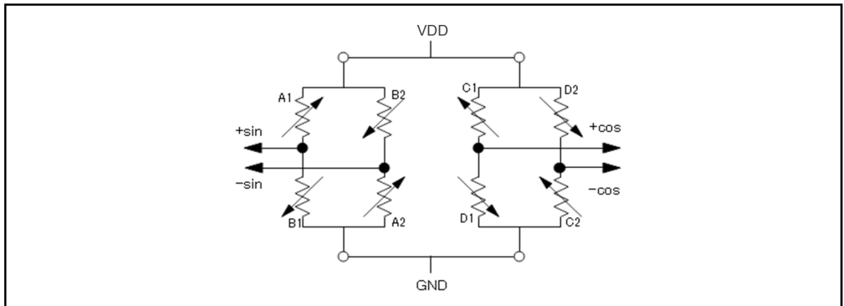
Figure 3-2 Equivalent Circuit
