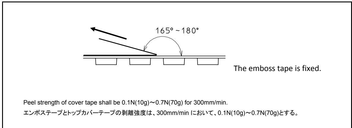
Figure 5-6 Peel Strength
