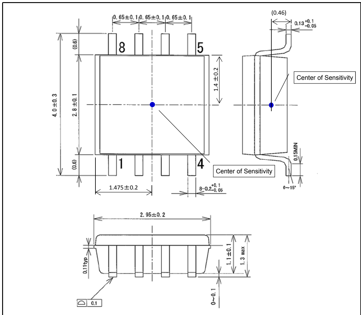
Figure 4-1 Package Outline (All dimensions in mm)
