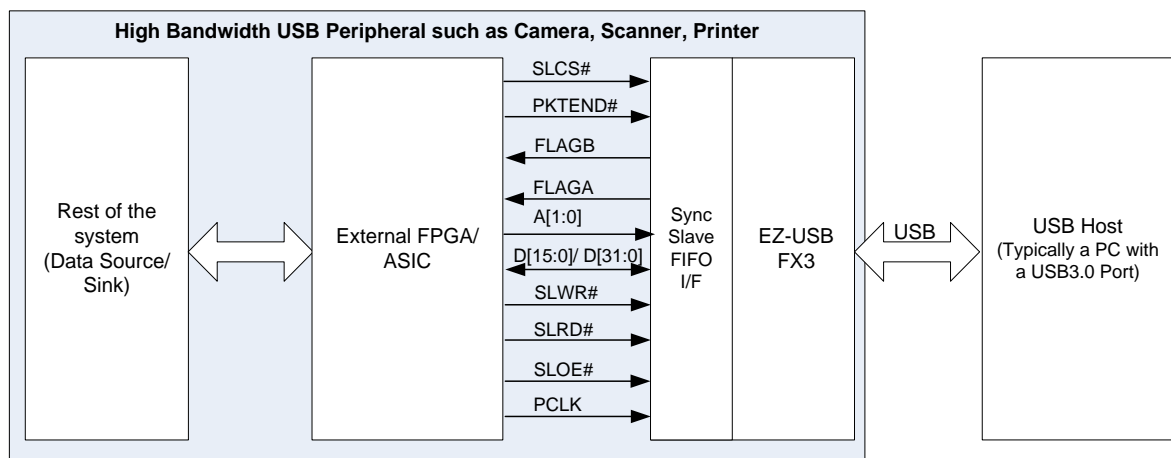
Figure 2. FPGA/ASIC Interfaced to FX3
