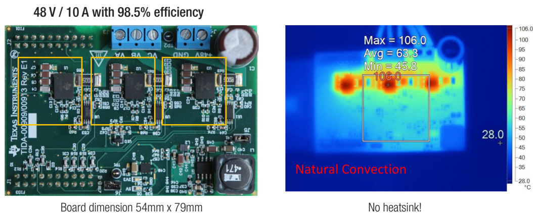
Figure 7. GaN inverter. 100kHz 3-stage design.
