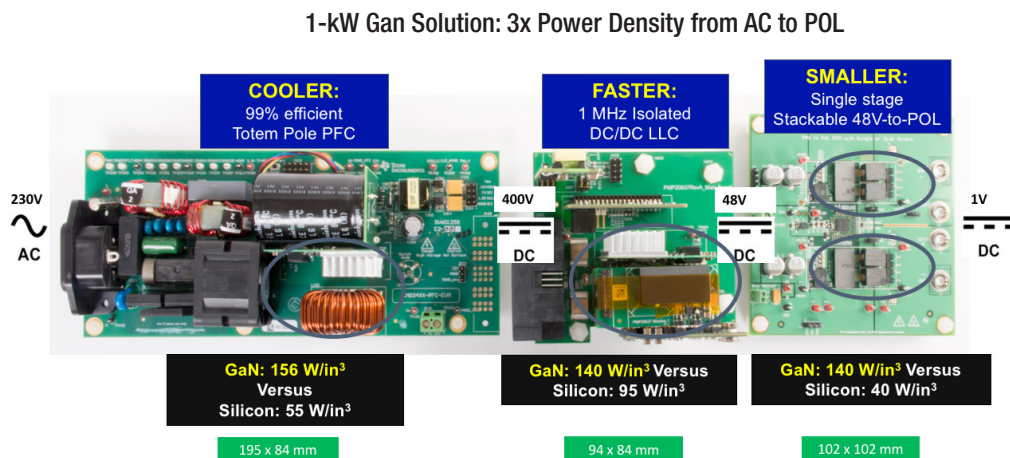
Figure 2. In all stages of the power supply, GaN solutions can reduce scale and increase efficiency.
