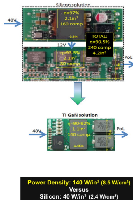
Figure 5. Two POL stages to a single stage.
