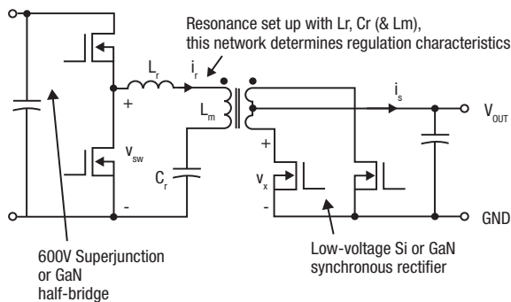
Figure 4. GaN LLC topology.
