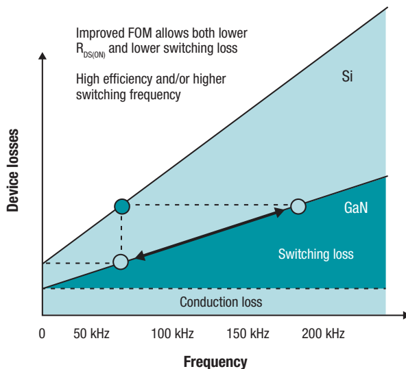
Figure 1. Comparison of device losses in GaN vs. Si.
