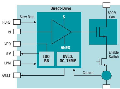
Figure 8. LMG3410: 600V/70 m \Omega 12A GaN Power Stage.
