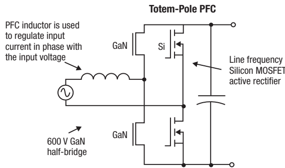
Figure 3. GaN PFC topology.
