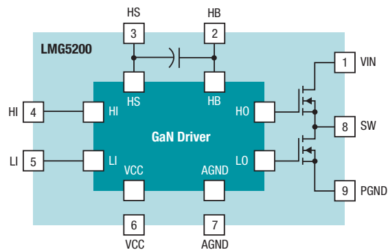
Figure 9. LMG5200: 80 V/10 A GaN Half-Bridge Power Stage.
