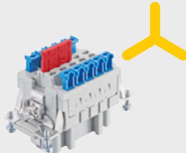
Star connection
