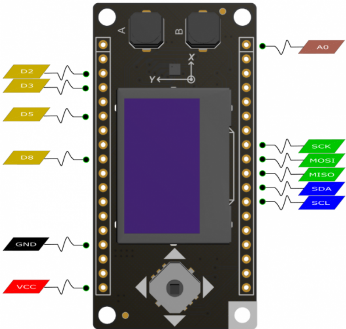
Fig2: FireBeetle Covers-OLED12864 Display Pinout
