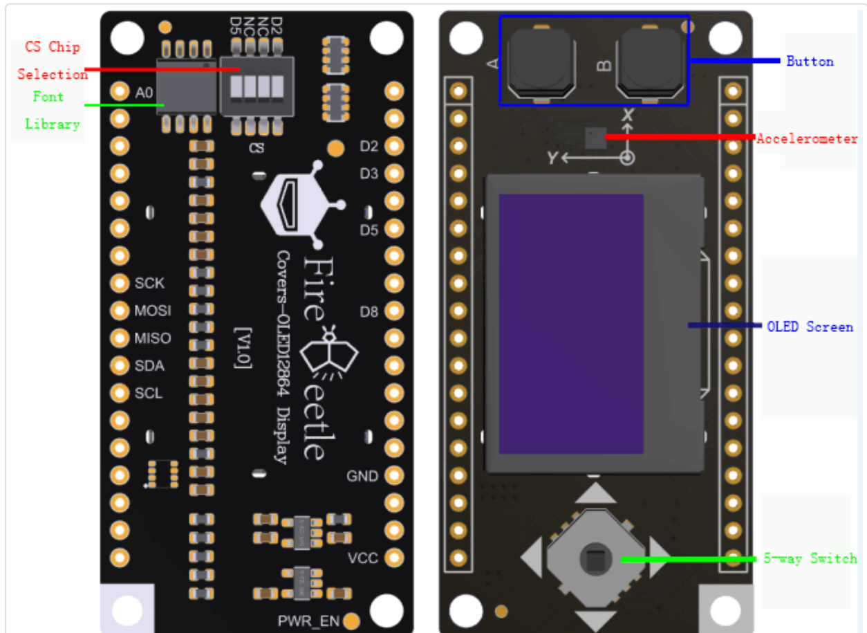
Fig1: FireBeetle Covers-OLED12864 Display Functional Module
