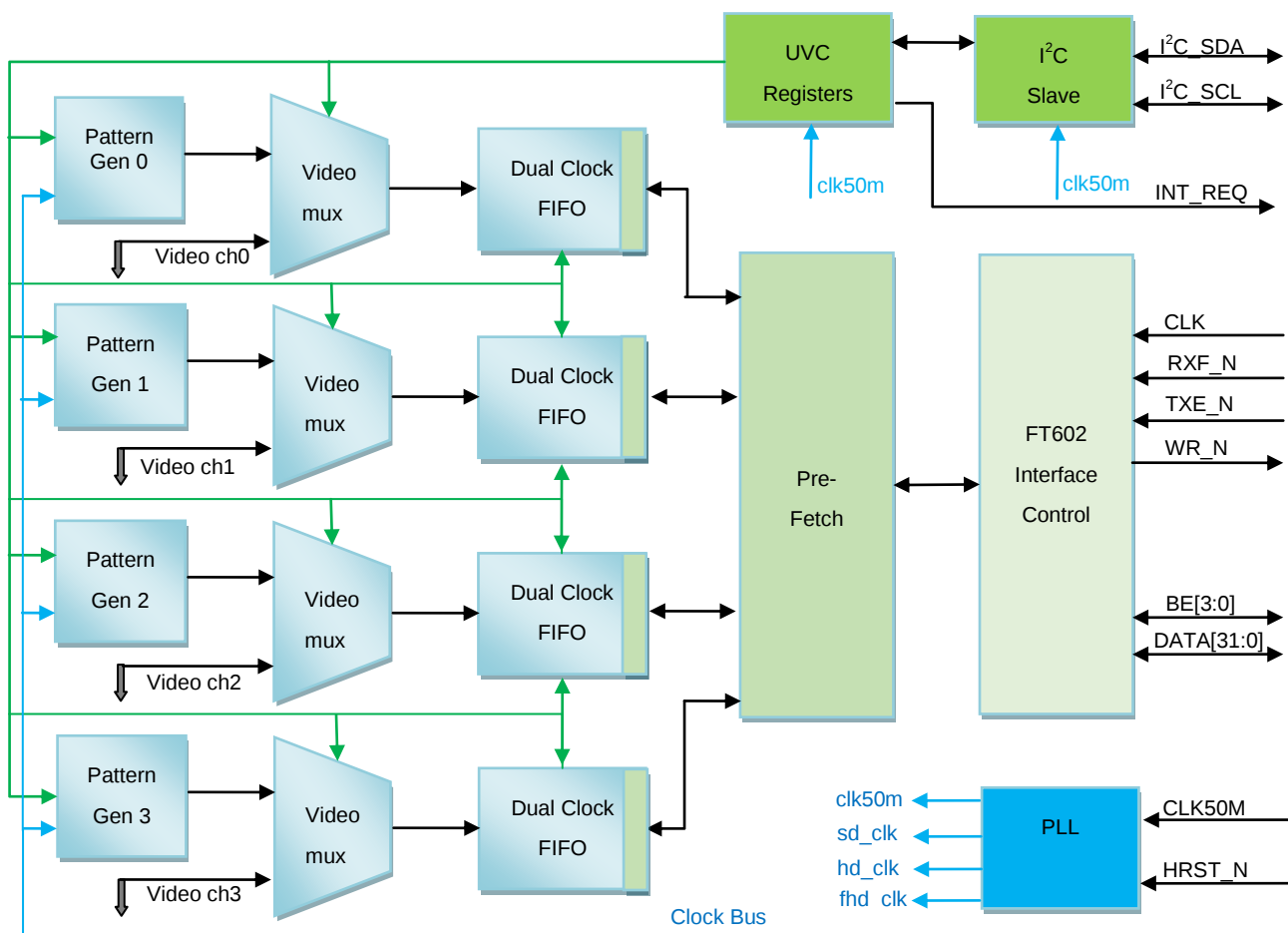
Figure 1 – Architecture
