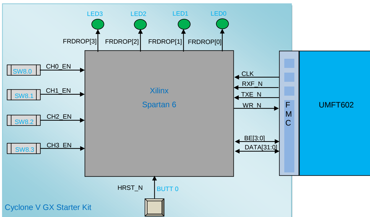
Figure 4 - Xilinx System Schematic
