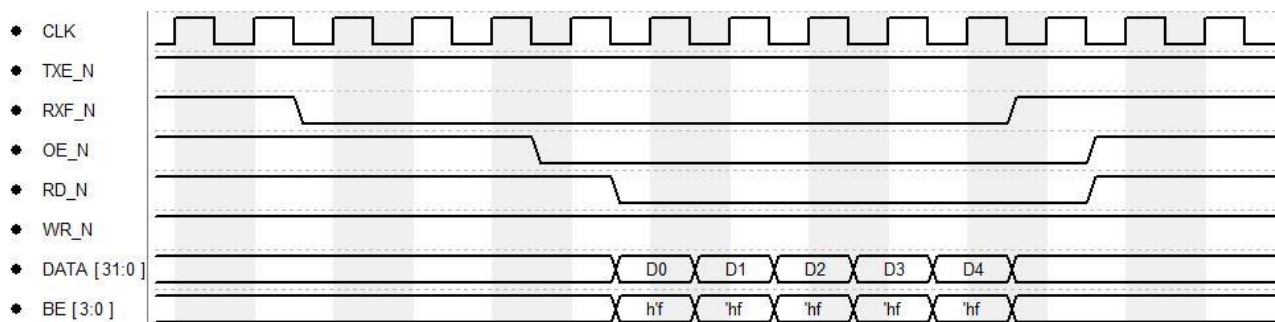
Figure 4.6 245 Synchronous FIFO mode bus master read cycle
