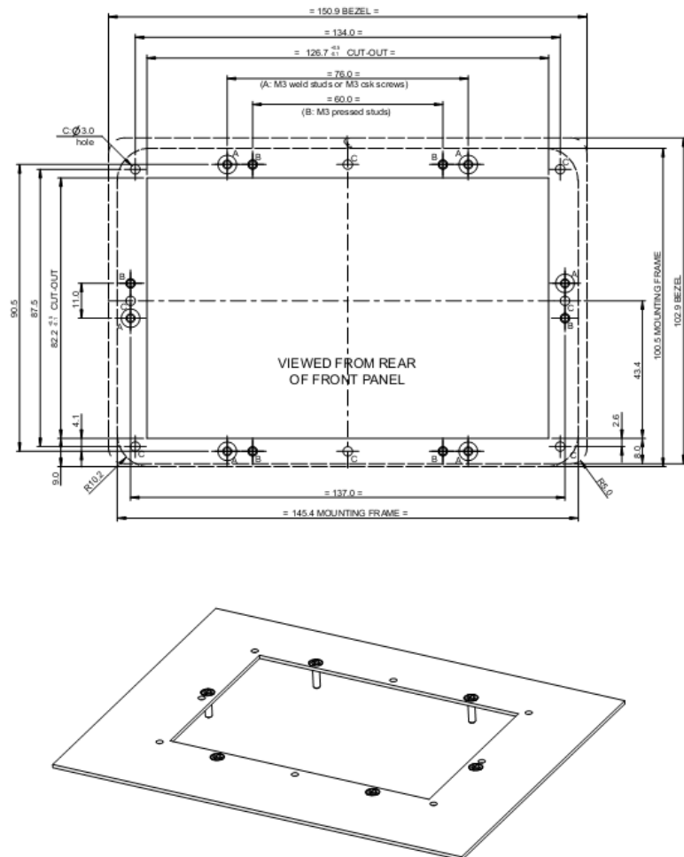
Figure 5-4 VM801P50A panel mount dimensions
