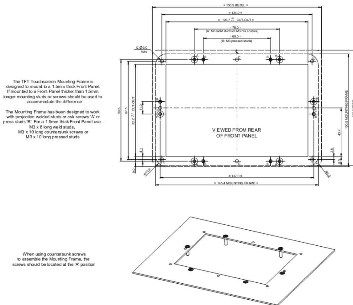
Figure 5-4 - VM801B 5.0" panel mount dimensions
