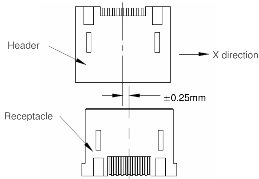
Fig.11 X-direction Misalignment
