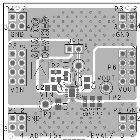
Figure 1. ADP7158CP-3.3EVALZ Printed Circuit Board (PCB) Layout
