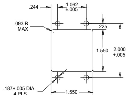
Mounting Layout
