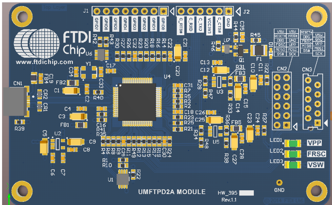
Figure 4.1 – UMFTPD2A Module Pin Out
