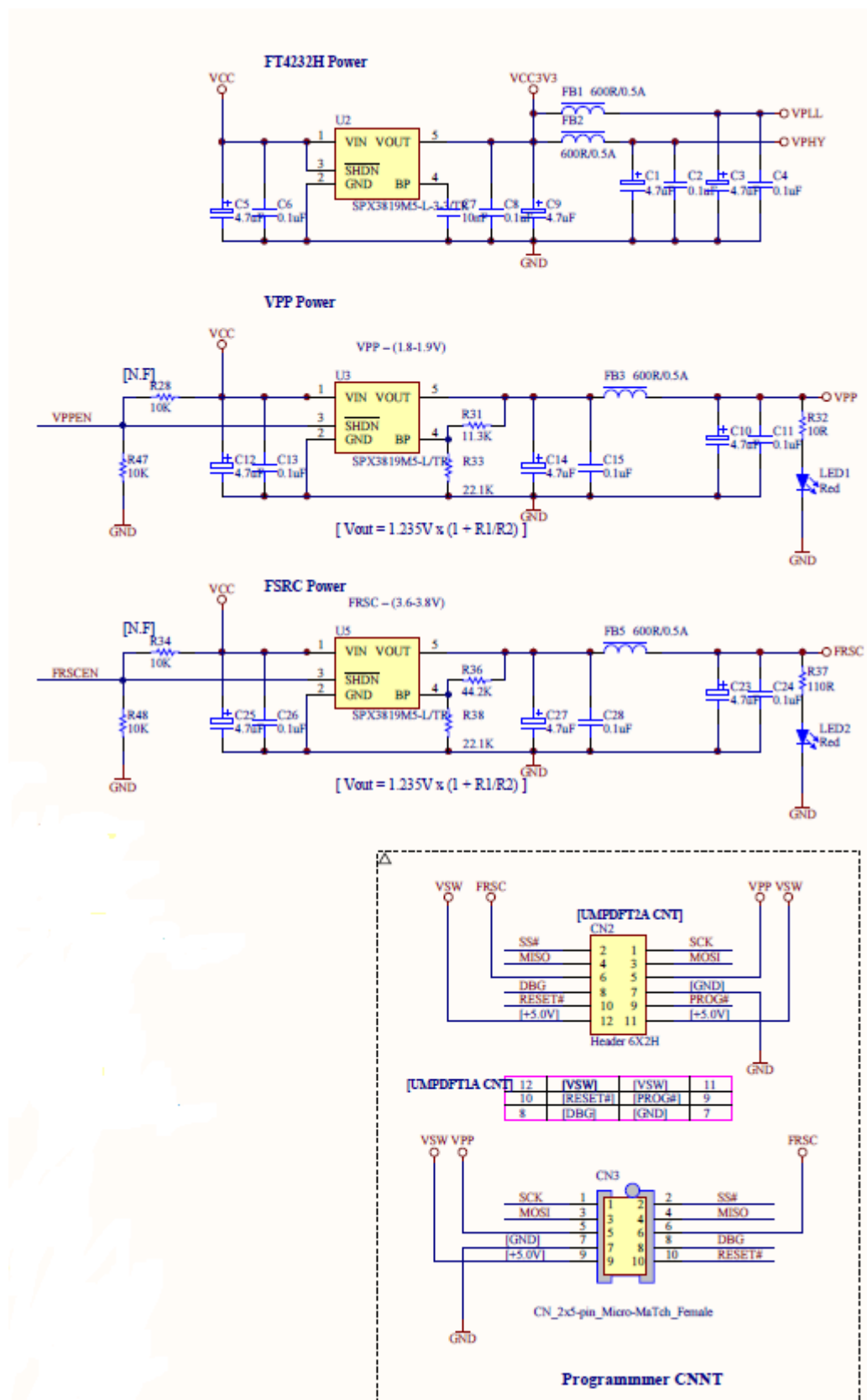
Figure 6.2 - Schematic part 1
