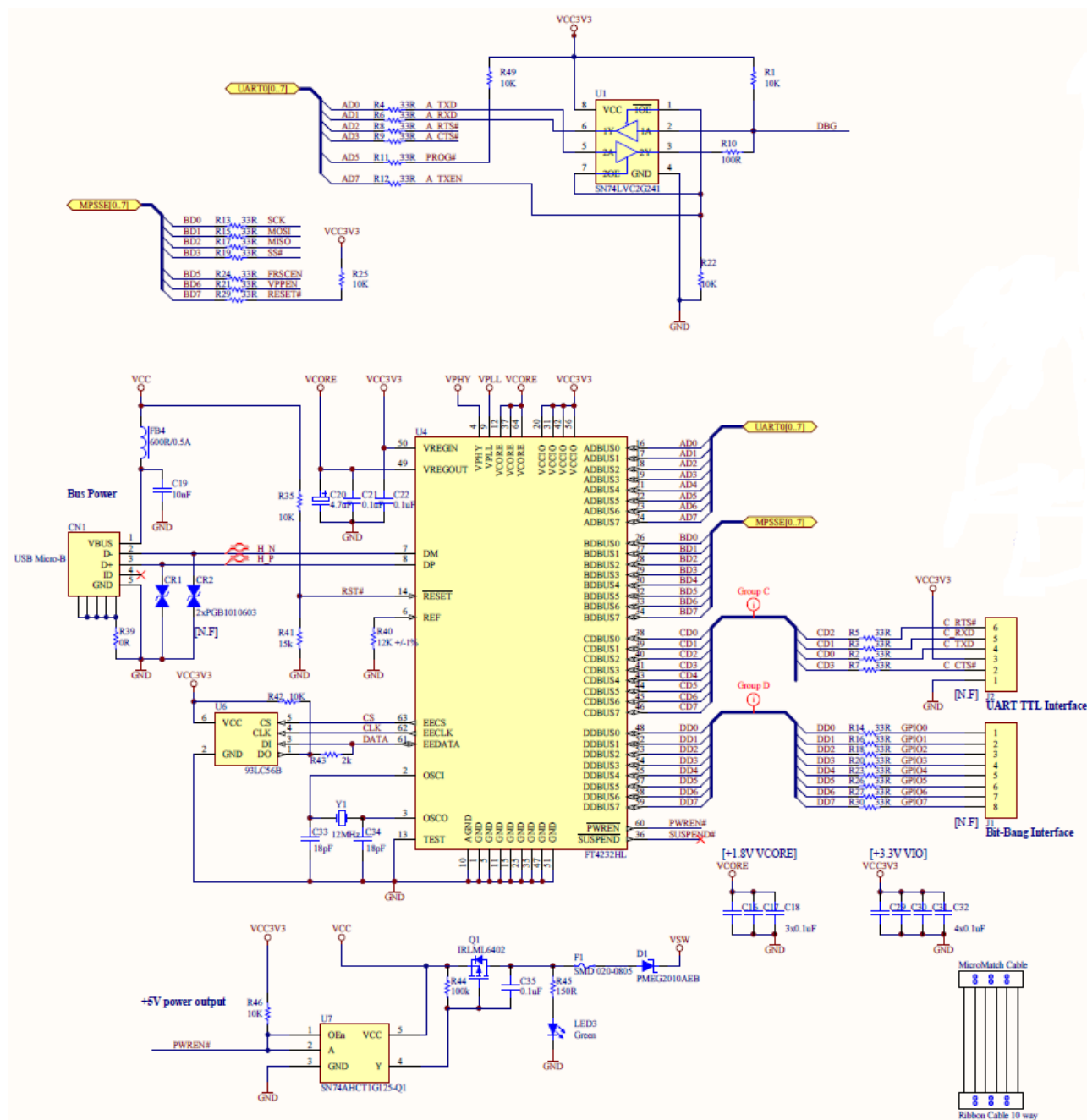
Figure 6.1 - Schematic part 1
