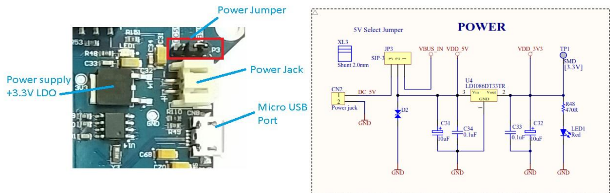
Figure 4-2– Power supply
