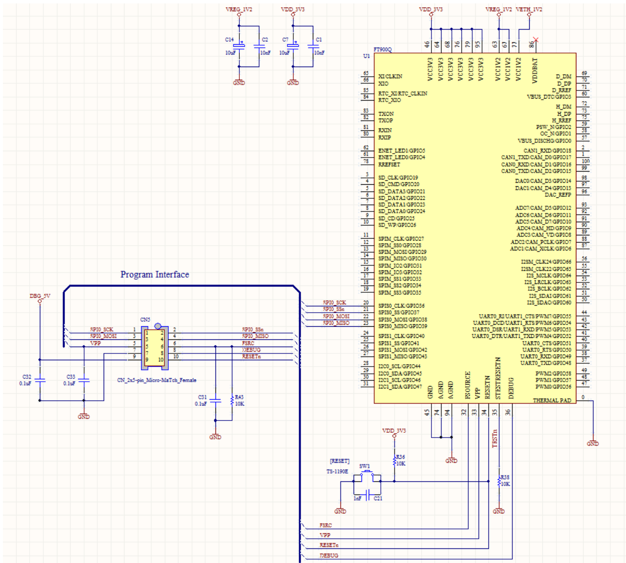
Figure 4-6 – Program Interface
