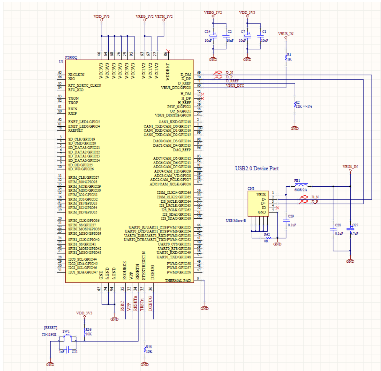
Figure 4-5– USB Connectors
