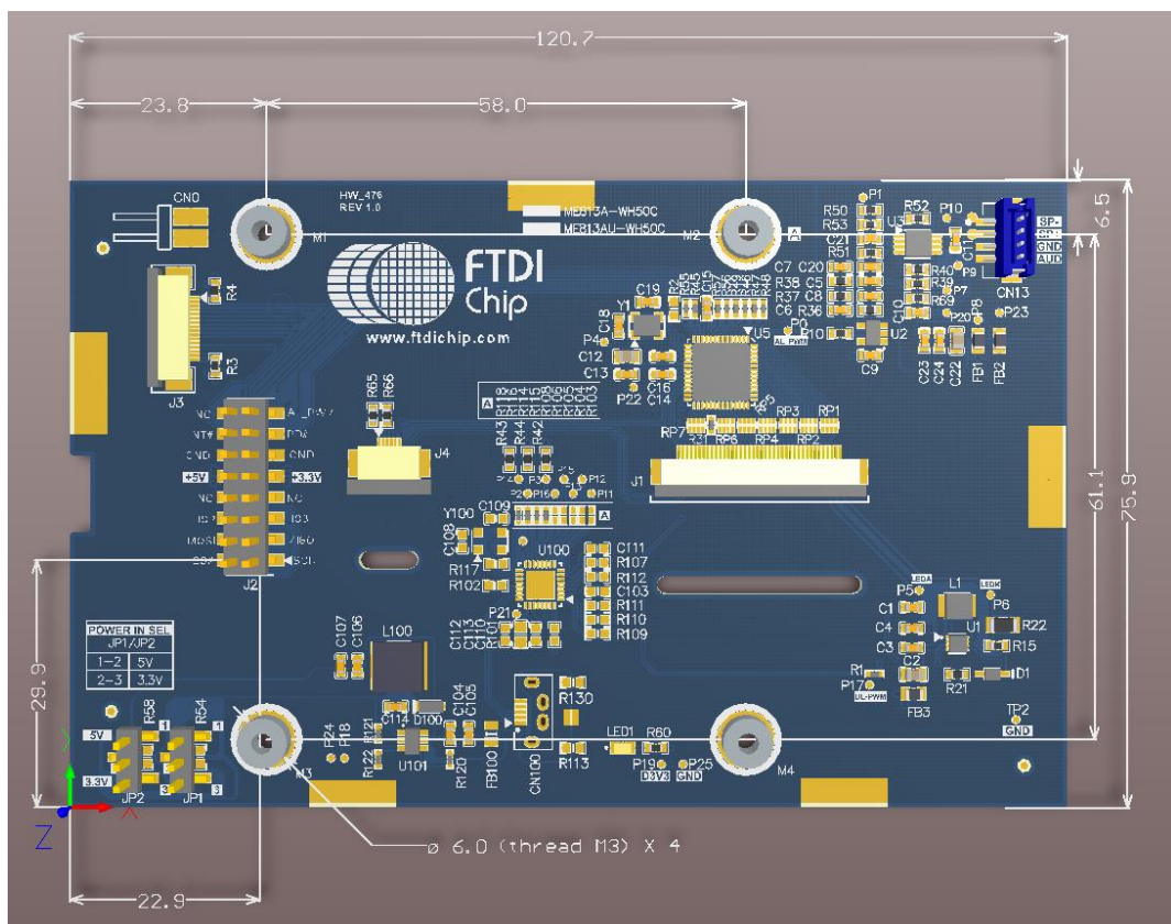
Figure 6-2 – PCB Dimensions
