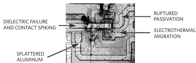
Figure 4. Integrated Circuits with Inadequate ESD Protection are Subject to Catastrophic Failures
