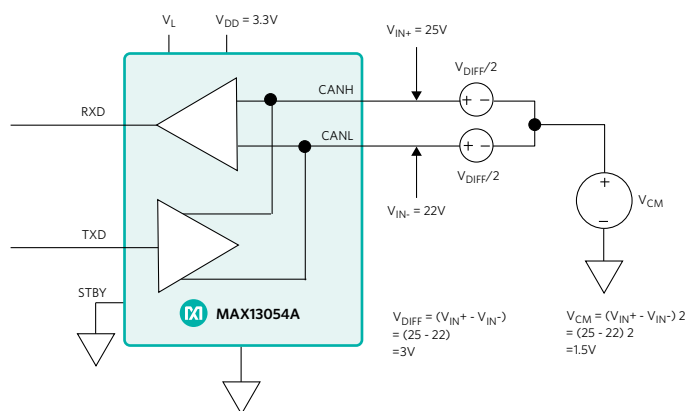
Figure 3. CAN Bus Common-Mode Model Showing the Differential Inputs ( V_{DIFF}/2 ) and the Common-Mode Input ( V_{CM} )
