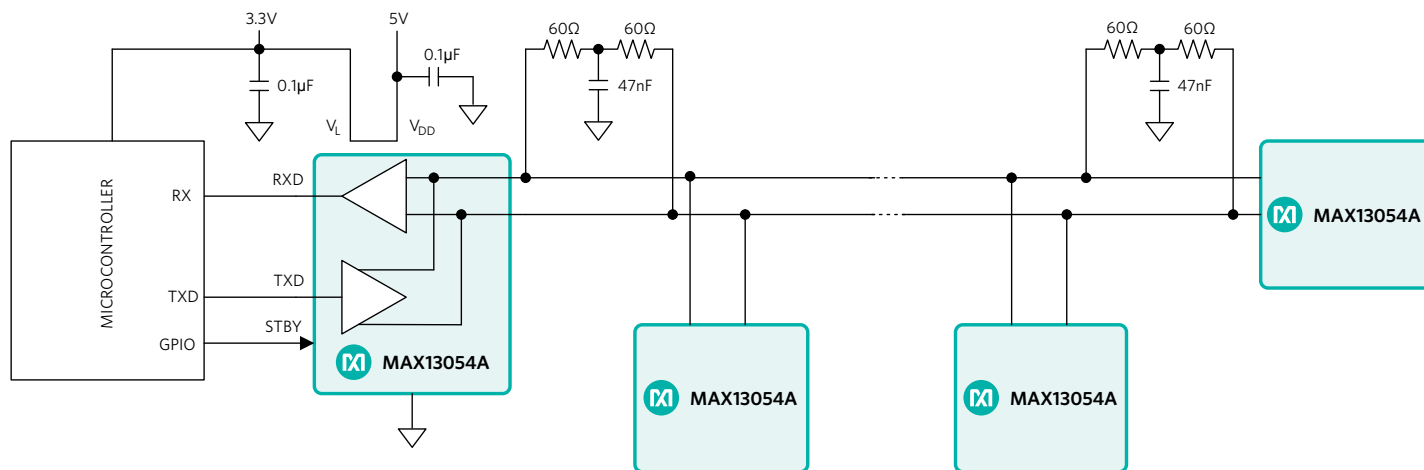
Figure 2. Multiple Receivers Connected to CAN Bus
