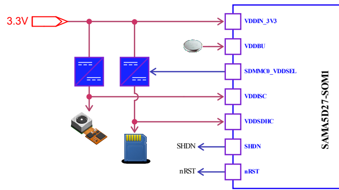
Figure 6-10. Power Configuration #4
