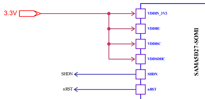
Figure 6-1. Power Configuration #1
