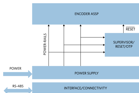
Figure 4. Encoder ASSP Power Rails Control
