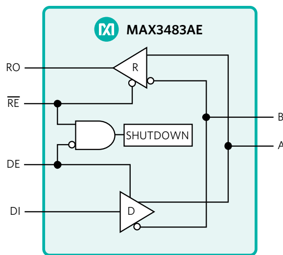
Figure 5. MAX3483AE Block Diagram
